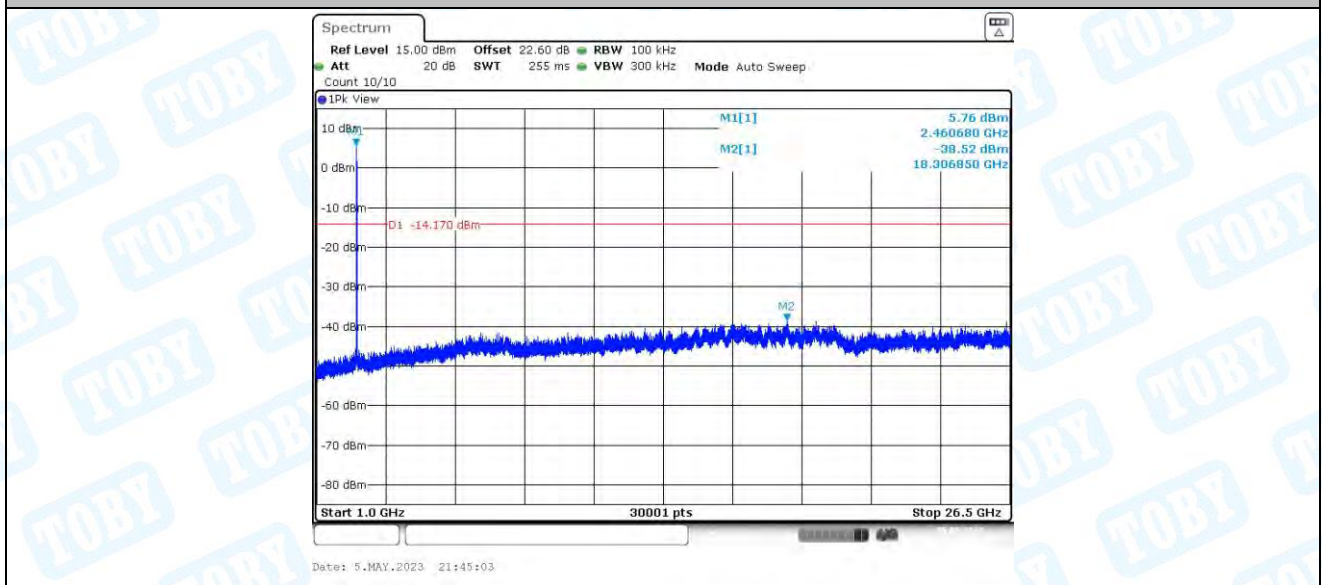
11G_Ant4_2462_0~Reference
