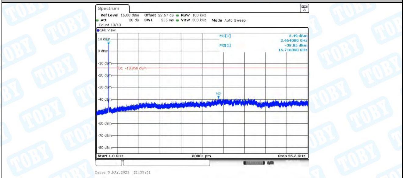
11G_Ant3_2462_0~Reference
