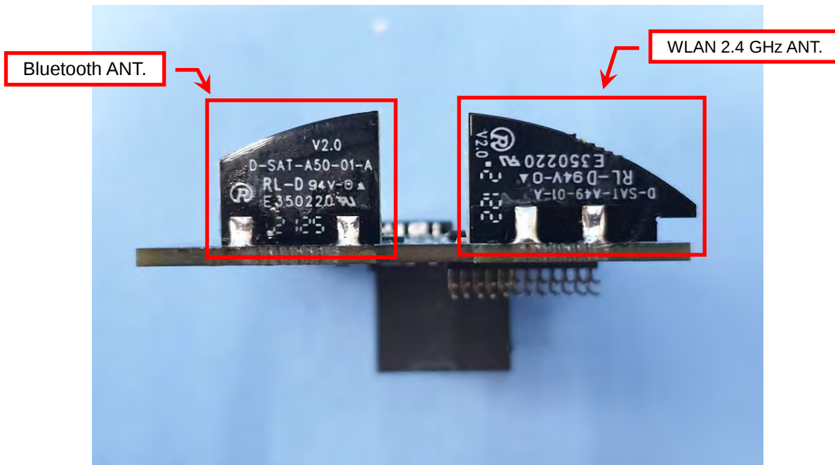
EUT Photo (28)
