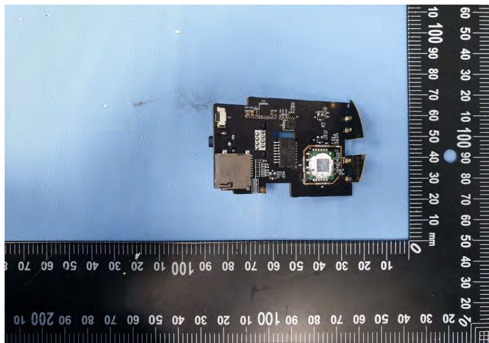
EUT Photo (26)
