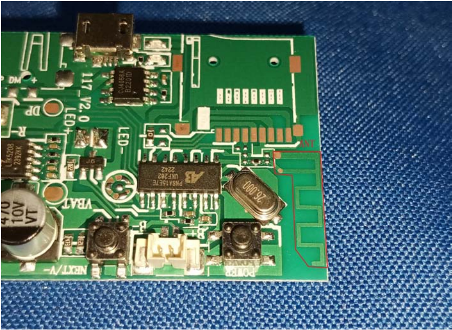
BT Antenna
