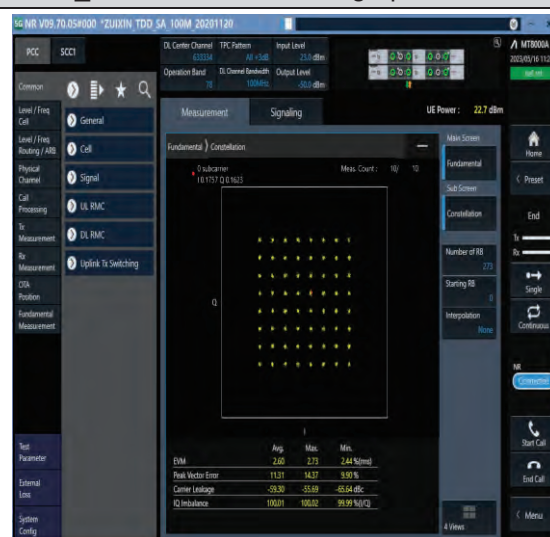
1-N78-3450-3550-PC1-30-100-M-8-CP-64QAM-Outer_Full-273@0-Ant1-see graph-PASS
