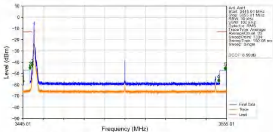
n77d_30kHz_SISO_NTNV_100MHz_CP-OFDM_QPSK_3500.01MHz_Edge_1RB_Left_Ant1
