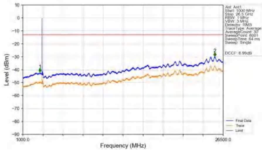
n77d_30kHz_SISO_NTNV_90MHz_DFT-s-OFDM_QPSK_3495MHz_Edge_1RB_Left_Ant1
