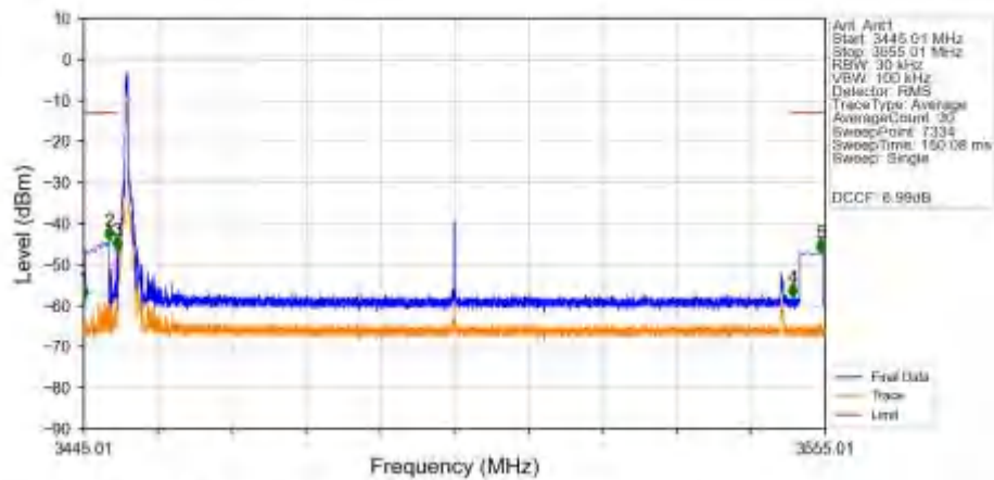
n77d_30kHz_SISO_NTNV_100MHz_DFT-s-OFDM_QPSK_3500.01MHz_Inner_1RB_Left_Ant1
