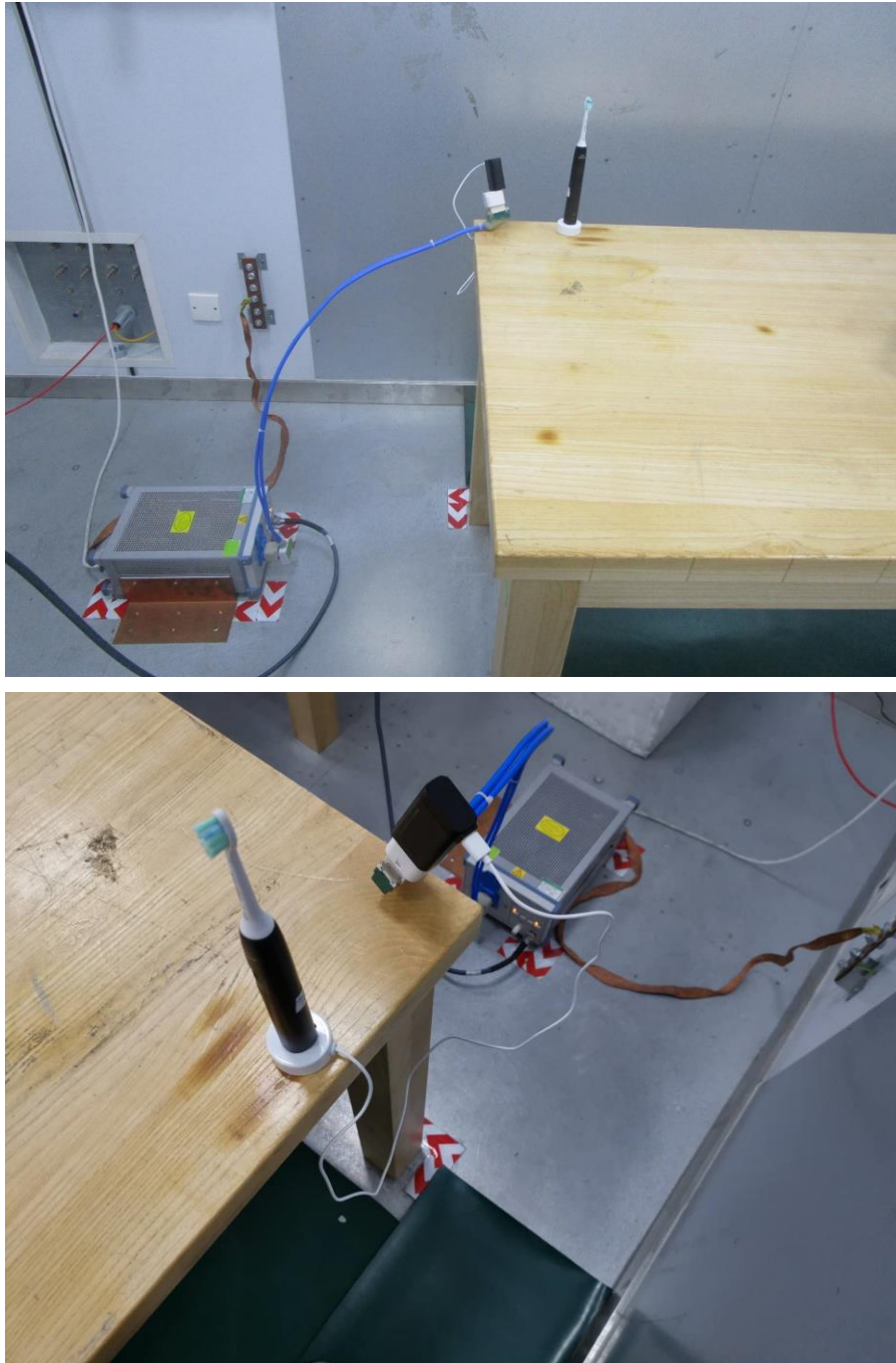
Conducted Emissions test setup photo
