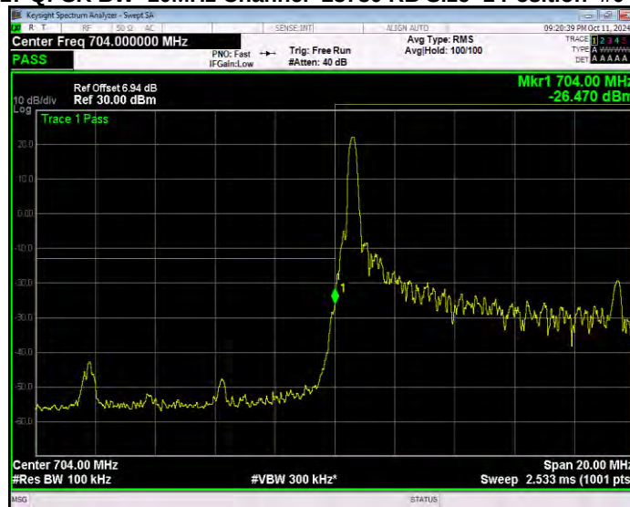
Band17 QPSK BW=10MHz Channel=23780 RB Size=1 Position=#Max Extended
