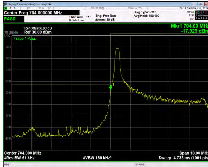
Band17 16QAM BW=5MHz Channel=23755 RB Size=1 Position=#Max Extended
