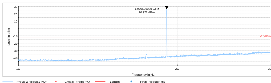
Plot #10 Radiated Emissions: 1-3 GHz
