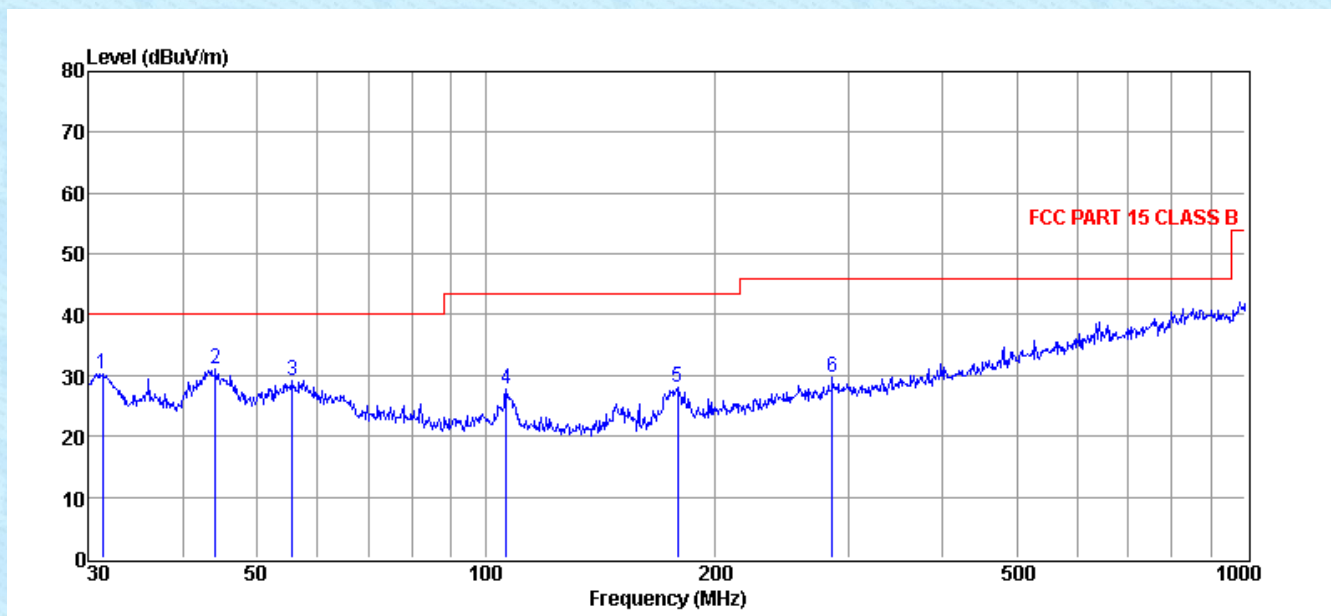
Quasi-peak measurement:
