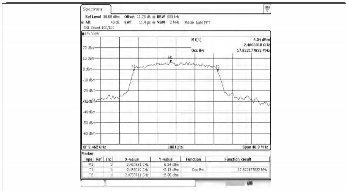
11N20SISO-Ant1-2462
