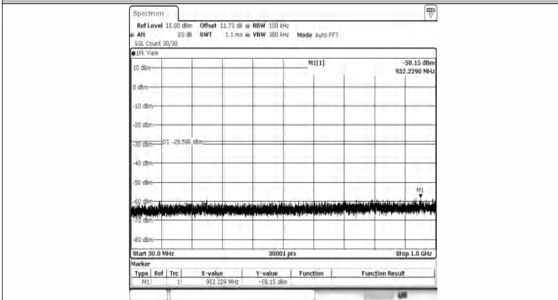
11N20SISO-Ant1-2462-30~1000-PASS
