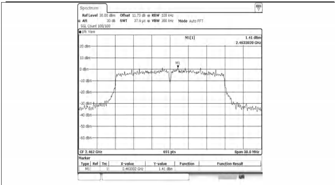
11N20SISO-Ant1-2462-0~Reference-PASS
