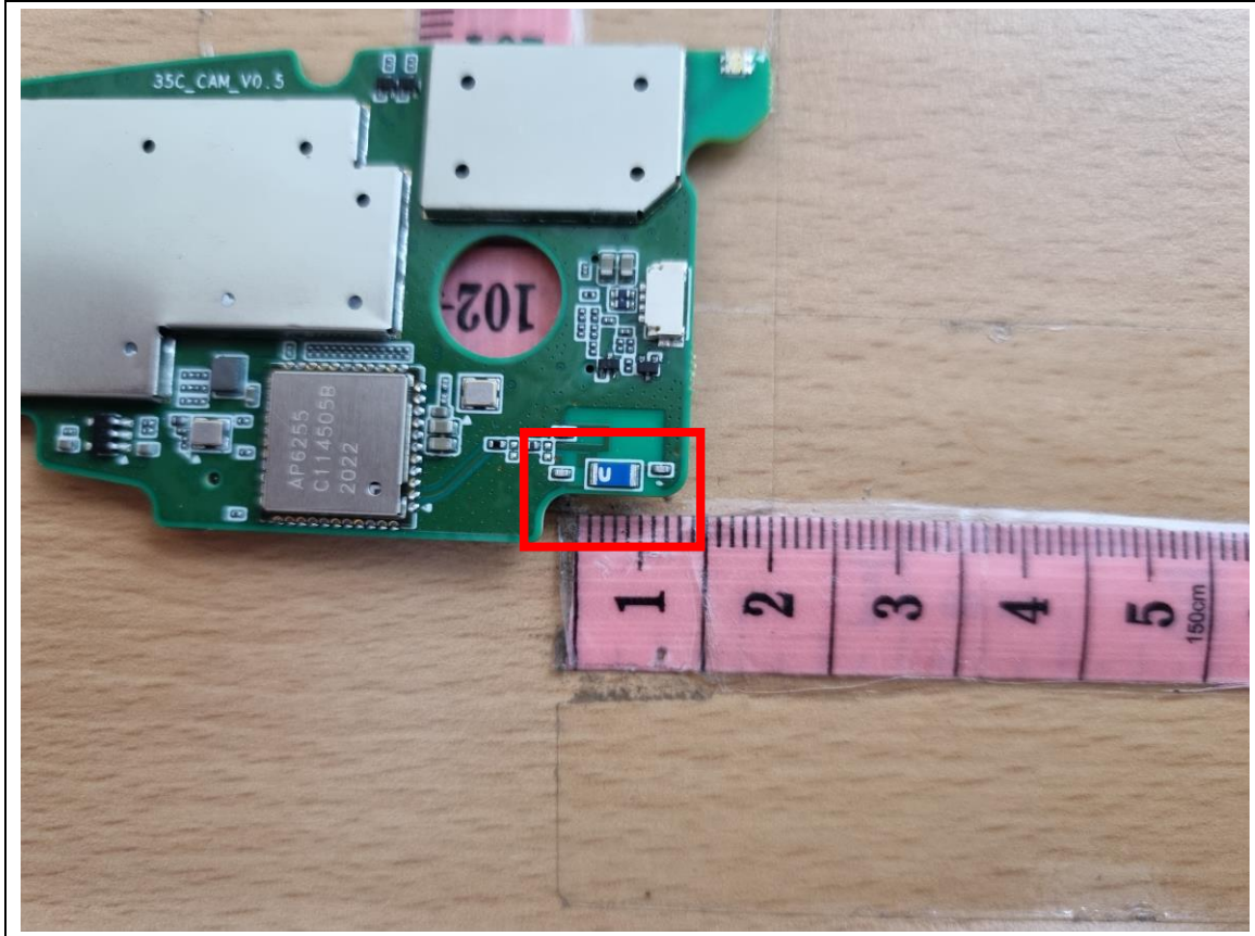
WLAN Antenna
