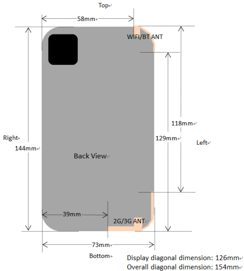
Fig.14.1 EUT Antenna Locations
