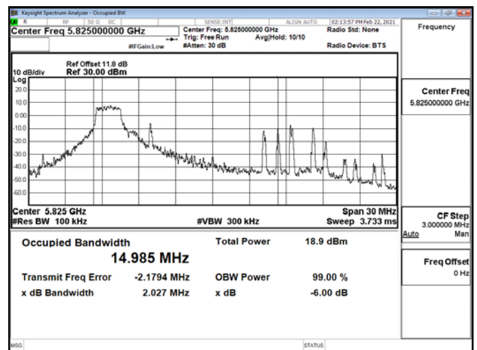
802.11ax_20MHz_Chain0_5825MHz_R26_0
