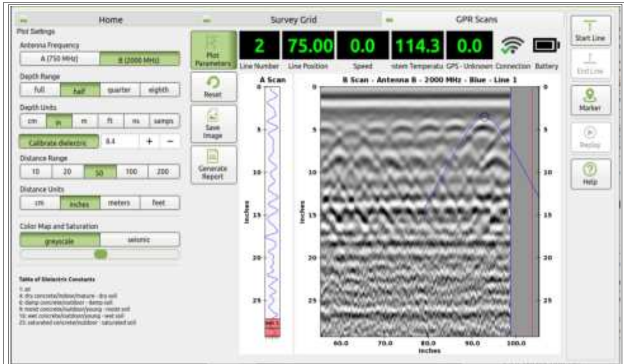
Figure 8: Plot settings dock. After clicking Calibrate dielectric , touch the top of a hyperbola. Then touch \pm or = until blue hyperbola matches the reflected radar arrivals on the screen.
