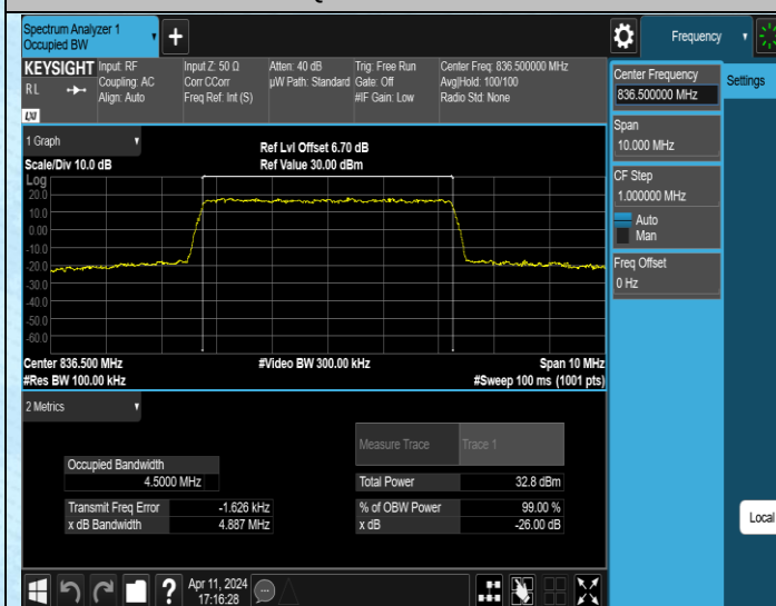
Band5-5MHz-16QAM-20525-25RB#0-PASS
