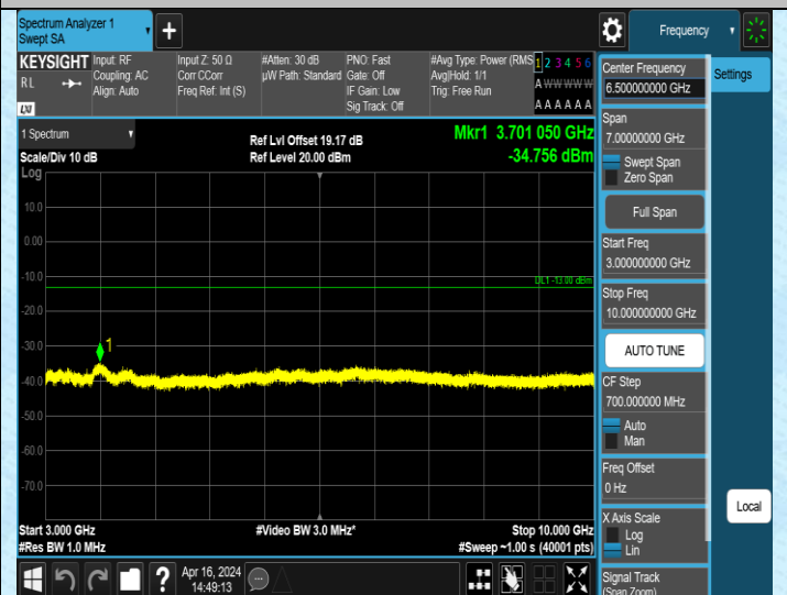
Band5_1.4MHz_QPSK_20525_1RB#0_3000~10000_3000~10000
