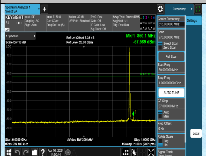
Band5_3MHz_QPSK_20415_1RB#0_30~1000_30~1000
