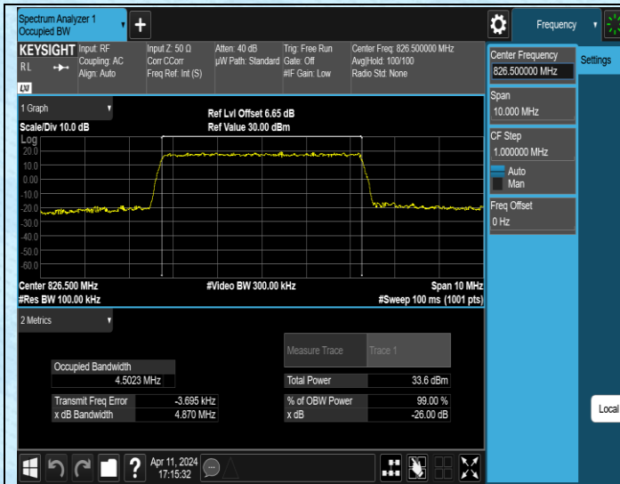
Band5-5MHz-QPSK-20425-25RB#0-PASS
