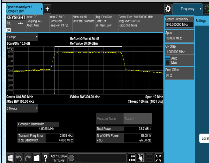
Band5-5MHz-QPSK-20625-25RB#0-PASS
