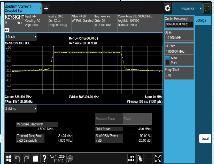
Band5-5MHz-QPSK-20525-25RB#0-PASS
