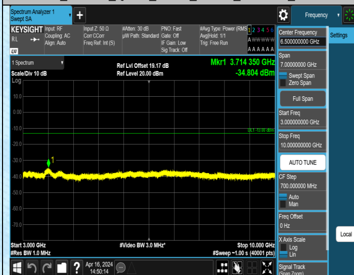
Band5_1.4MHz_QPSK_20643_1RB#0_3000~10000_3000~10000
