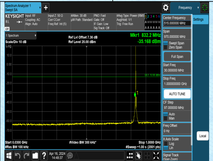
Band5_1.4MHz_QPSK_20525_1RB#0_30~1000_30~1000
