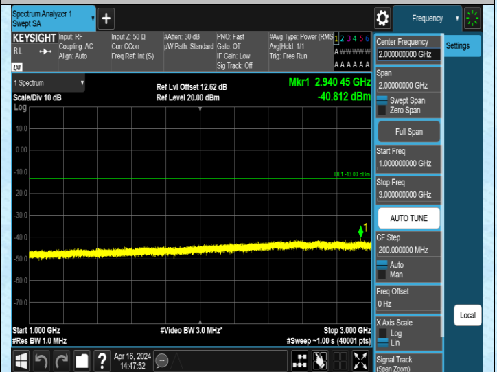
Band5_1.4MHz_QPSK_20407_1RB#0_1000~3000_1000~3000
