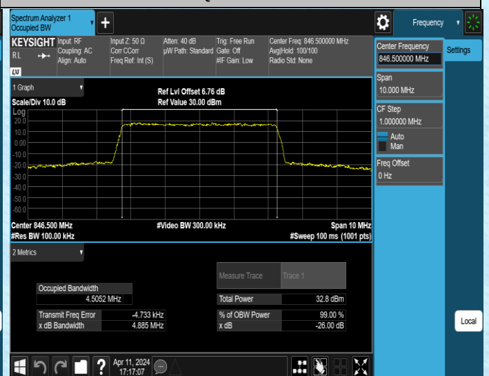
Band5-5MHz-16QAM-20625-25RB#0-PASS
