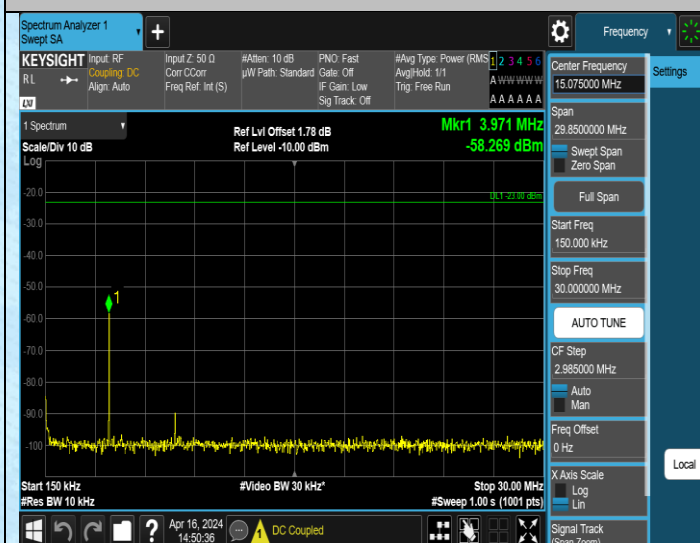
Band5_3MHz_QPSK_20415_1RB#0_0.15~30_0.15~30
