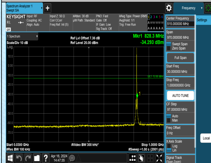
Band5_1.4MHz_QPSK_20407_1RB#0_30~1000_30~1000
