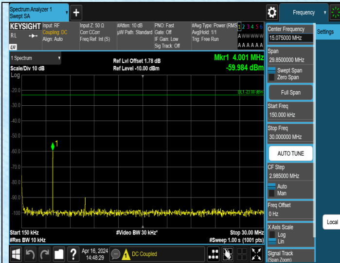
Band5_1.4MHz_QPSK_20525_1RB#0_0.15~30_0.15~30
