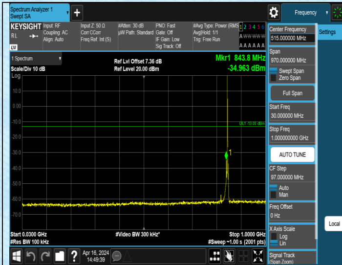
Band5_1.4MHz_QPSK_20643_1RB#0_30~1000_30~1000
