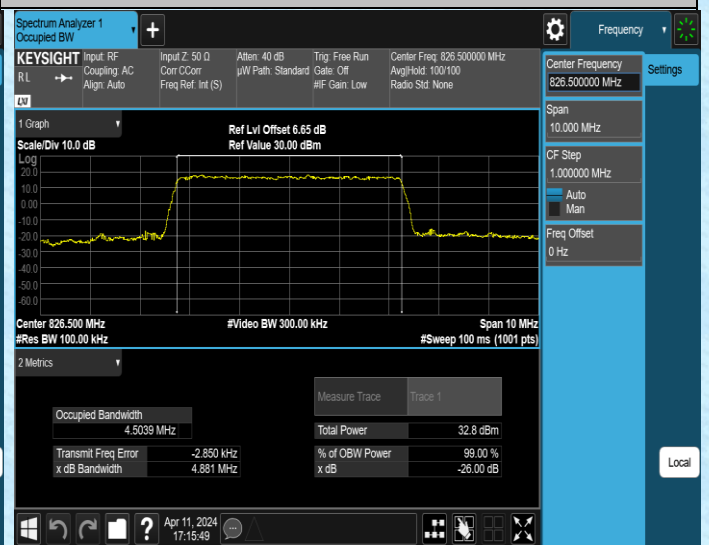
Band5-5MHz-16QAM-20425-25RB#0-PASS
