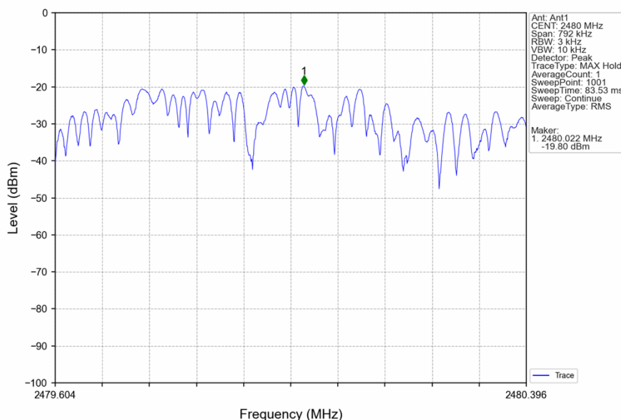
1M_HCH_2480MHz_Ant1_NTNV
