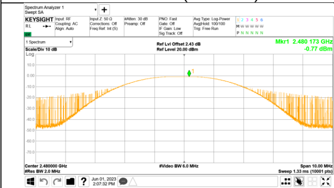
Channel 39 (2480MHz)
