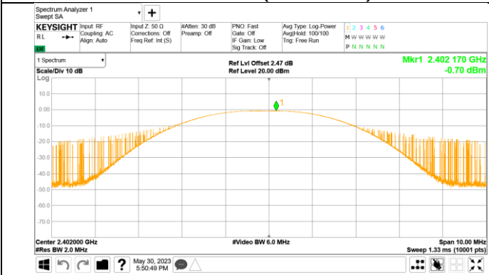
Channel 0 (2402MHz)
