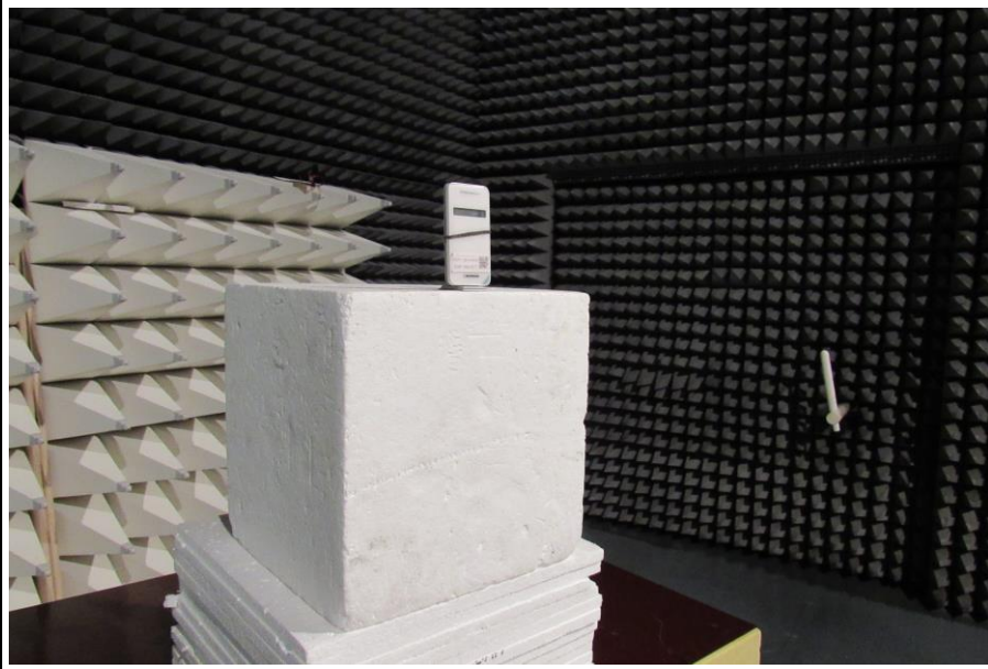
Test Setup above 1 GHz -Detail View
