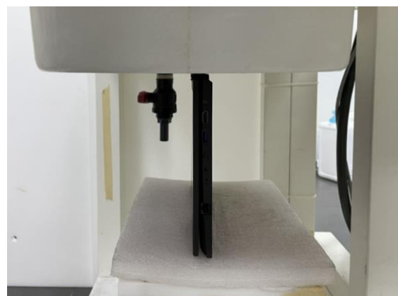
Fig.5 EUT Bottom side to flat phantom (Tablet mode)
