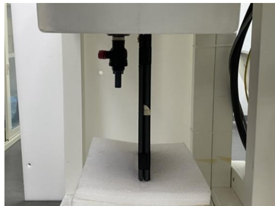
Fig.6 EUT Right side to flat phantom (Tablet mode)
