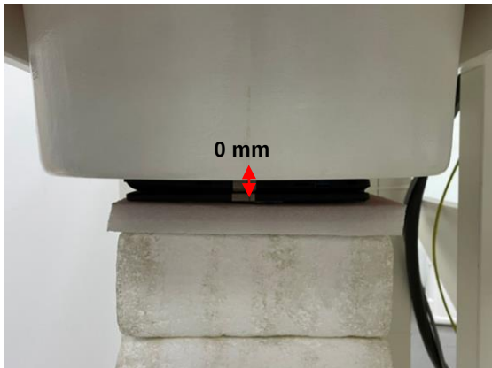
Fig.3 EUT Back side to flat phantom (Tablet mode)
