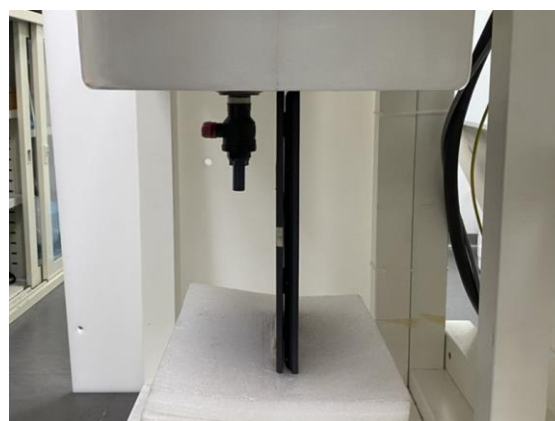
Fig.7 EUT Left side to flat phantom (Tablet mode)
