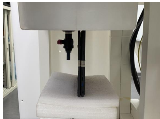
Fig.4 EUT Top side to flat phantom (Tablet mode)
