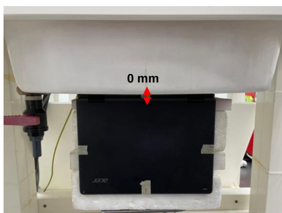
Fig.8 EUT Bottom side to flat phantom (Laptop mode)
