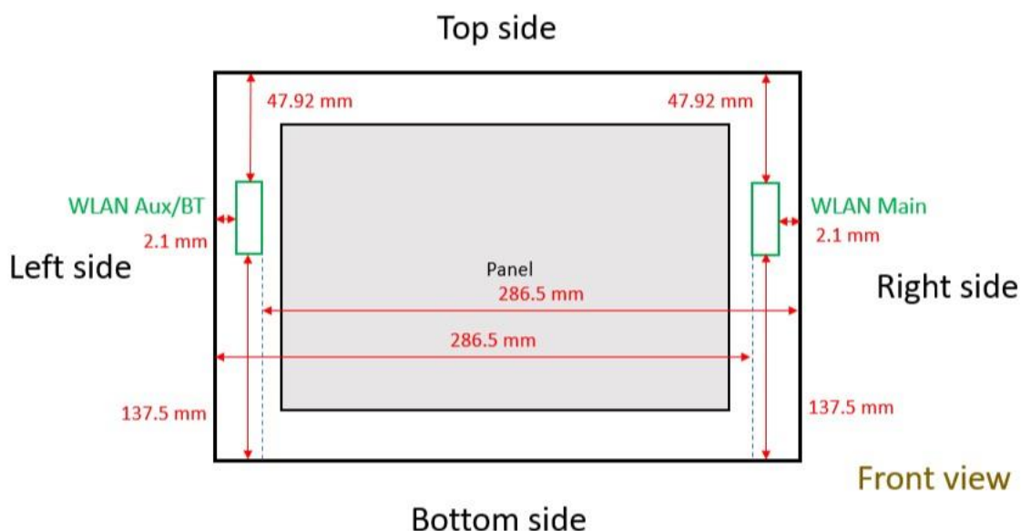
Fig.10 Antenna location of EUT (Tablet mode)
