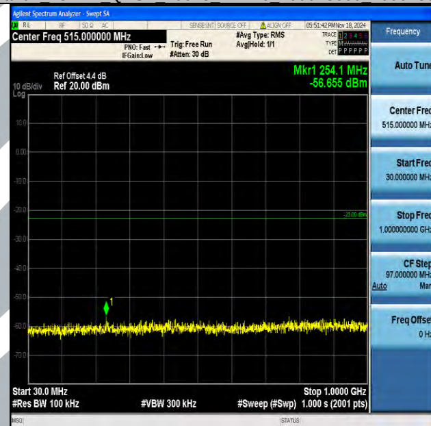
Band4_15MHz_QPSK_20175_1RB#0_30~1000_30~1000
