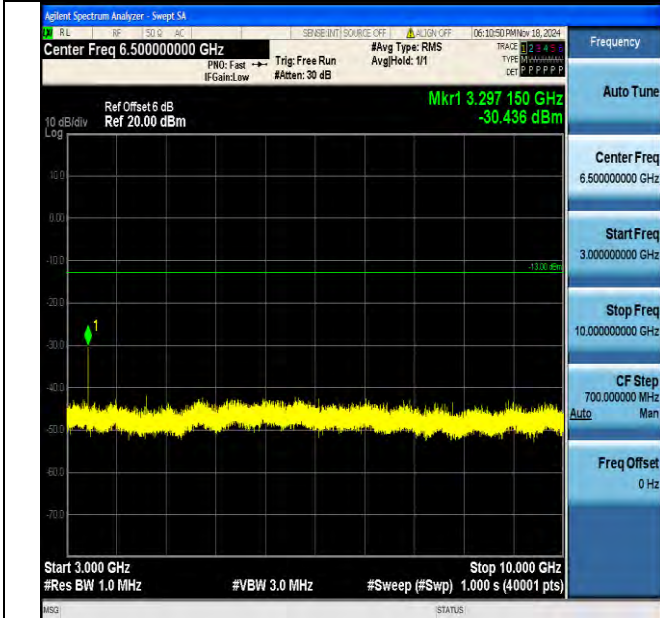
Band5_1.4MHz_QPSK_20407_1RB#0_3000~10000_3000~10000
