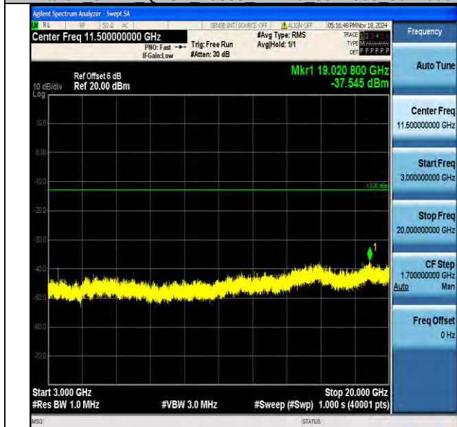
Band4_3MHz_QPSK_20385_1RB#0_3000~20000_3000~20000
