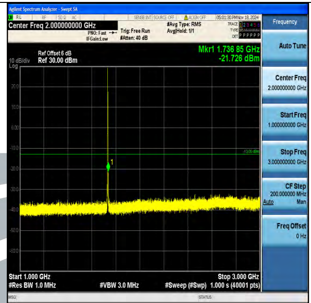
Band4_1.4MHz_16QAM_20175_1RB#0_1000~3000_1000~3000
