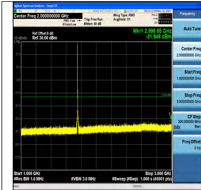
Band4_5MHz_16QAM_20375_1RB#0_1000~3000_1000~3000
