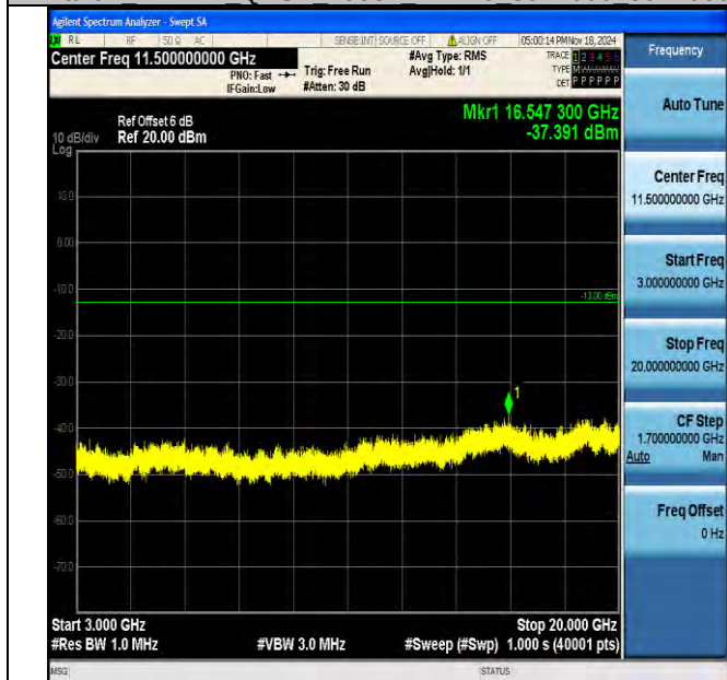
Band4_1.4MHz_QPSK_19957_1RB#0_3000~20000_3000~20000
