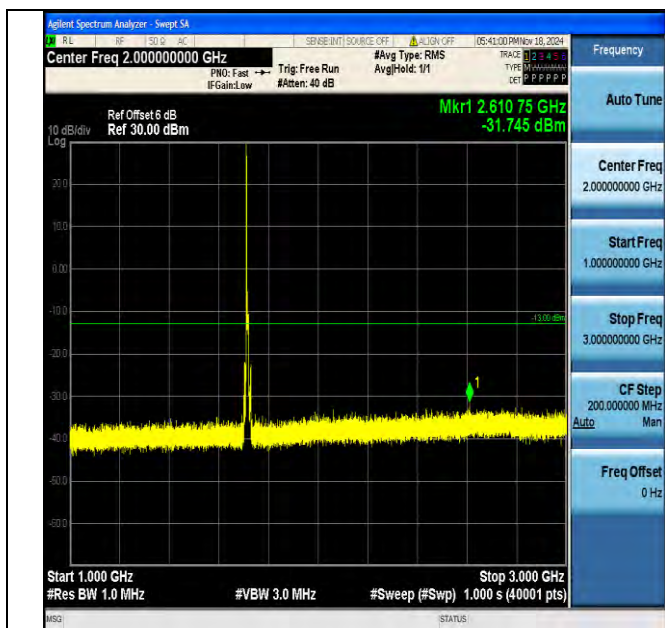
Band4_10MHz_16QAM_20000_1RB#0_1000-3000_1000-3000
