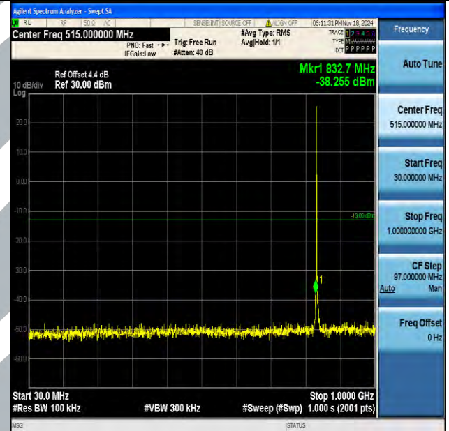
Band5_1.4MHz_QPSK_20525_1RB#0_30~1000_30~1000
