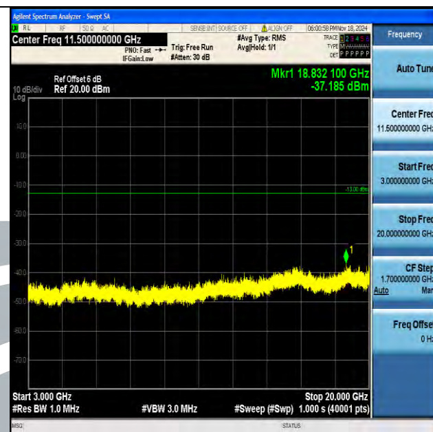
Band4_20MHz_16QAM_20050_1RB#0_3000~20000_3000~20000
