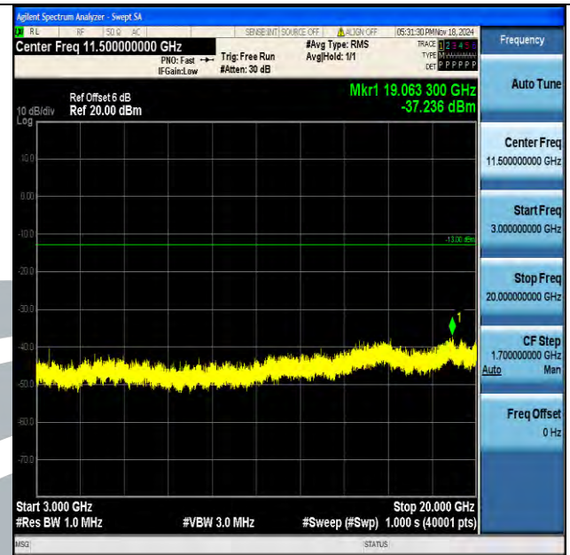
Band4_5MHz_16QAM_20375_1RB#0_3000~20000_3000~20000
