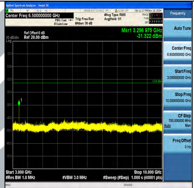
Band5_1.4MHz_16QAM_20407_1RB#0_3000~10000_3000~10000
