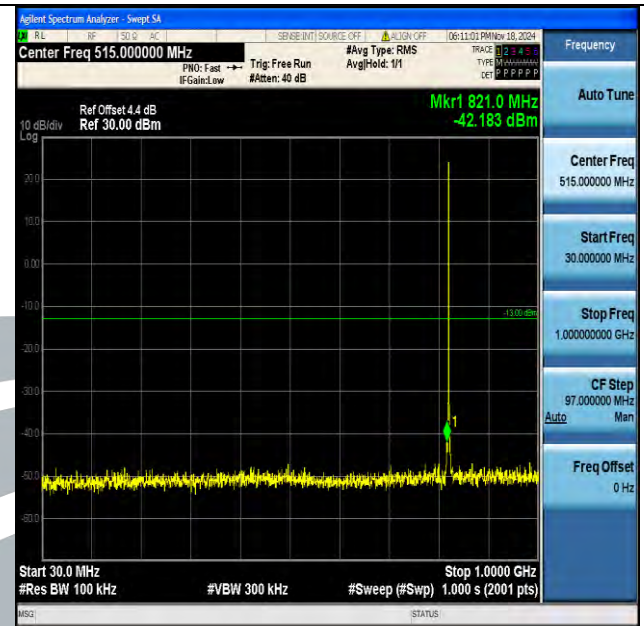
Band5_1.4MHz_16QAM_20407_1RB#0_30~1000_30~1000
