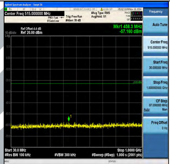
Band4_1.4MHz_16QAM_20393_1RB#0_30~1000_30~1000
