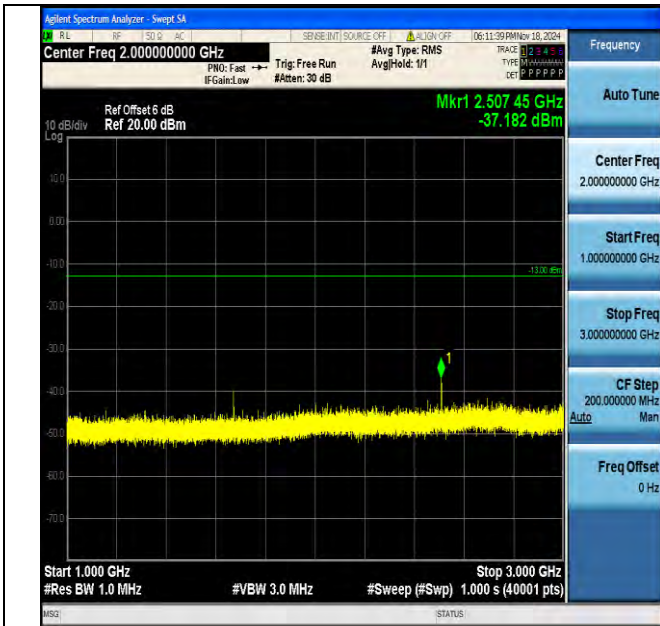
Band5_1.4MHz_QPSK_20525_1RB#0_1000~3000_1000~3000
