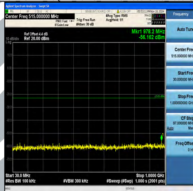
Band4_15MHz_16QAM_20325_1RB#0_30~1000_30~1000
