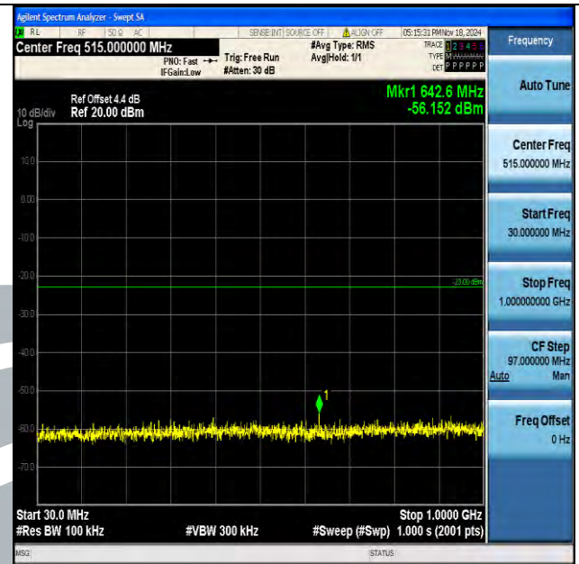
Band4_3MHz_QPSK_20175_1RB#0_30~1000_30~1000
