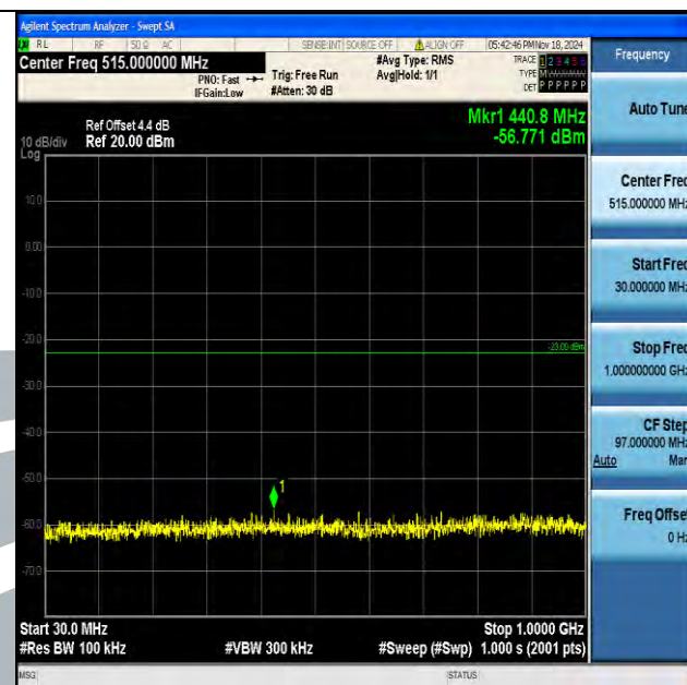
Band4_10MHz_16QAM_20350_1RB#0_30~1000_30~1000
