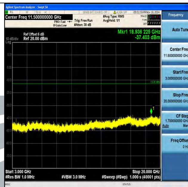
Band4_15MHz_QPSK_20175_1RB#0_3000~20000_3000~20000
