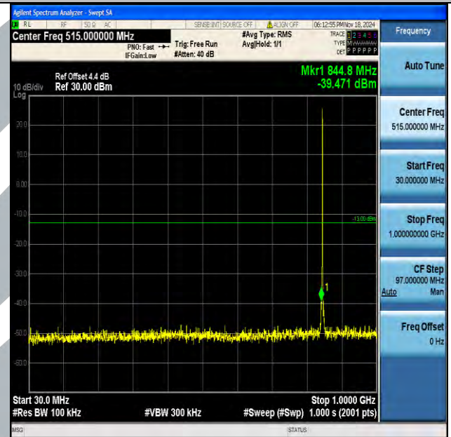
Band5_1.4MHz_16QAM_20643_1RB#0_30~1000_30~1000
