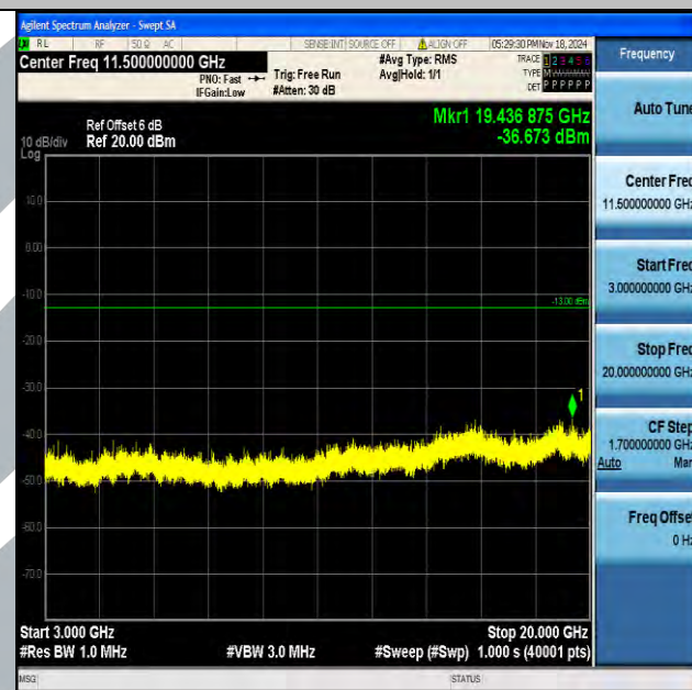
Band4_5MHz_16QAM_19975_1RB#0_3000~20000_3000~20000
