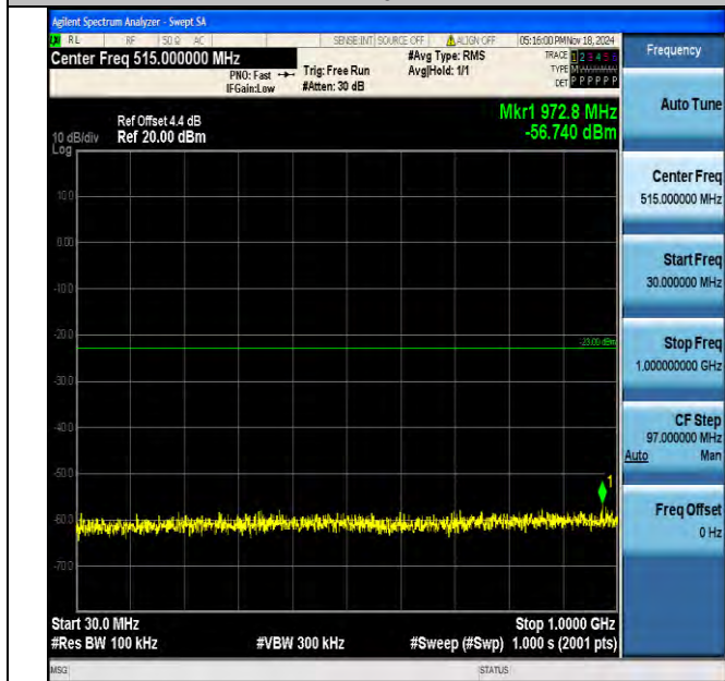
Band4_3MHz_16QAM_20175_1RB#0_30~1000_30~1000
