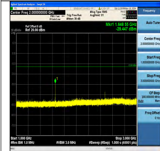
Band5_1.4MHz_16QAM_20407_1RB#0_1000~3000_1000~3000
