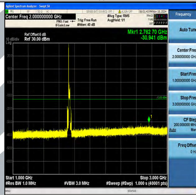
Band4_20MHz_16QAM_20175_1RB#0_1000~3000_1000~3000
