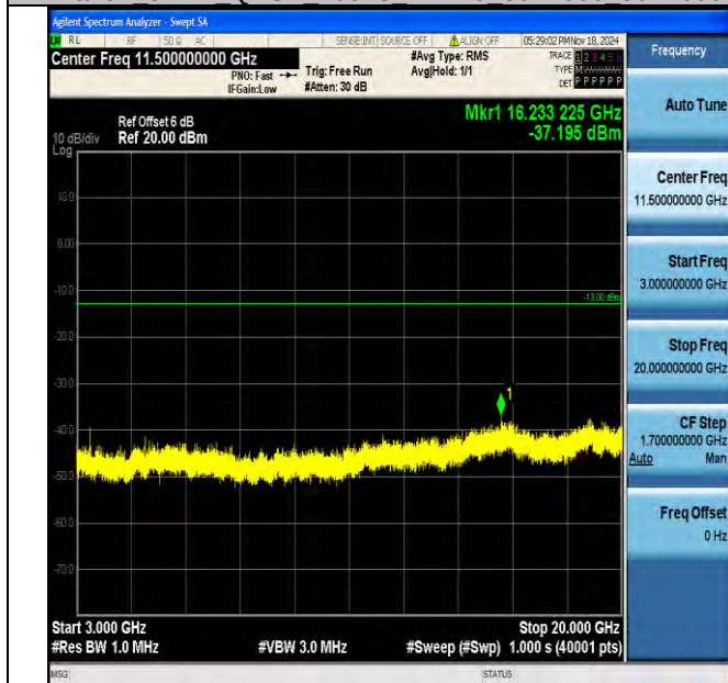
Band4_5MHz_QPSK_19975_1RB#0_3000~20000_3000~20000
