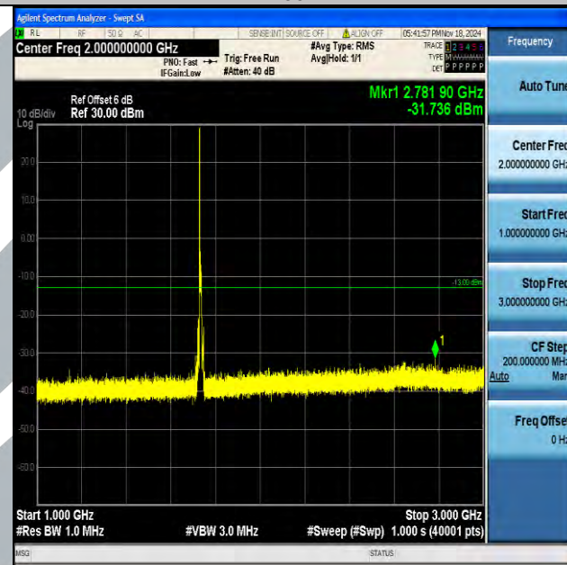
Band4_10MHz_16QAM_20175_1RB#0_1000-3000_1000-3000
