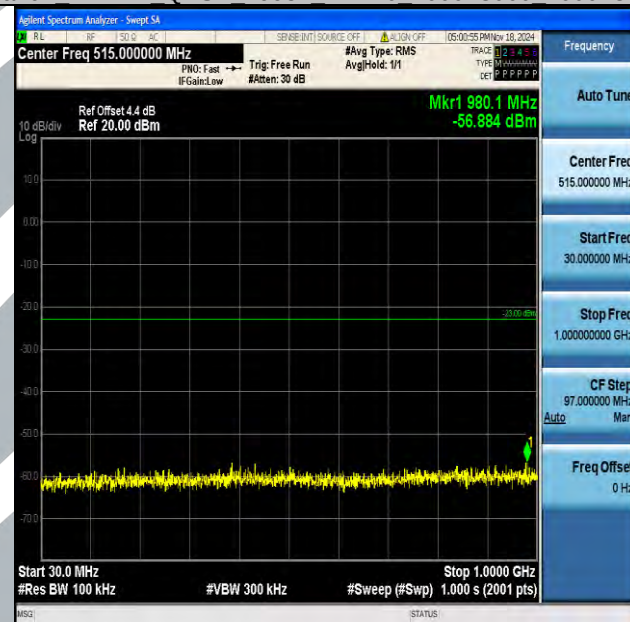
Band4_1.4MHz_QPSK_20175_1RB#0_30~1000_30~1000
