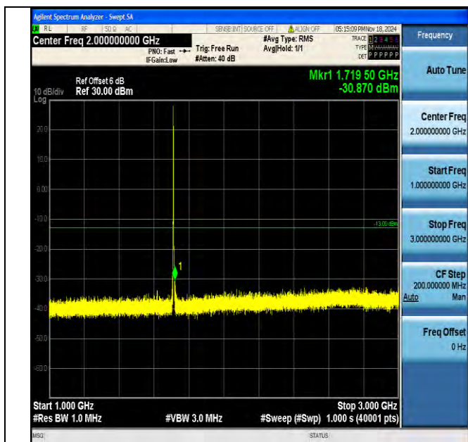
Band4_3MHz_16QAM_19965_1RB#0_1000~3000_1000~3000
