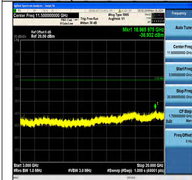
Band4_15MHz_16QAM_20175_1RB#0_3000~20000_3000~20000
