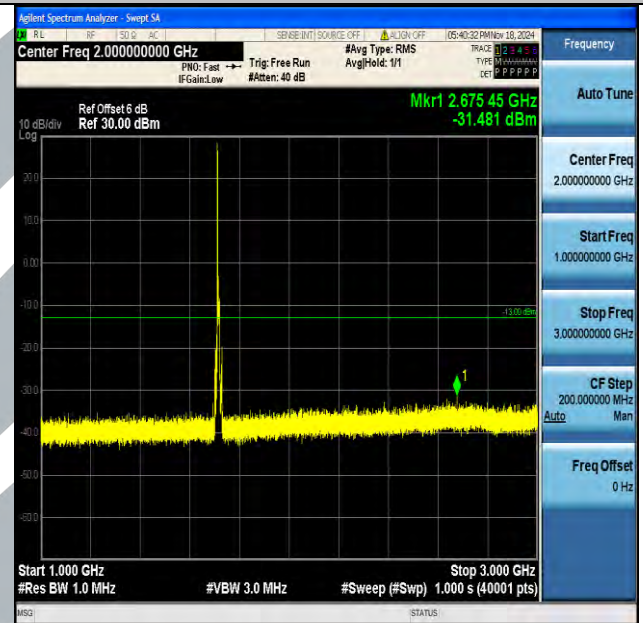
Band4_10MHz_QPSK_20000_1RB#0_1000~3000_1000~3000
