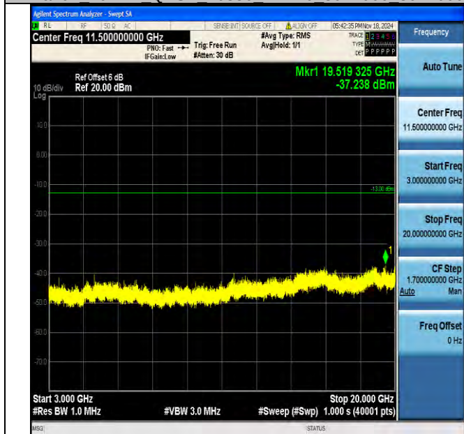
Band4_10MHz_QPSK_20350_1RB#0_3000~20000_3000~20000
