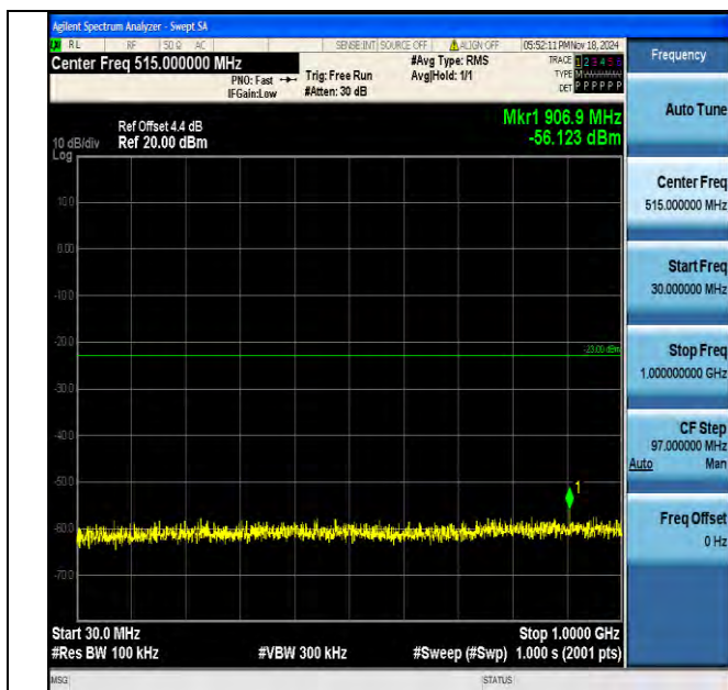
Band4_15MHz_16QAM_20175_1RB#0_30~1000_30~1000
