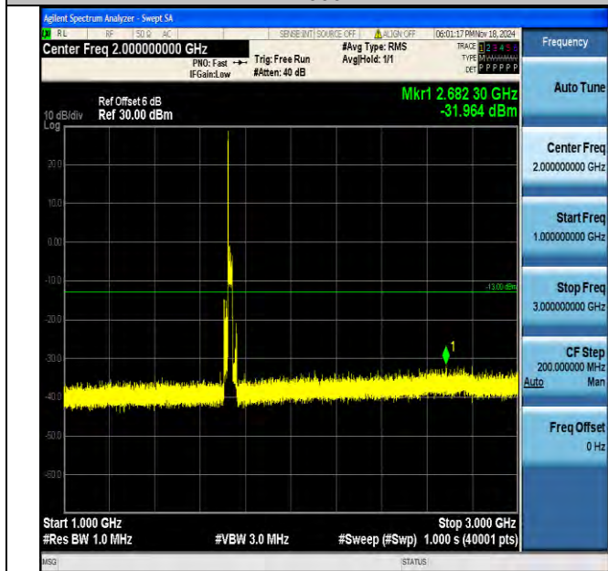
Band4_20MHz_QPSK_20175_1RB#0_1000~3000_1000~3000
