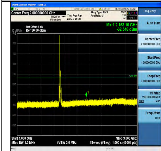
Band4_15MHz_16QAM_20025_1RB#0_1000~3000_1000~3000
