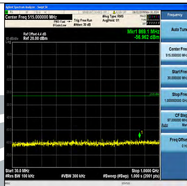
Band4_20MHz_QPSK_20175_1RB#0_30~1000_30~1000
