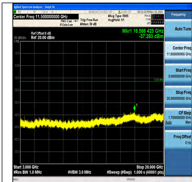
Band4_5MHz_QPSK_20375_1RB#0_3000~20000_3000~20000
