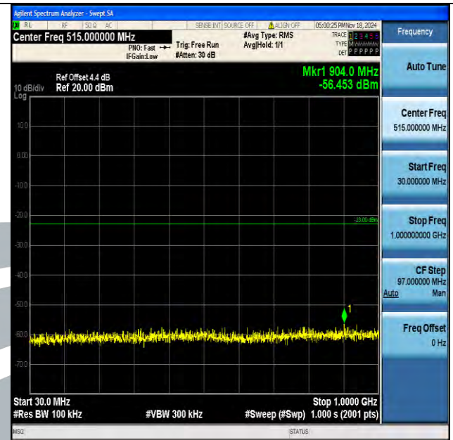
Band4_1.4MHz_16QAM_19957_1RB#0_30~1000_30~1000
