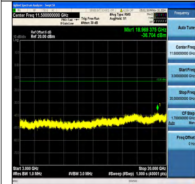
Band4_1.4MHz_16QAM_20175_1RB#0_3000~20000_3000~20000
