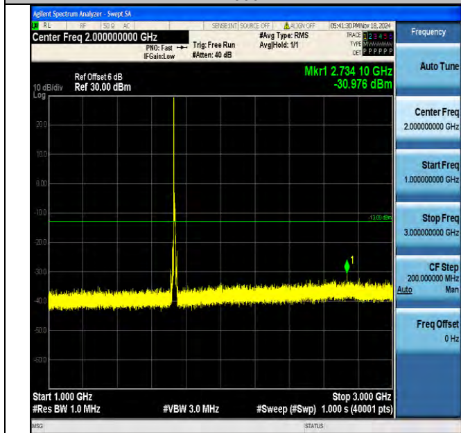
Band4_10MHz_QPSK_20175_1RB#0_1000~3000_1000~3000
