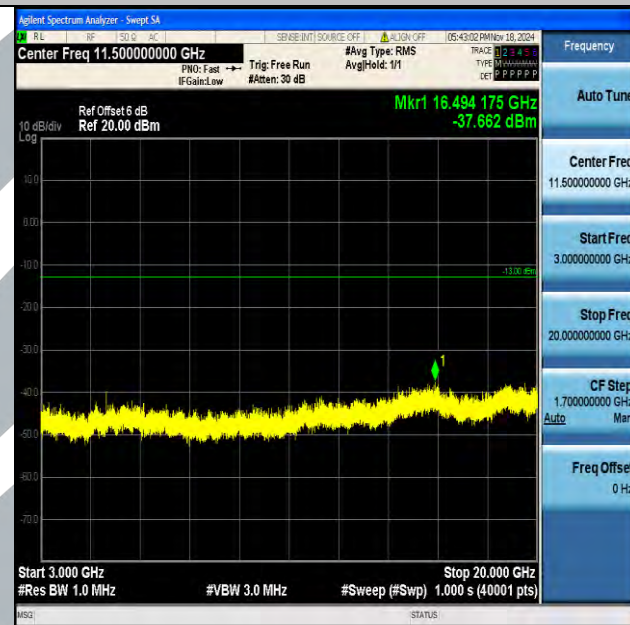
Band4_10MHz_16QAM_20350_1RB#0_3000~20000_3000~20000
