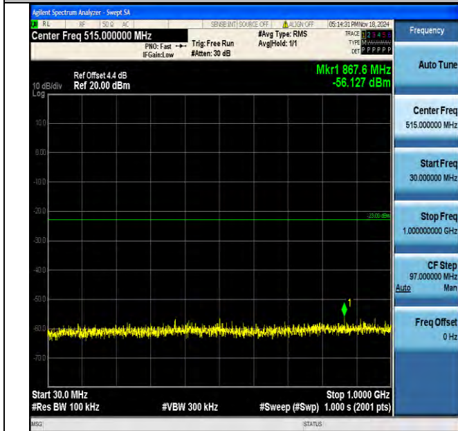
Band4_3MHz_QPSK_19965_1RB#0_30~1000_30~1000
