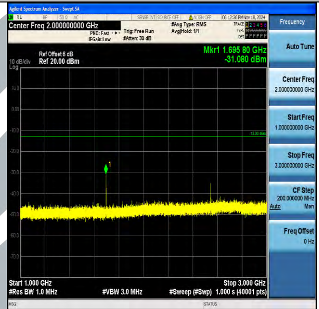
Band5_1.4MHz_QPSK_20643_1RB#0_1000~3000_1000~3000
