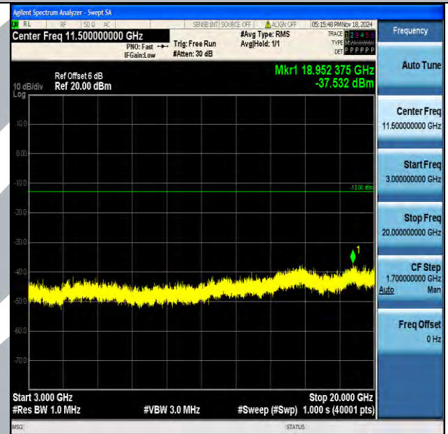
Band4_3MHz_QPSK_20175_1RB#0_3000~20000_3000~20000
