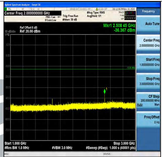
Band5_1.4MHz_16QAM_20525_1RB#0_1000~3000_1000~3000
