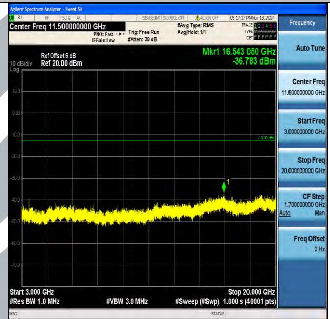
Band4_3MHz_16QAM_20385_1RB#0_3000~20000_3000~20000
