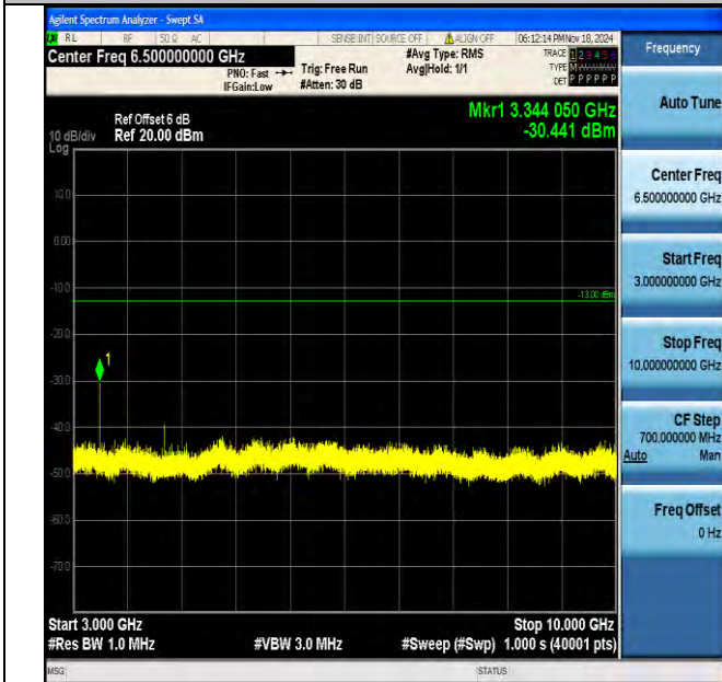
Band5_1.4MHz_16QAM_20525_1RB#0_3000~10000_3000~10000
