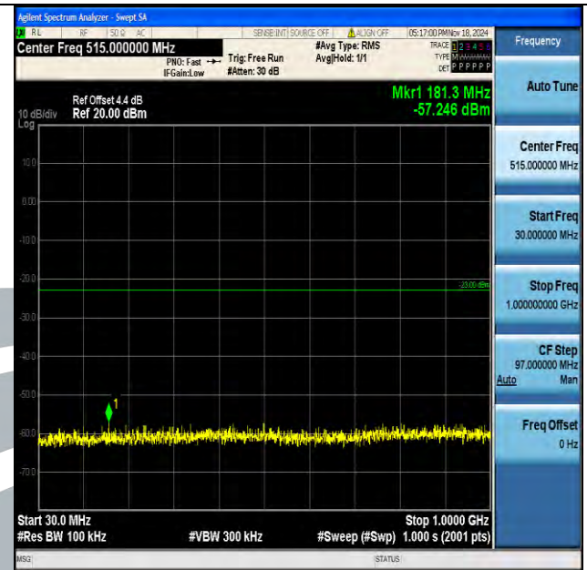
Band4_3MHz_16QAM_20385_1RB#0_30~1000_30~1000
