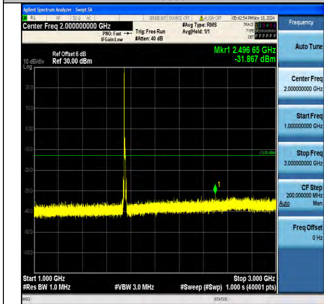
Band4_10MHz_16QAM_20350_1RB#0_1000~3000_1000~3000
