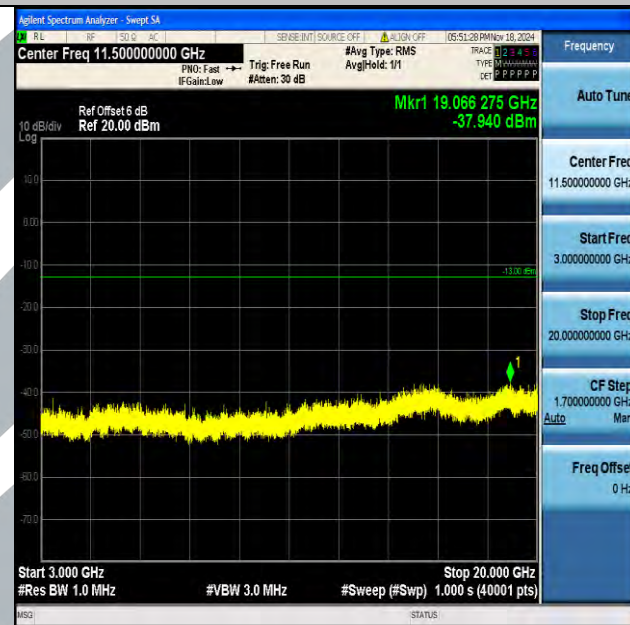
Band4_15MHz_16QAM_20025_1RB#0_3000~20000_3000~20000
