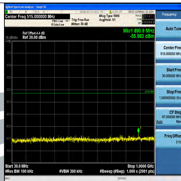
Band4_15MHz_16QAM_20025_1RB#0_30~1000_30~1000
