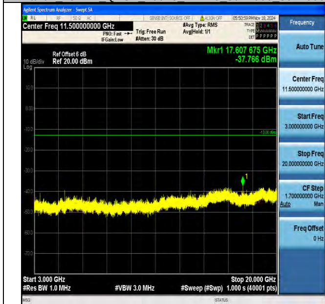
Band4_15MHz_QPSK_20025_1RB#0_3000~20000_3000~20000
