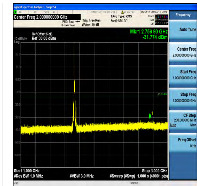
Band4_15MHz_QPSK_20175_1RB#0_1000~3000_1000~3000
