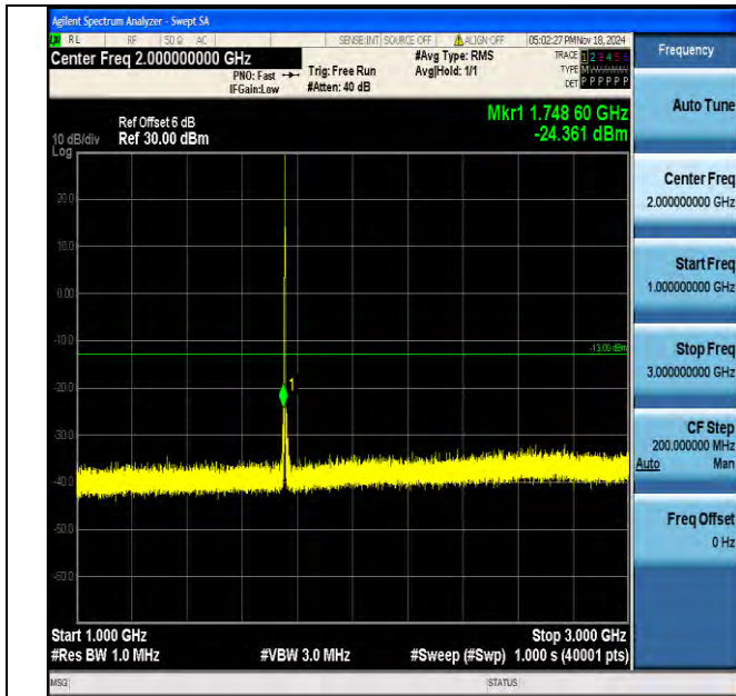
Band4_1.4MHz_16QAM_20393_1RB#0_1000~3000_1000~3000
