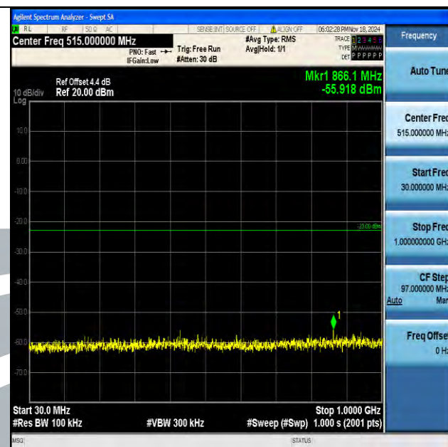
Band4_20MHz_16QAM_20300_1RB#0_30~1000_30~1000
