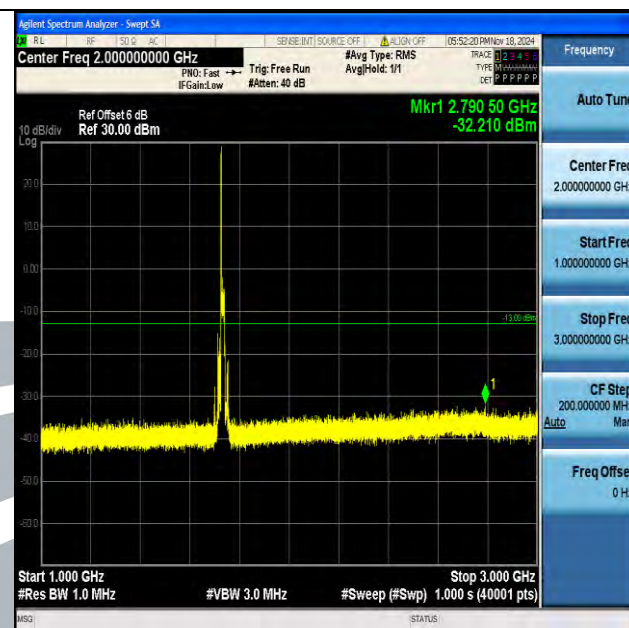
Band4_15MHz_16QAM_20175_1RB#0_1000~3000_1000~3000
