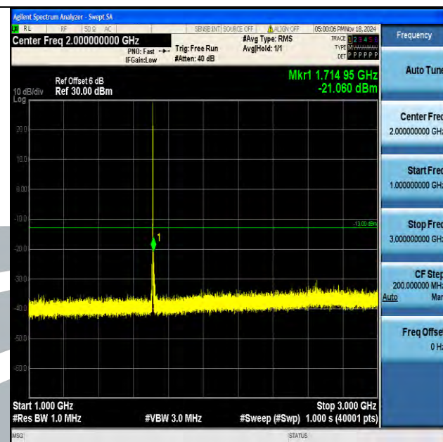
Band4_1.4MHz_QPSK_19957_1RB#0_1000~3000_1000~3000
