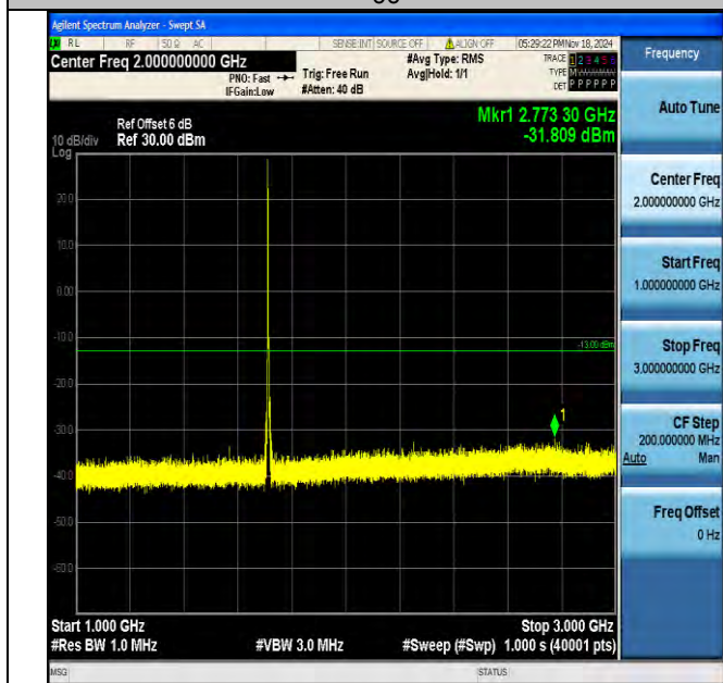
Band4_5MHz_16QAM_19975_1RB#0_1000~3000_1000~3000
