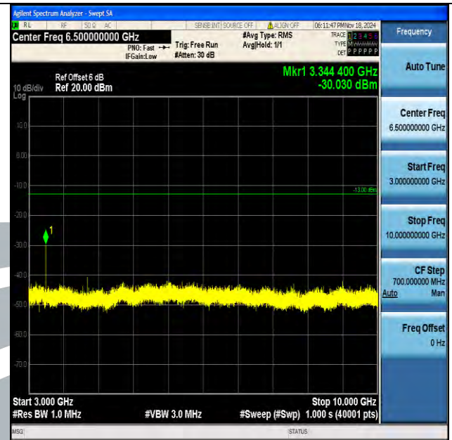
Band5_1.4MHz_QPSK_20525_1RB#0_3000~10000_3000~10000
