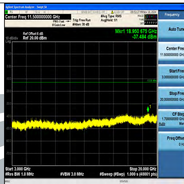
Band4_15MHz_16QAM_20325_1RB#0_3000-20000_3000-20000
