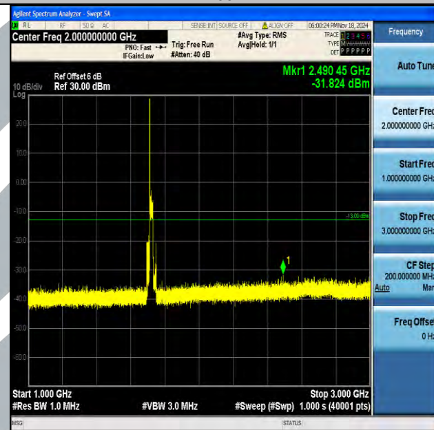
Band4_20MHz_QPSK_20050_1RB#0_1000-3000_1000-3000
