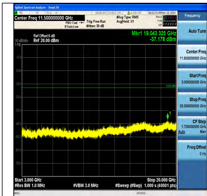
Band4_20MHz_16QAM_20175_1RB#0_3000~20000_3000~20000
