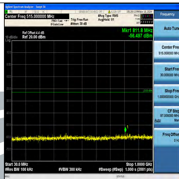
Band4_5MHz_16QAM_19975_1RB#0_30~1000_30~1000
