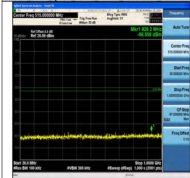
Band4 5MHz QPSK 20375 1RB#0 30~1000 30~1000
