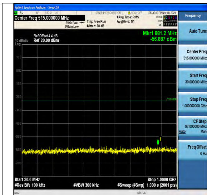
Band4_5MHz_16QAM_20175_1RB#0_30~1000_30~1000
