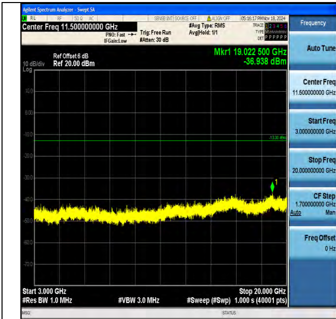
Band4_3MHz_16QAM_20175_1RB#0_3000~20000_3000~20000
