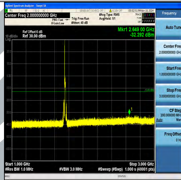
Band4_15MHz_QPSK_20325_1RB#0_1000~3000_1000~3000
