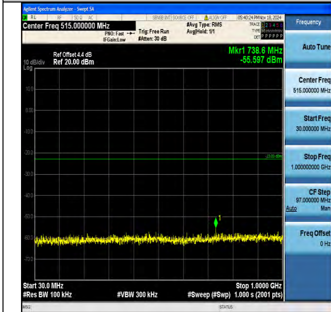
Band4_10MHz_QPSK_20000_1RB#0_30~1000_30~1000
