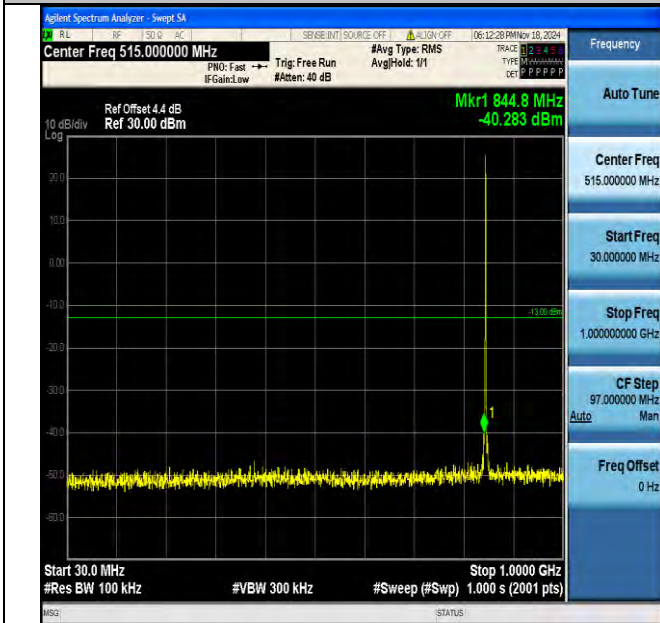
Band5_1.4MHz_QPSK_20643_1RB#0_30~1000_30~1000
