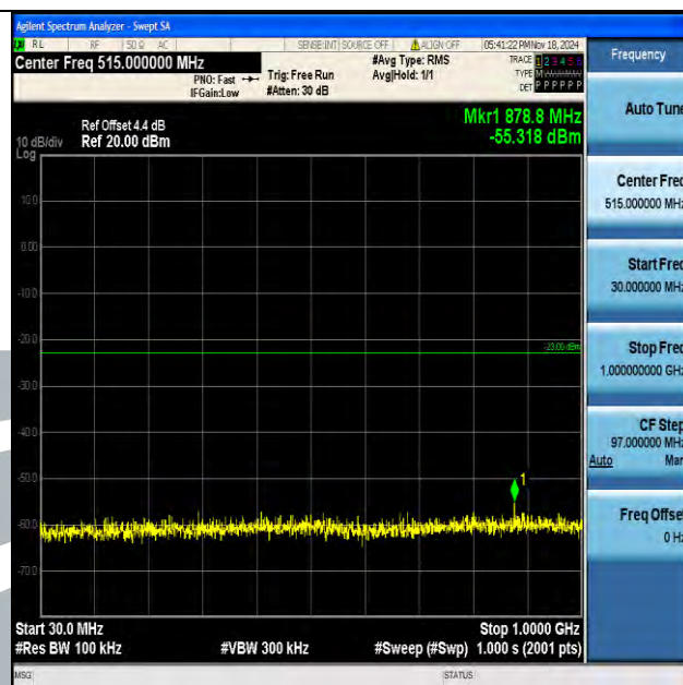
Band4_10MHz_QPSK_20175_1RB#0_30~1000_30~1000
