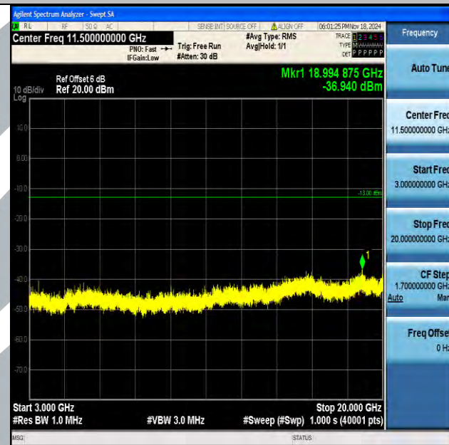
Band4_20MHz_QPSK_20175_1RB#0_3000~20000_3000~20000
