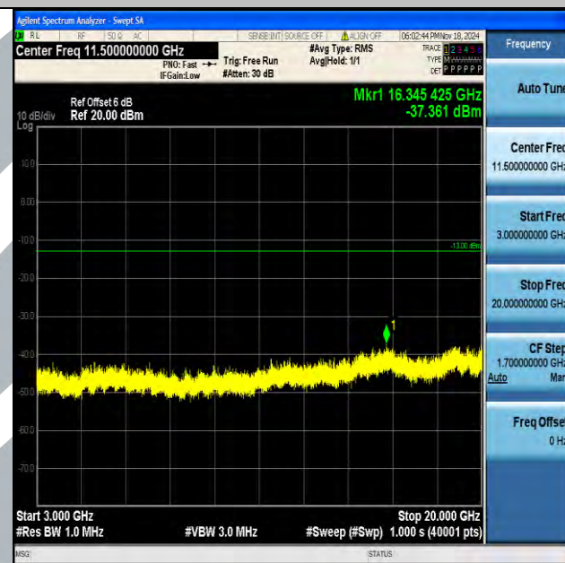
Band4_20MHz_16QAM_20300_1RB#0_3000~20000_3000~20000
