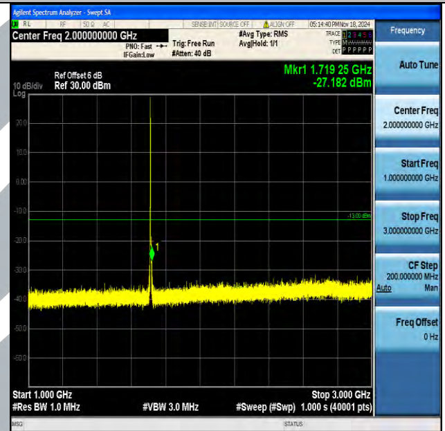
Band4_3MHz_QPSK_19965_1RB#0_1000~3000_1000~3000
