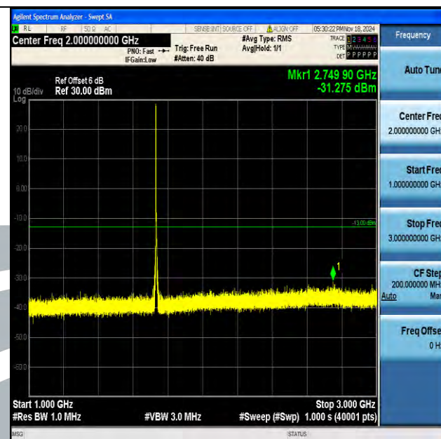
Band4_5MHz_16QAM_20175_1RB#0_1000~3000_1000~3000
