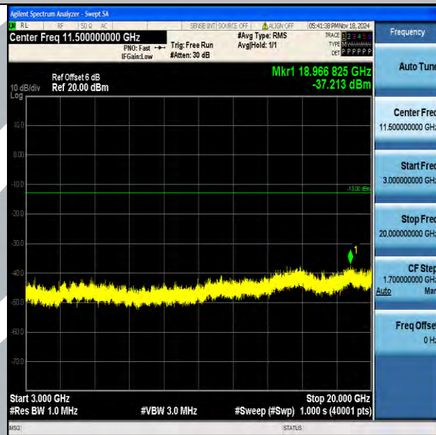
Band4_10MHz_QPSK_20175_1RB#0_3000~20000_3000~20000
