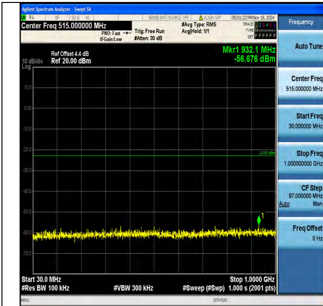
Band4_1.4MHz_16QAM_20175_1RB#0_30~1000_30~1000
