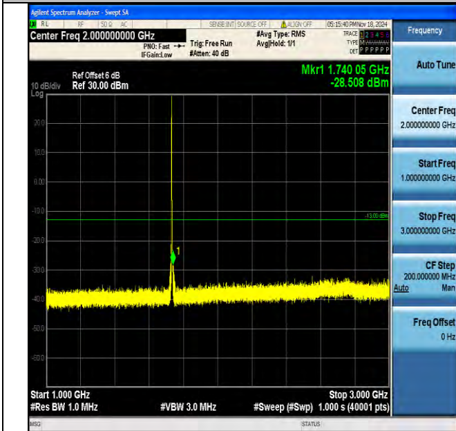
Band4_3MHz_QPSK_20175_1RB#0_1000~3000_1000~3000
