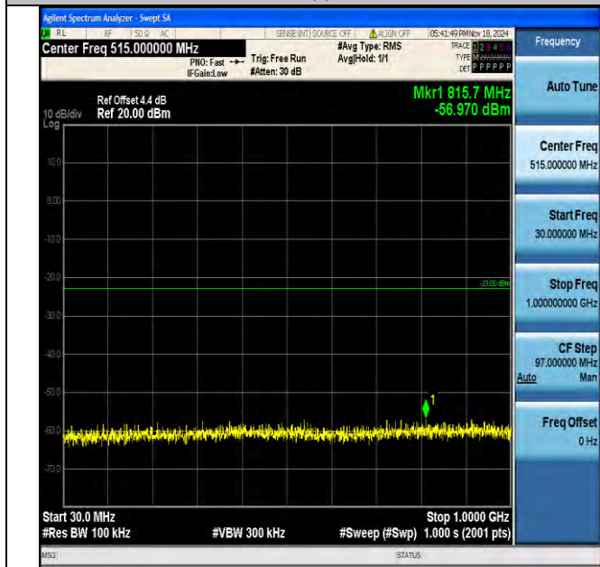
Band4_10MHz_16QAM_20175_1RB#0_30-1000_30-1000
