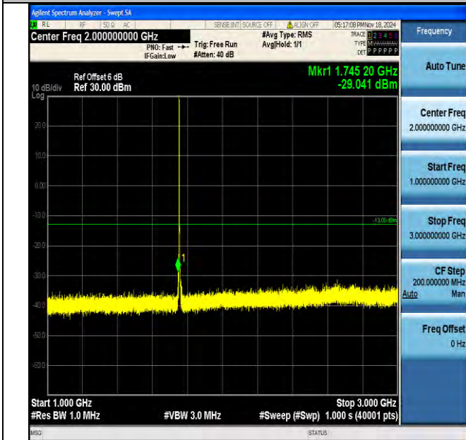
Band4_3MHz_16QAM_20385_1RB#0_1000~3000_1000~3000
