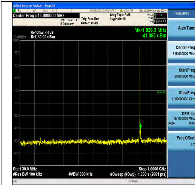
Band5 1.4MHz QPSK 20407 1RB#0 30~1000 30~1000
