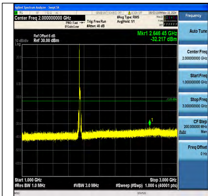
Band4_15MHz_16QAM_20325_1RB#0_1000-3000_1000-3000
