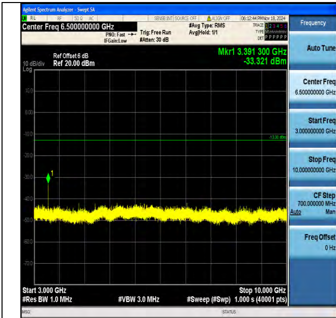
Band5_1.4MHz_QPSK_20643_1RB#0_3000~10000_3000~10000
