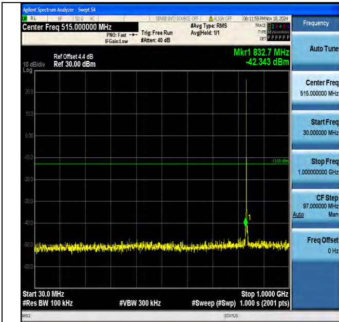
Band5_1.4MHz_16QAM_20525_1RB#0_30~1000_30~1000
