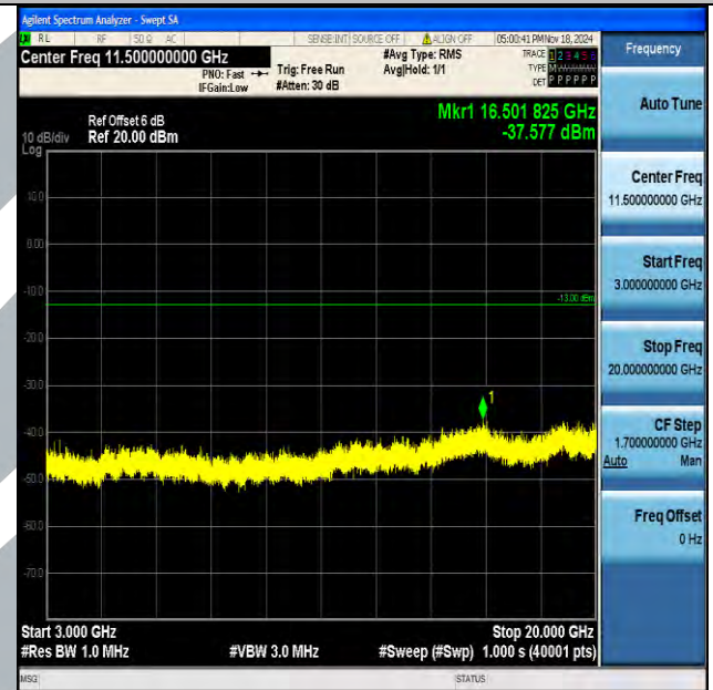
Band4_1.4MHz_16QAM_19957_1RB#0_3000~20000_3000~20000
