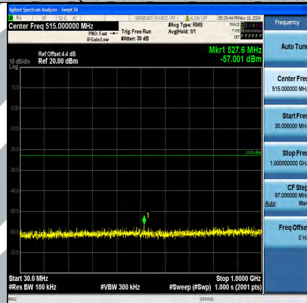
Band4_5MHz_QPSK_20175_1RB#0_30~1000_30~1000
