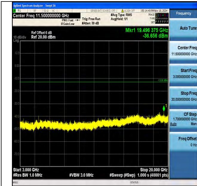
Band4_3MHz_QPSK_19965_1RB#0_3000~20000_3000~20000
