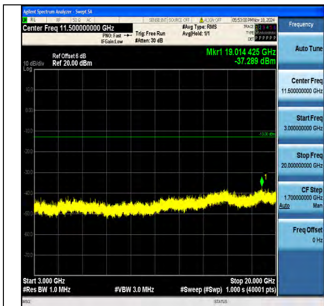
Band4_15MHz_QPSK_20325_1RB#0_3000~20000_3000~20000
