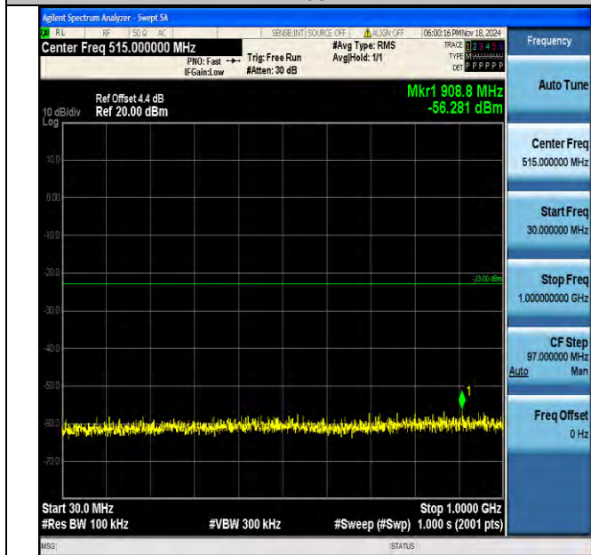
Band4_20MHz_QPSK_20050_1RB#0_30-1000_30-1000
