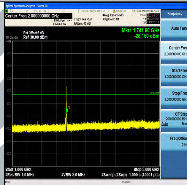
Band4_3MHz_16QAM_20175_1RB#0_1000~3000_1000~3000
