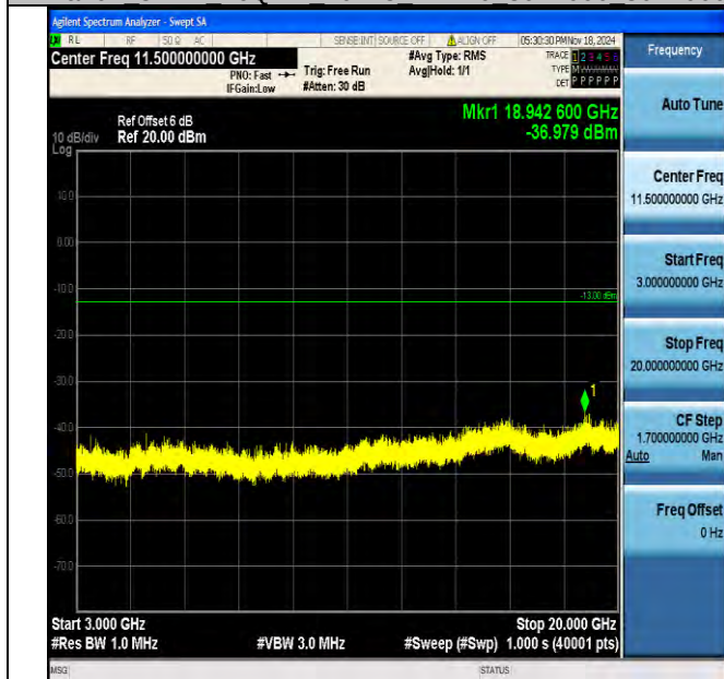
Band4_5MHz_16QAM_20175_1RB#0_3000~20000_3000~20000
