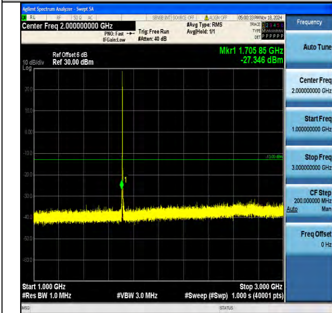
Band4_1.4MHz_16QAM_19957_1RB#0_1000~3000_1000~3000
