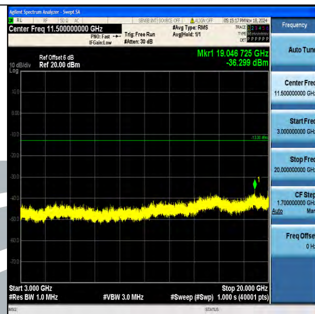
Band4_3MHz_16QAM_19965_1RB#0_3000~20000_3000~20000
