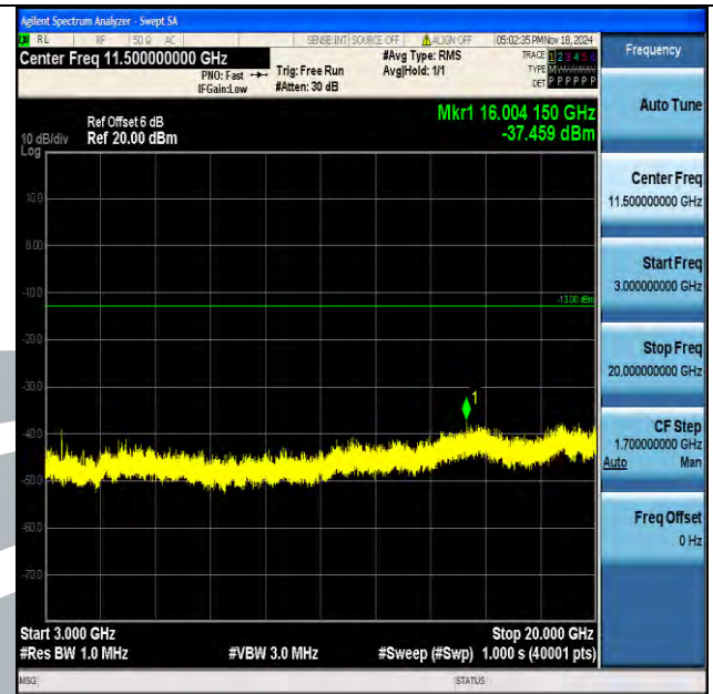
Band4_1.4MHz_16QAM_20393_1RB#0_3000~20000_3000~20000
