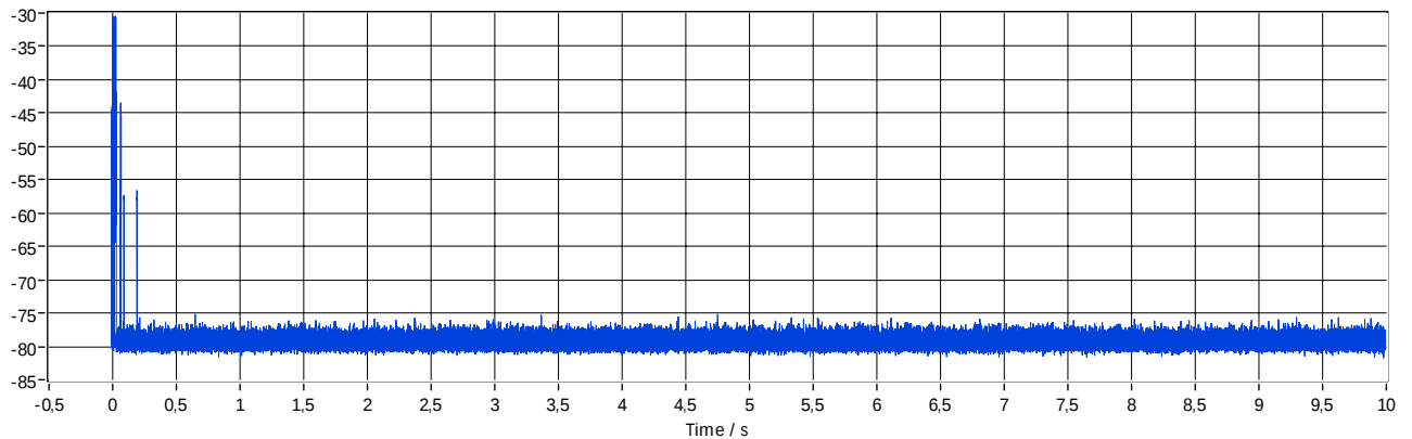
ZeroSpanGraph
