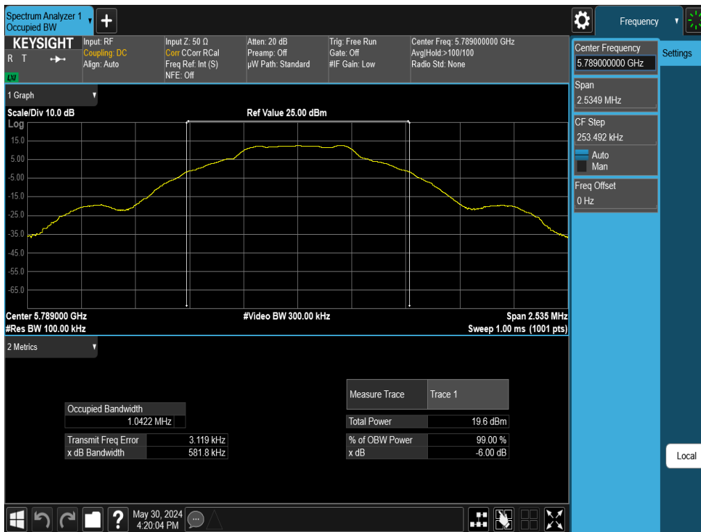
Plot 7-20. 6dB BW & 99% OBW Antenna WF5T (NB UNII BDR, ePA – 5789MHz)
