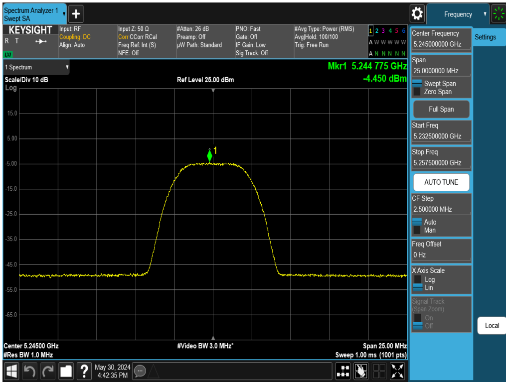
Plot 7-54. PSD Antenna WF5T (NB UNII HDR8, iPA– 5245MHz)
