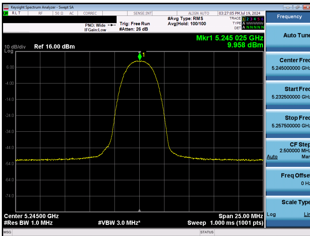
Plot 7-45. PSD Antenna WF5T (NB UNII HDR4, ePA- 5245MHz)
