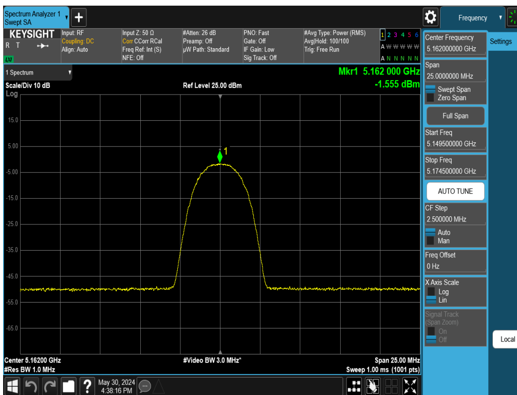
7-46. PSD Antenna WF5T (NB UNII HDR4, iPA - 5162MHz)
