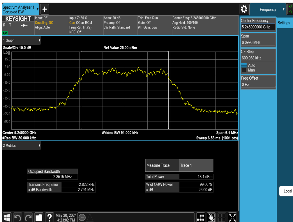
Plot 7-6. 26dB BW & 99% OBW Antenna WF5T (NB UNII HDR4, ePA– 5245MHz)
