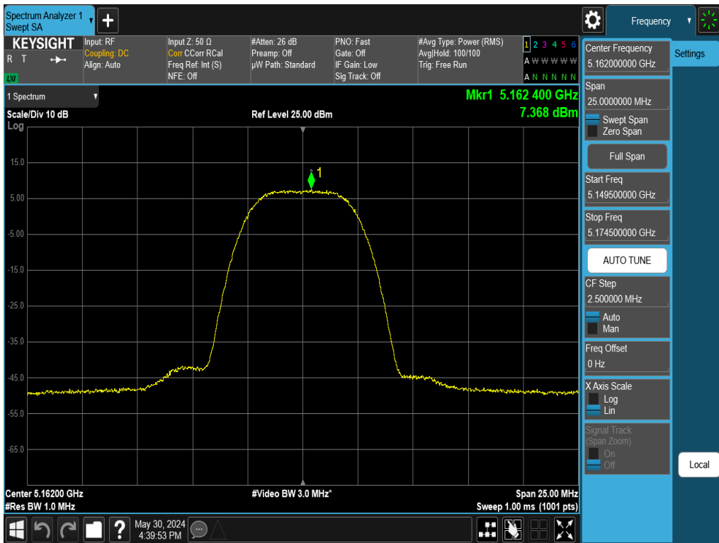
7-49. PSD Antenna WF5T (NB UNII HDR8, ePA – 5162MHz)
