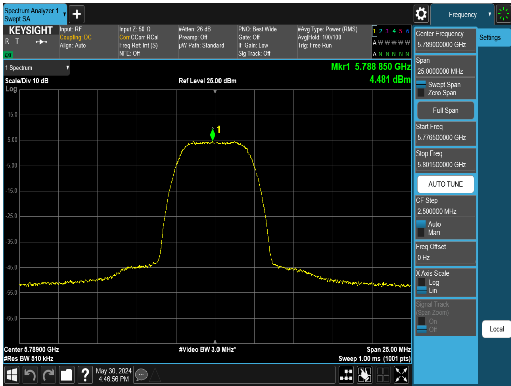
Plot 7-68. PSD Antenna WF5T (NB UNII HDR8, ePA - 5789MHz)
