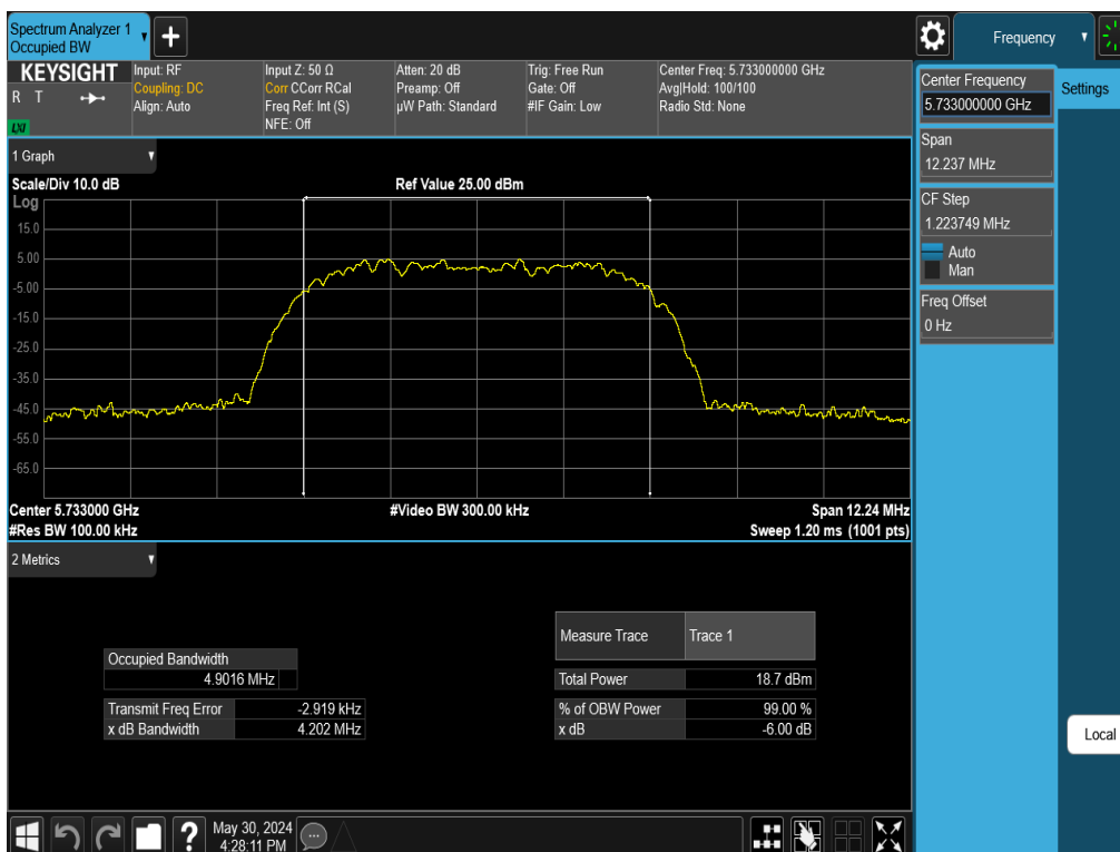
Plot 7-25. 6dB BW & 99% OBW Antenna WF5T (NB UNII HDR8, ePA – 5733MHz)
