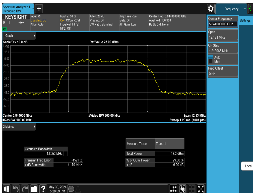
Plot 7-36. 6dB BW & 99% OBW Antenna WF2 (NB UNII HDR8, ePA – 5844MHz)
