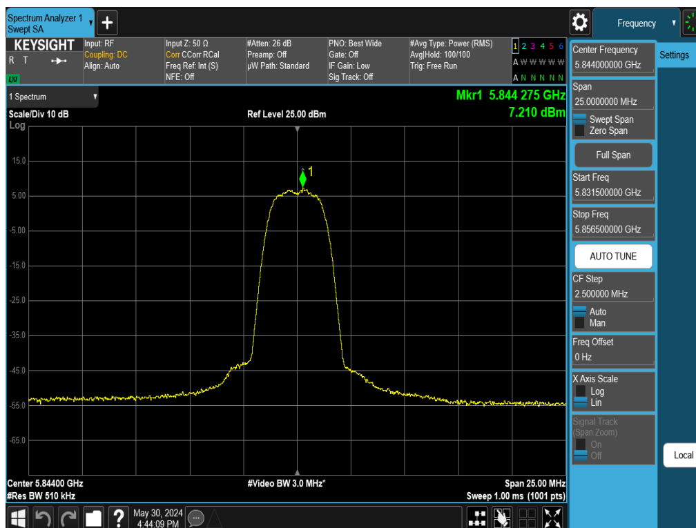
Plot 7-63. PSD Antenna WF5T (NB UNII HDR4, ePA – 5844MHz)
