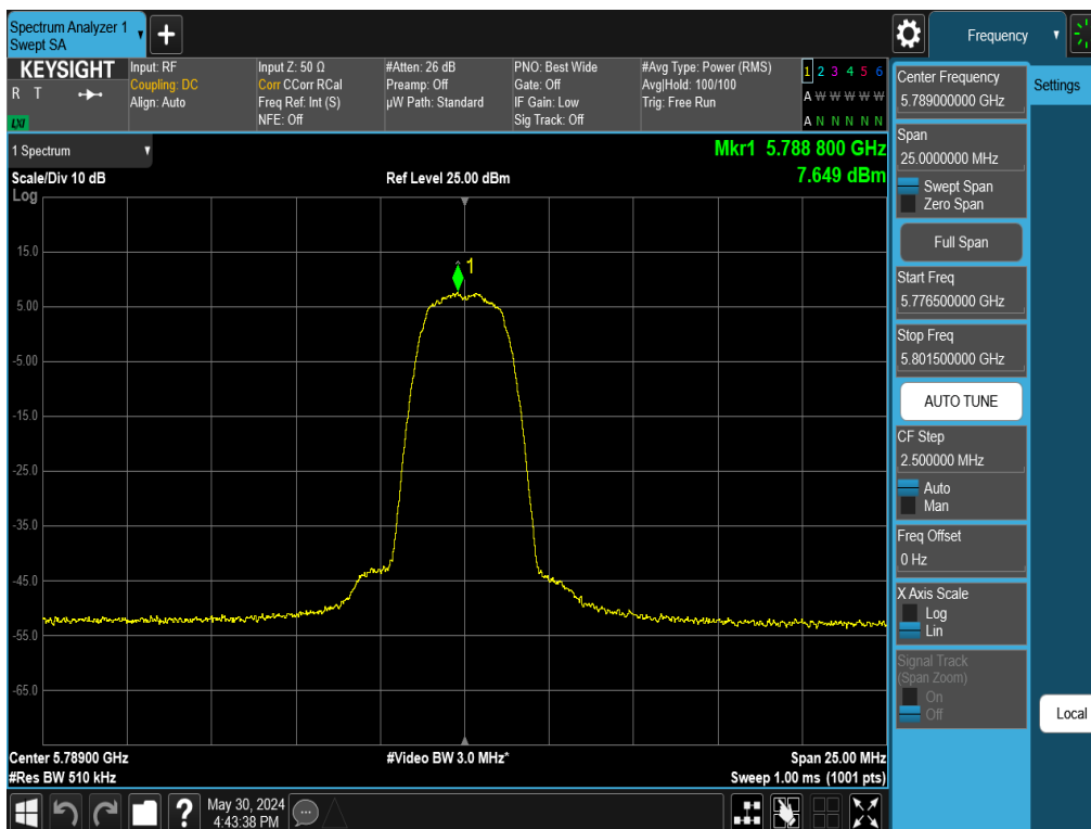
Plot 7-62. PSD Antenna WF5T (NB UNII HDR4, ePA – 5789MHz)
