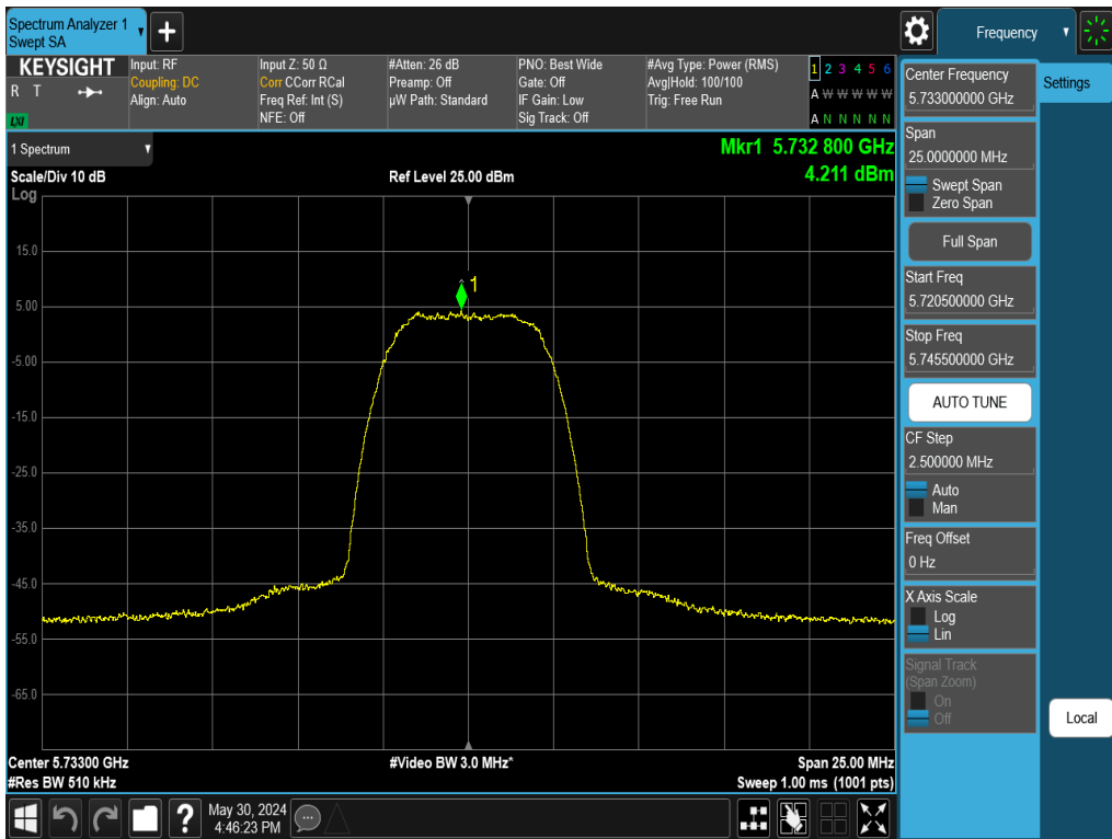
Plot 7-67. PSD Antenna WF5T (NB UNII HDR8, ePA - 5733MHz)
