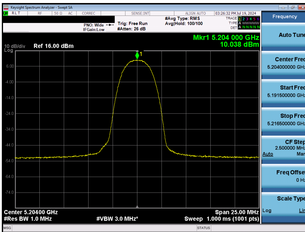
Plot 7-44. PSD Antenna WF5T (NB UNII HDR4, ePA – 5204MHz)
