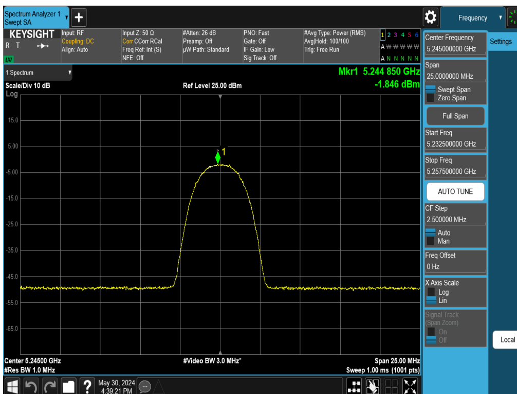
Plot 7-48. PSD Antenna WF5T (NB UNII HDR4, iPA– 5245MHz)
