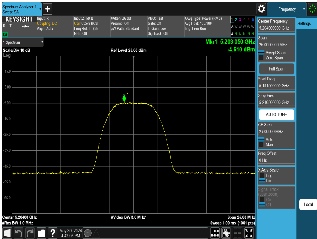
Plot 7-53. PSD Antenna WF5T (NB UNII HDR8, iPA – 5204MHz)
