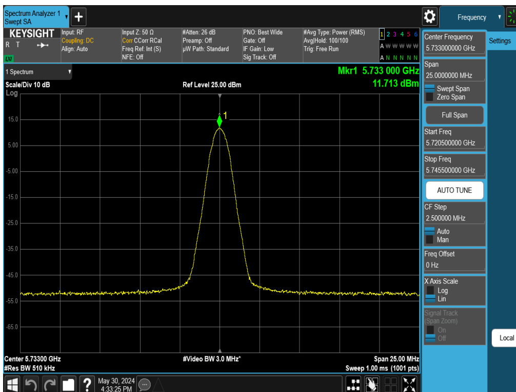
Plot 7-55. PSD Antenna WF5T (NB UNII BDR, ePA – 5733MHz)
