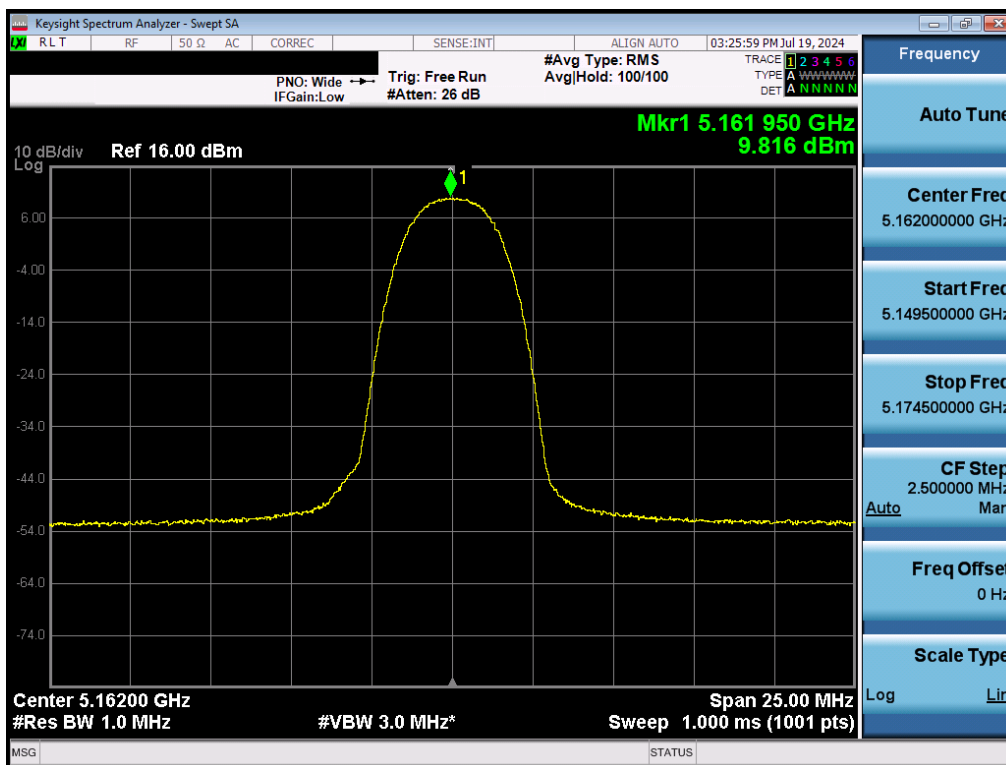
7-43. PSD Antenna WF5T (NB UNII HDR4, ePA – 5162MHz)
