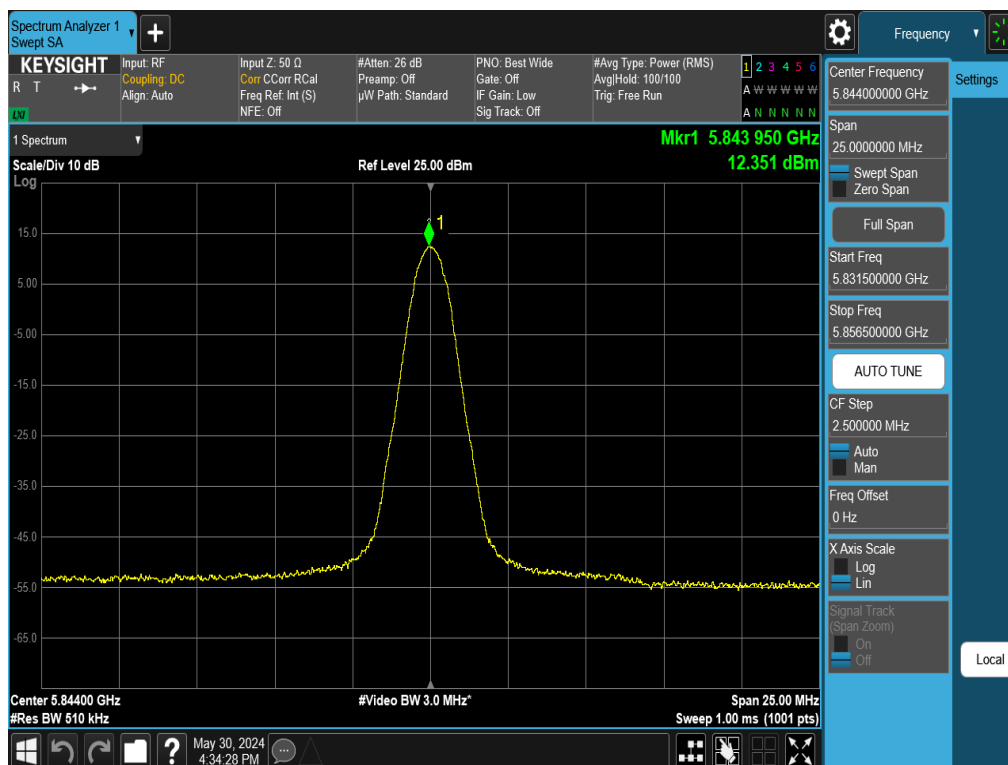
Plot 7-57. PSD Antenna WF5T (NB UNII BDR, ePA – 5844MHz)
