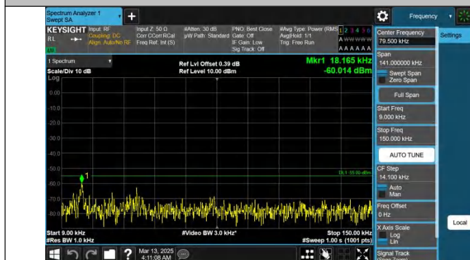
Band38-20MHz-QPSK-38000-1RB#0-0.009~0.15-PASS
