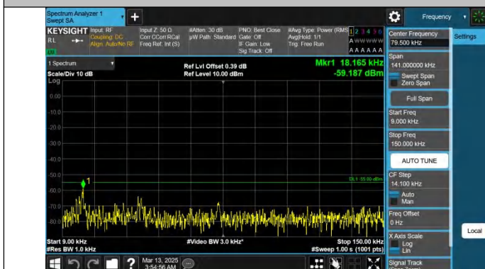
Band38-15MHz-QPSK-38000-1RB#0-0.009~0.15-PASS
