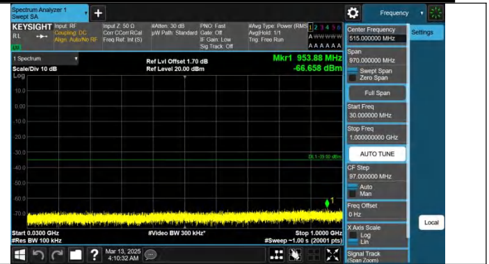
Band38-20MHz-QPSK-37850-1RB#99-30~1000-PASS
