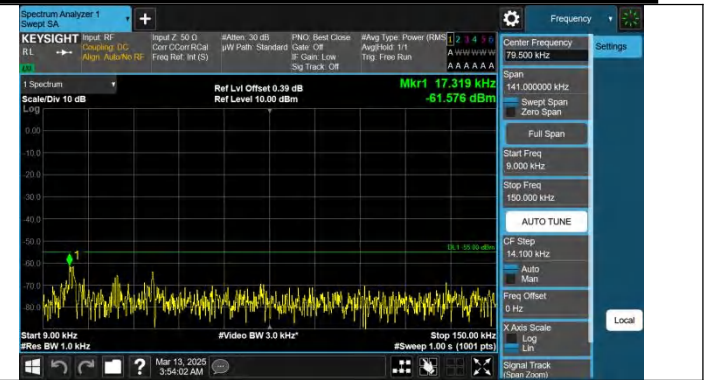
Band38-15MHz-QPSK-37825-1RB#74-0.009~0.15-PASS
