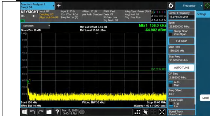
Band38-10MHz-QPSK-38200-1RB#49-0.15~30-PASS
