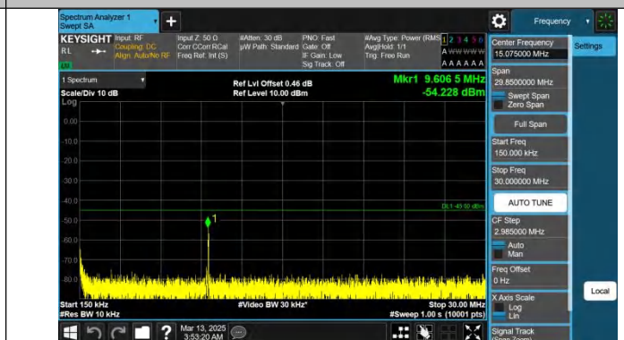
Band38-15MHz-QPSK-37825-1RB#0-0.15~30-PASS
