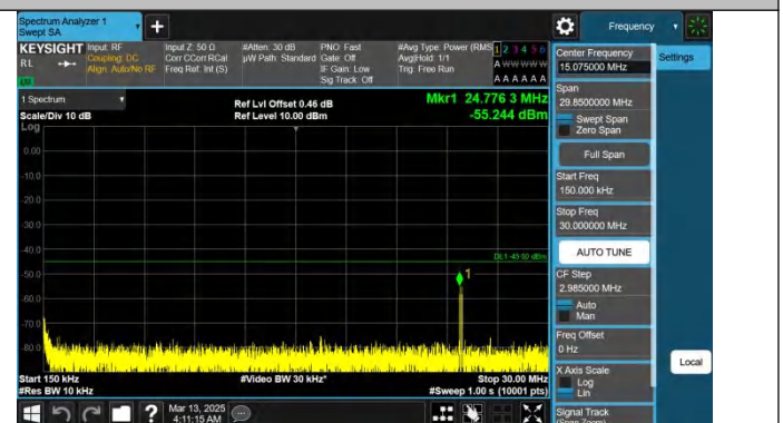
Band38-20MHz-QPSK-38000-1RB#0-0.15~30-PASS
