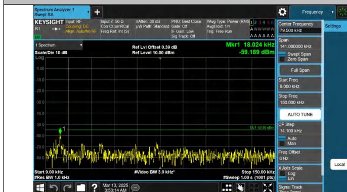
Band38-15MHz-QPSK-37825-1RB#0-0.009~0.15-PASS
