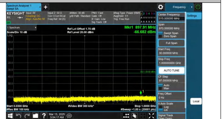
Band38-15MHz-QPSK-37825-1RB#74-30~1000-PASS
