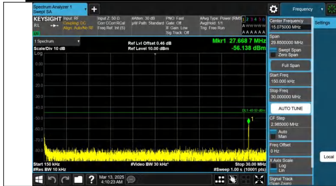
Band38-20MHz-QPSK-37850-1RB#99-0.15~30-PASS
