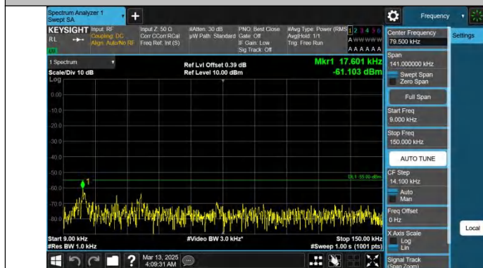
Band38-20MHz-QPSK-37850-1RB#0-0.009~0.15-PASS
