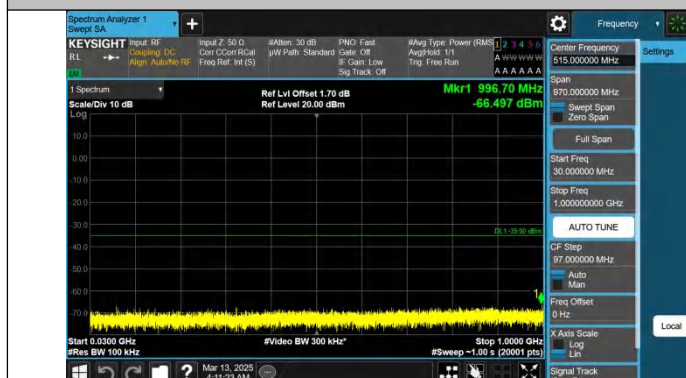
Band38-20MHz-QPSK-38000-1RB#0-30~1000-PASS
