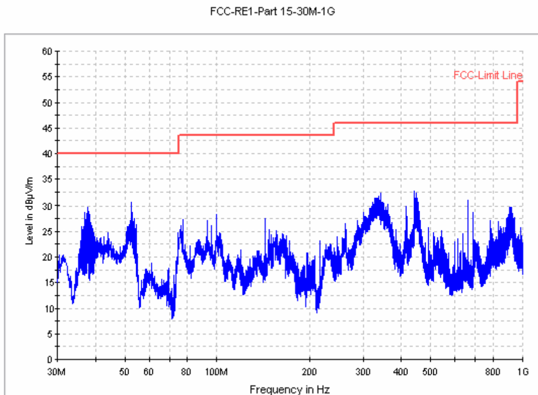
Figure A.5 Radiated Emission from 30MHz to 1GHz (Set.2, USB mode)
