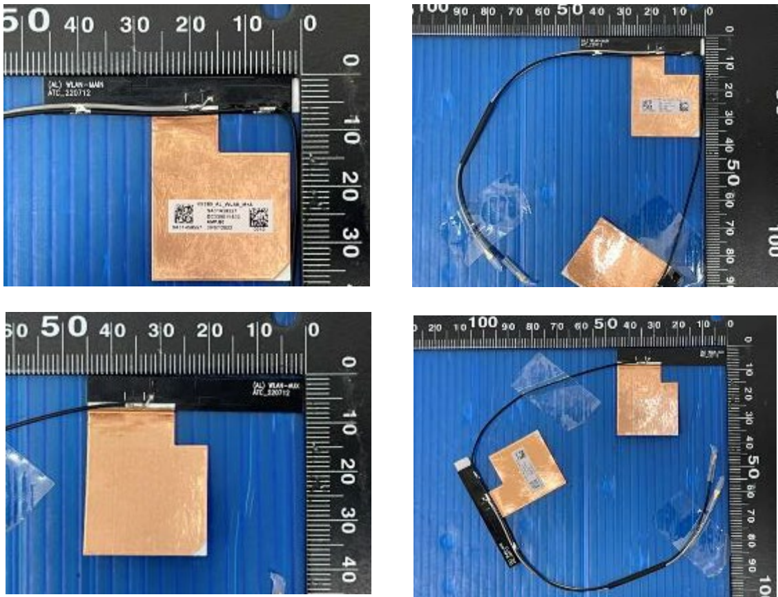
Main Antenna Photo (Front/Back):
