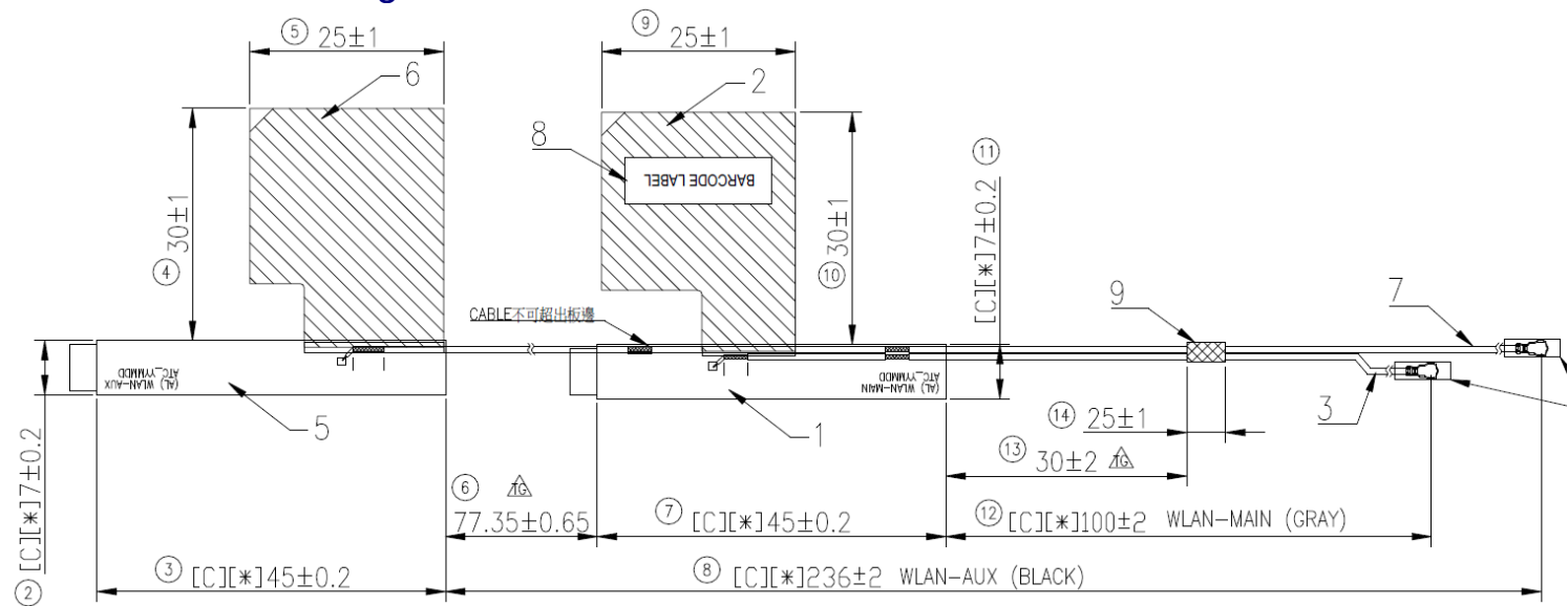
Main Antenna Drawing:
