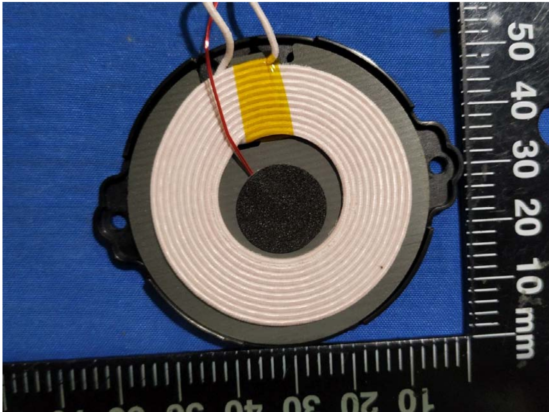
Wireless charger Coil Antenna
