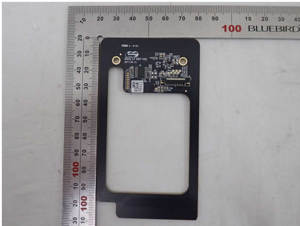
< 126.7 kHz Antenna Board - Back >
