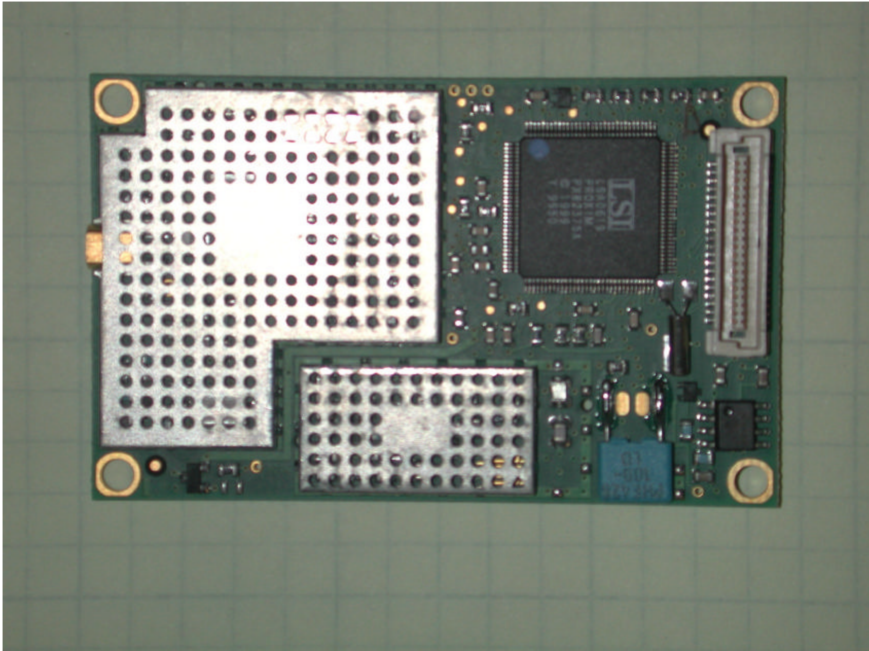
Bottom of Radio Board with Shields Installed
