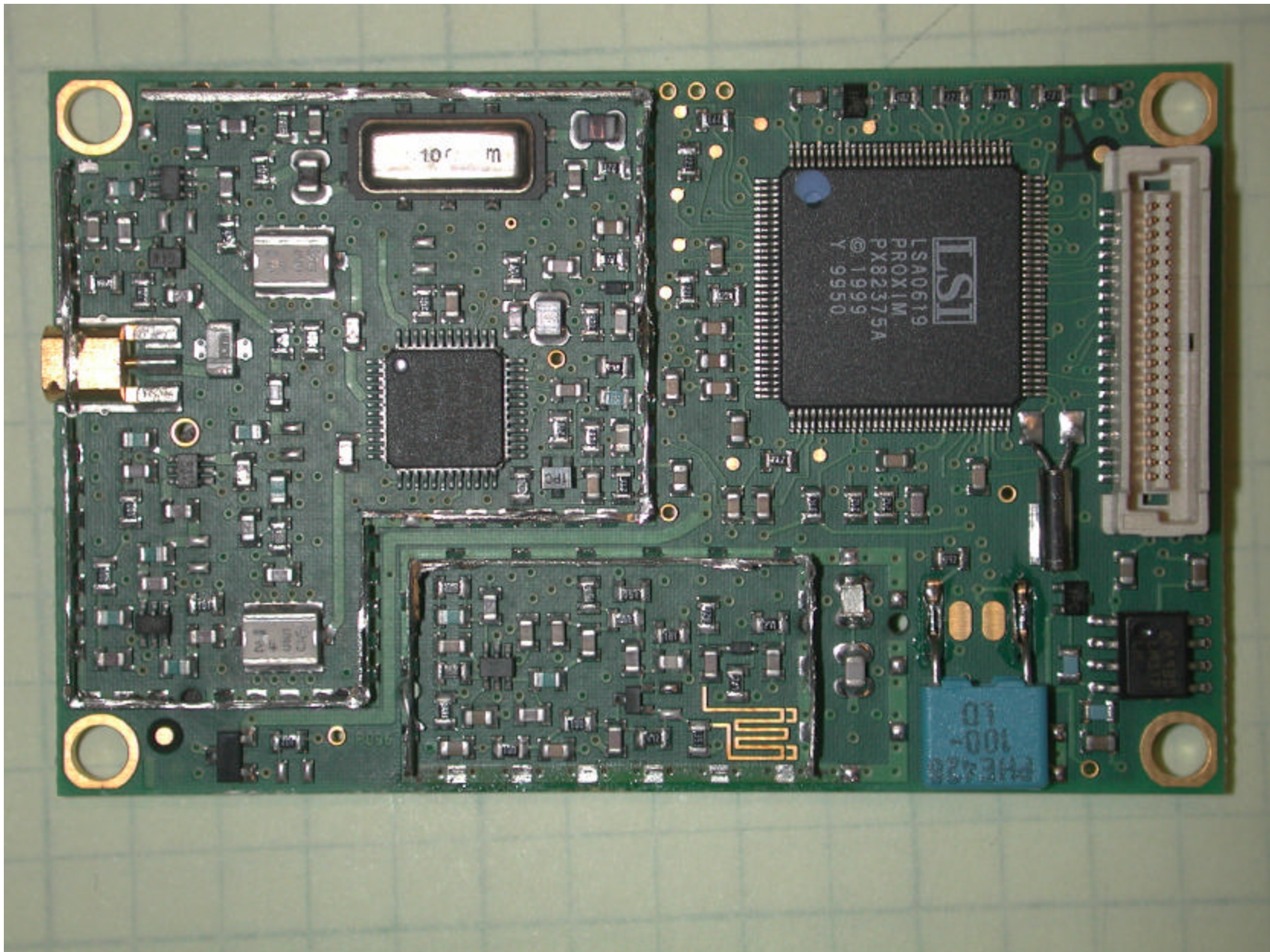
Bottom of Radio Board with Shields Removed
