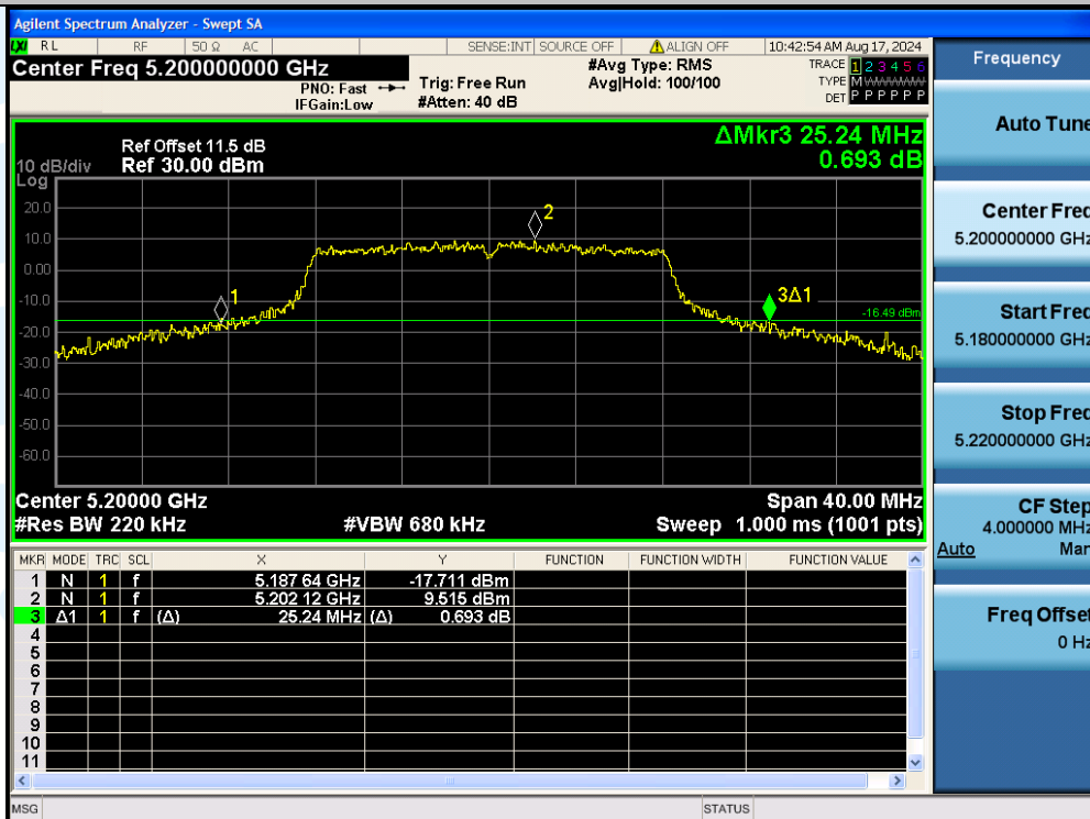
11A-Ant2-5200
