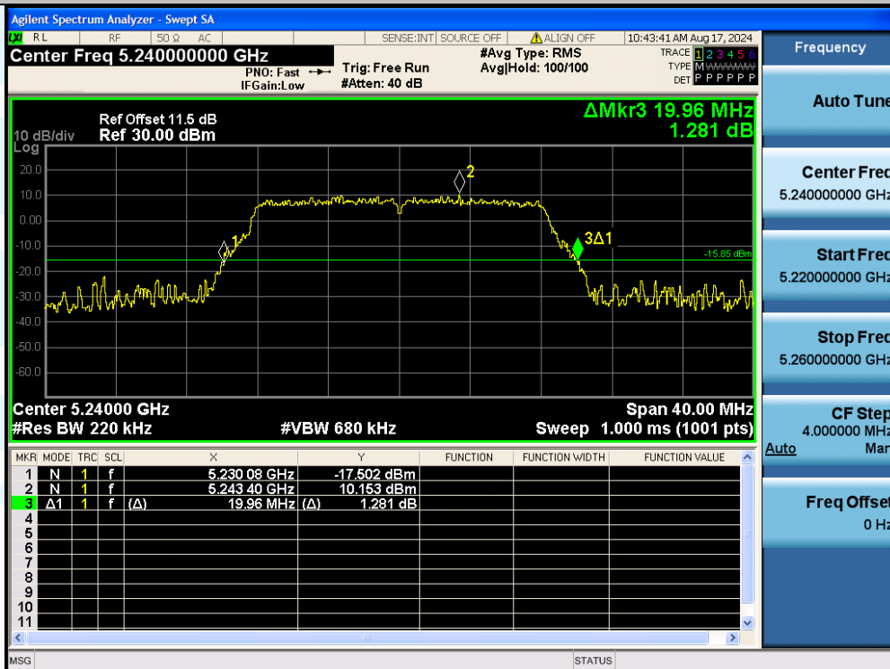
11A-Ant2-5240
