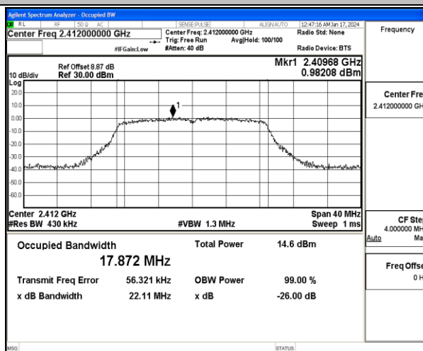
11N20MIMO-Ant2-2412
