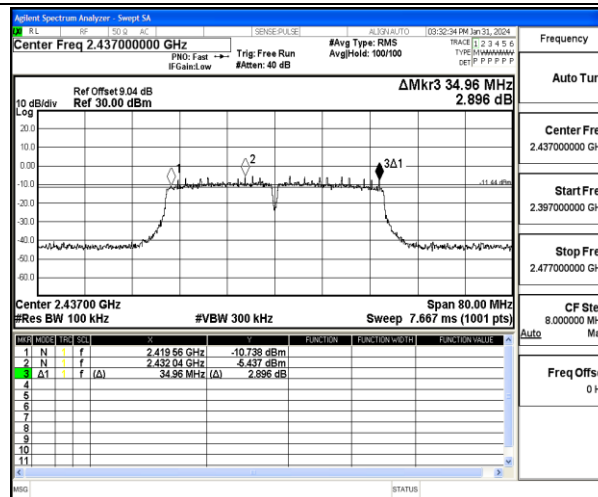
11N40MIMO-Ant2-2437-PASS
