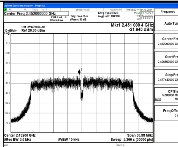
11N40MIMO-Ant1-2452-PASS
