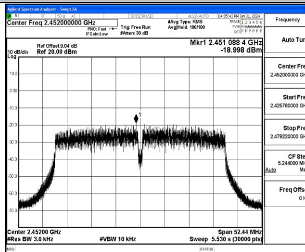
11N40MIMO-Ant2-2452-PASS
