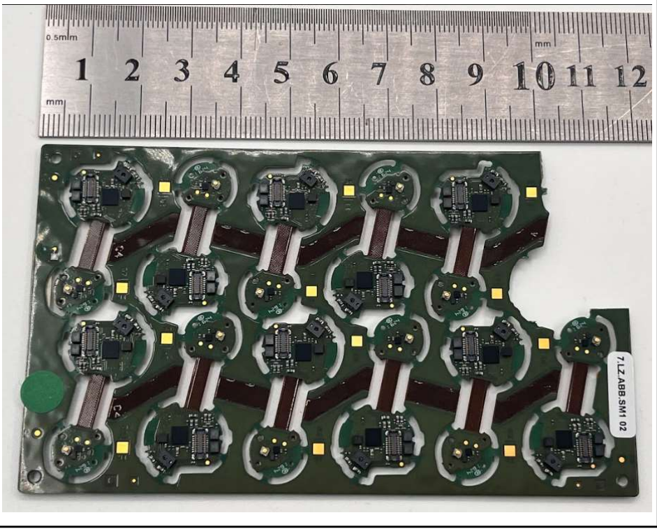
Right Mainboard Panel Bottom Side
