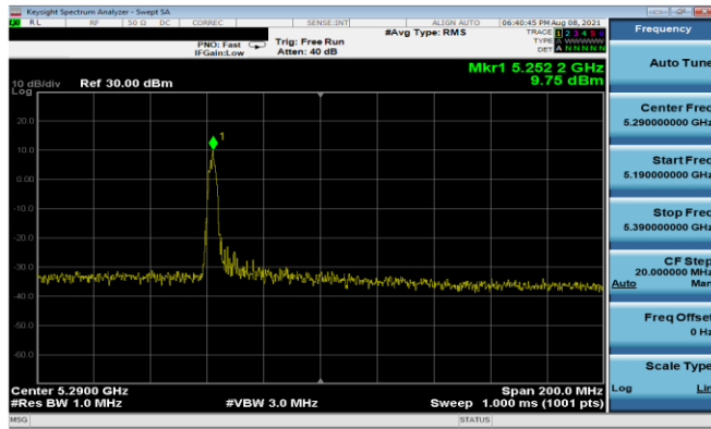
Plot 7-285. PSD Antenna 1b (80MHz BW 11ax Index 0 - RU26 - Ch.58)
