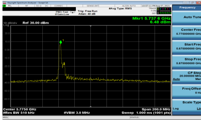
Plot 7-249. PSD Antenna 3b (80MHz BW 11ax Index 0 - RU26 - Ch.155)
