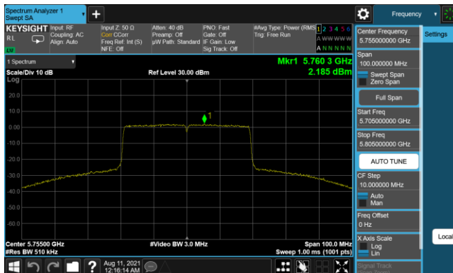
Plot 7-248. PSD Antenna 3b (40MHz BW 11ax - RU484 - Ch.151)
