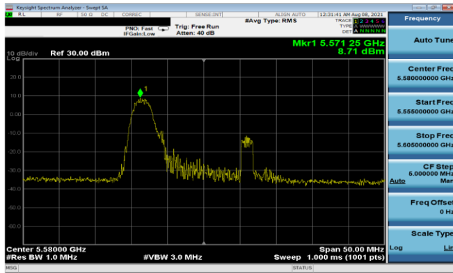
Plot 7-289. PSD Antenna 1b (20MHz BW 11ax Index 0 - RU26 - Ch.116)
