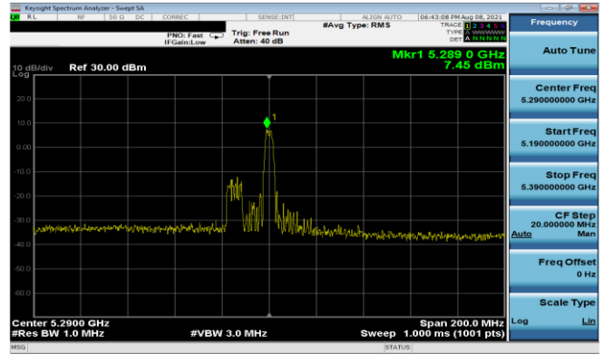
Plot 7-286. PSD Antenna 1b (80MHz BW 11ax Index 18 - RU26 - Ch.58)
