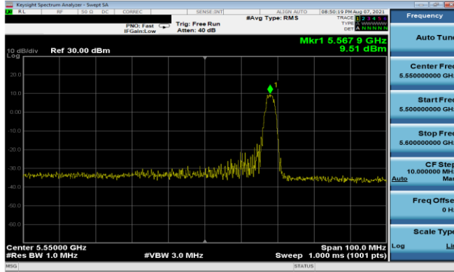
Plot 7-235. PSD Antenna 3b (40MHz BW 11ax Index 17 – RU26 – Ch.110)
