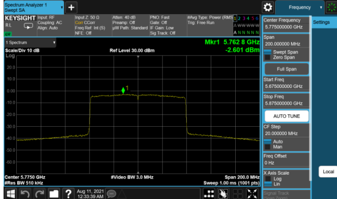
Plot 7-252. PSD Antenna 3b (80MHz BW 11ax - RU996 - Ch.155)
