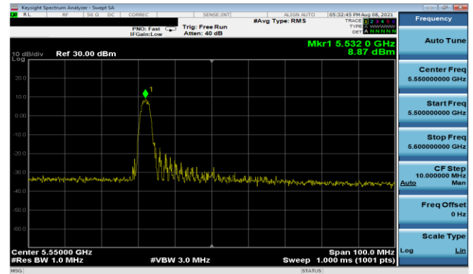
Plot 7-293. PSD Antenna 1b (40MHz BW 11ax Index 0 - RU26 - Ch.110)
