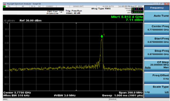
Plot 7-251. PSD Antenna 3b (80MHz BW 11ax Index 36 - RU26 - Ch.155)
