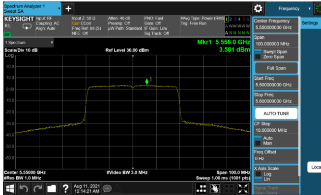
Plot 7-236. PSD Antenna 3b (40MHz BW 11ax – RU484 – Ch.110)
