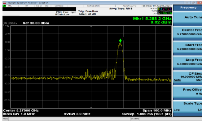
Plot 7-283. PSD Antenna 1b (40MHz BW 11ax Index 17 - RU26 - Ch.54)
