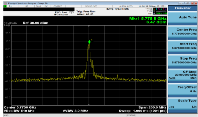
Plot 7-250. PSD Antenna 3b (80MHz BW 11ax Index 18 - RU26 - Ch.155)
