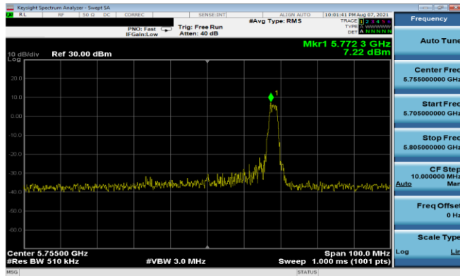
Plot 7-247. PSD Antenna 3b (40MHz BW 11ax Index 17 - RU26 - Ch.151)
