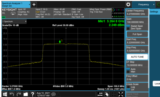
Plot 7-284. PSD Antenna 1b (40MHz BW 11ax - RU484 - Ch.54)
