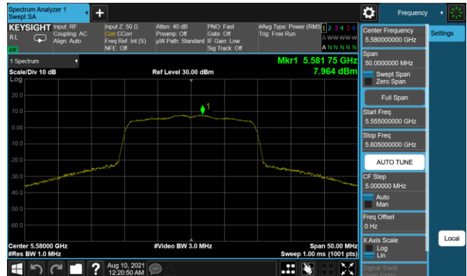
Plot 7-292. PSD Antenna 1b (20MHz BW 11ax - RU242 - Ch.116)
