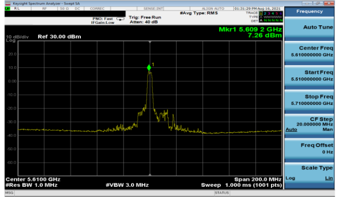
Plot 7-238. PSD Antenna 3b (80MHz BW 11ax Index 18 – RU26 – Ch.122)
