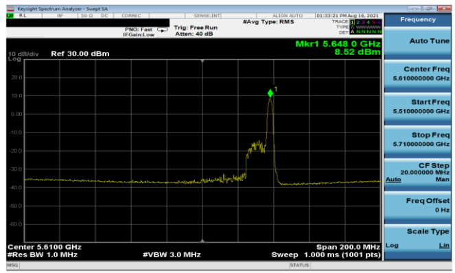
Plot 7-239. PSD Antenna 3b (80MHz BW 11ax Index 36 – RU26 – Ch.122)
