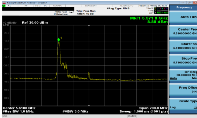
Plot 7-237. PSD Antenna 3b (80MHz BW 11ax Index 0 – RU26 – Ch.122)
