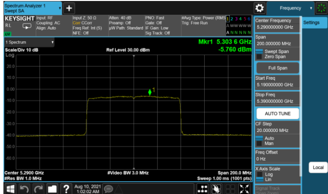
Plot 7-288. PSD Antenna 1b (80MHz BW 11ax - RU996 - Ch.58)
