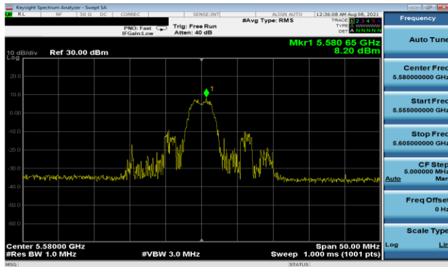
Plot 7-290. PSD Antenna 1b (20MHz BW 11ax Index 4 - RU26 - Ch.116)
