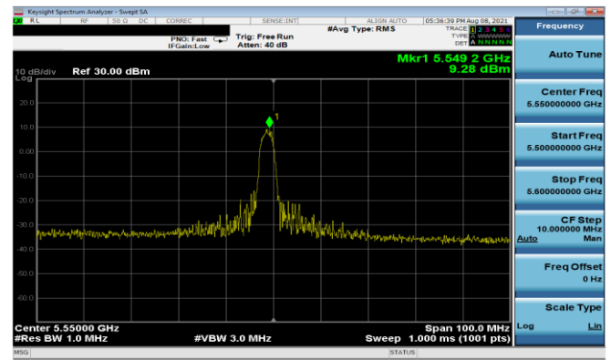
Plot 7-294. PSD Antenna 1b (40MHz BW 11ax Index 8 - RU26 - Ch.110)
