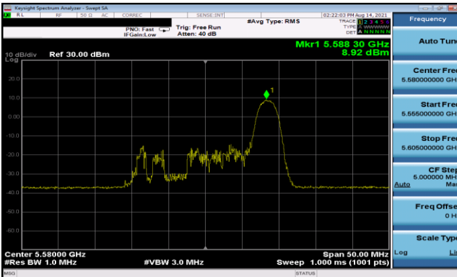
Plot 7-291. PSD Antenna 1b (20MHz BW 11ax Index 8 - RU26 - Ch.116)
