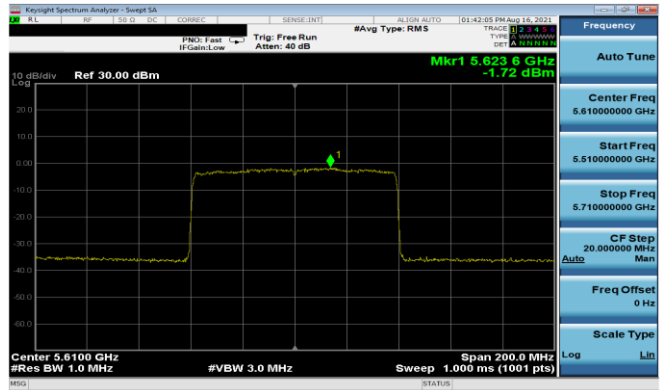
Plot 7-240. PSD Antenna 3b (80MHz BW 11ax – RU996 – Ch.122)
