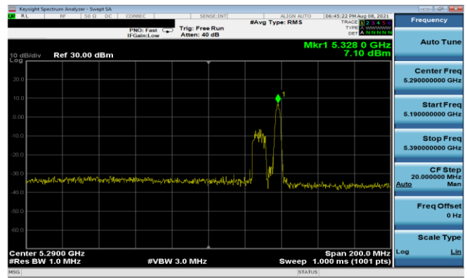
Plot 7-287. PSD Antenna 1b (80MHz BW 11ax Index 36 - RU26 - Ch.58)
