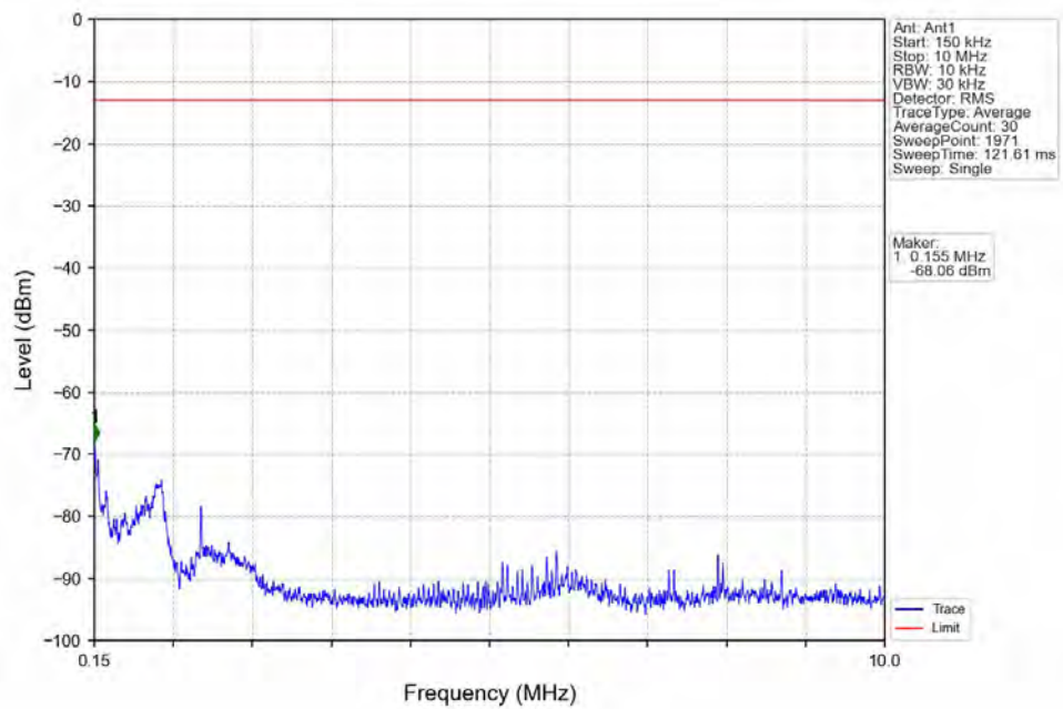
Band4_10MHz_16QAM_LCH_1715MHz_RB_1_0_NTNV
