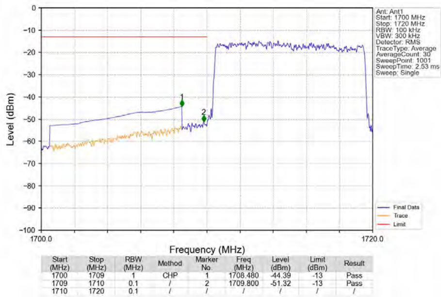
Band4_10MHz_16QAM_LCH_1715MHz_RB_50_0_NTNV
