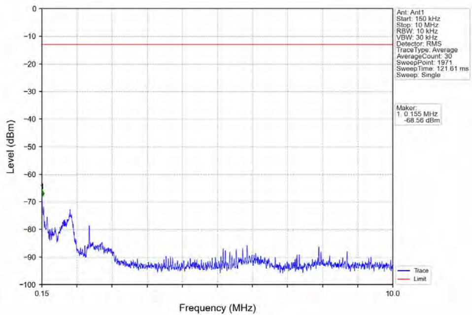
Band4_10MHz_16QAM_MCH_1732.5MHz_RB_1_0_NTNV
