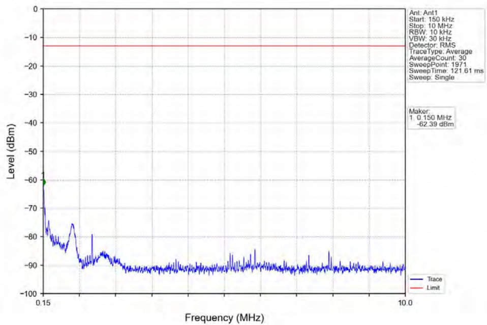
Band4_20MHz_16QAM_MCH_1732.5MHz_RB_1_0_NTNV
