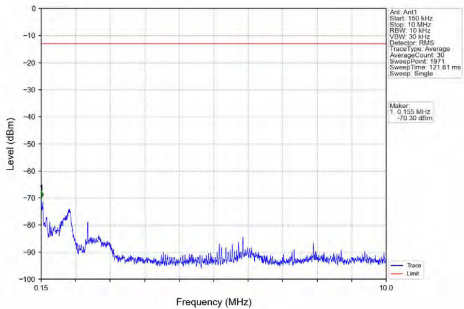
Band4_5MHz_16QAM_MCH_1732.5MHz_RB_1_0_NTNV
