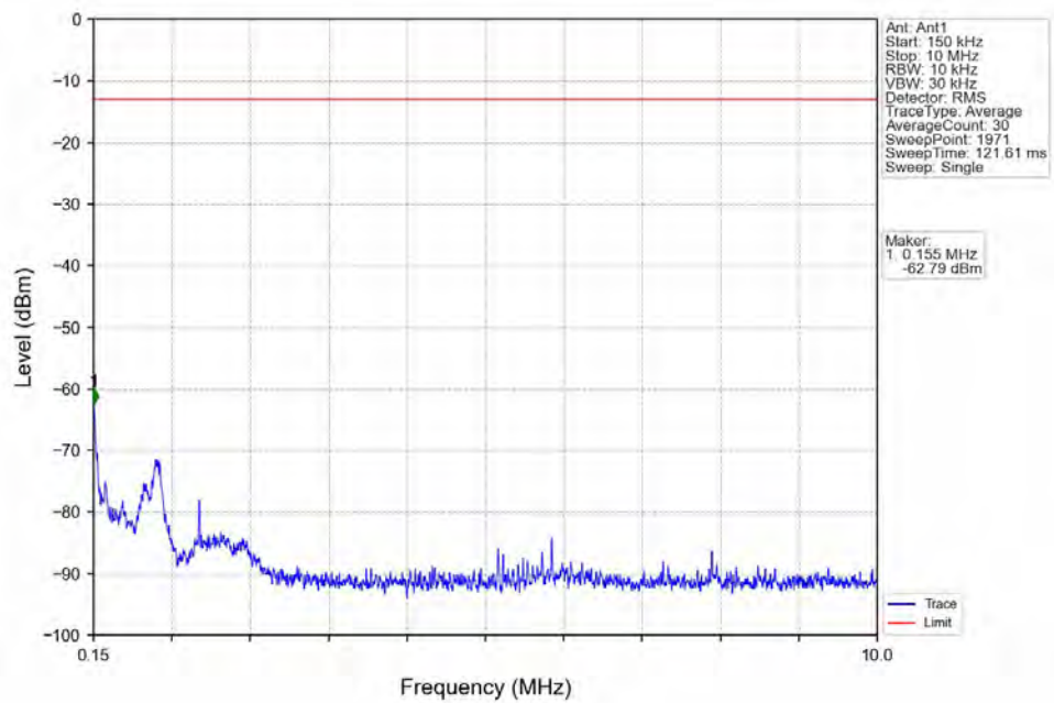
Band4_15MHz_16QAM_MCH_1732.5MHz_RB_1_0_NTNV
