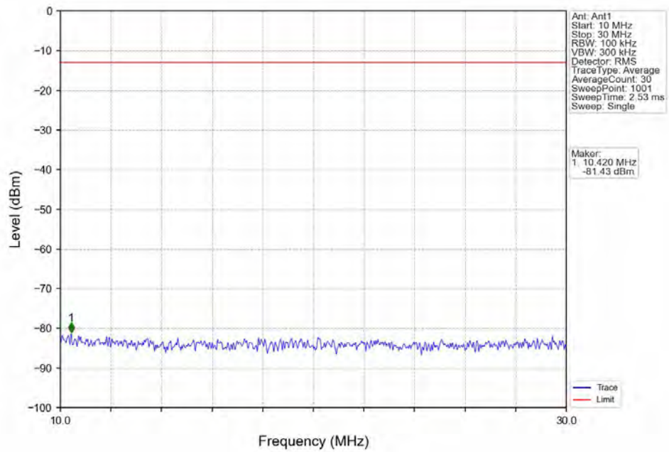
Band4_10MHz_16QAM_LCH_1715MHz_RB_1_0_NTNV
