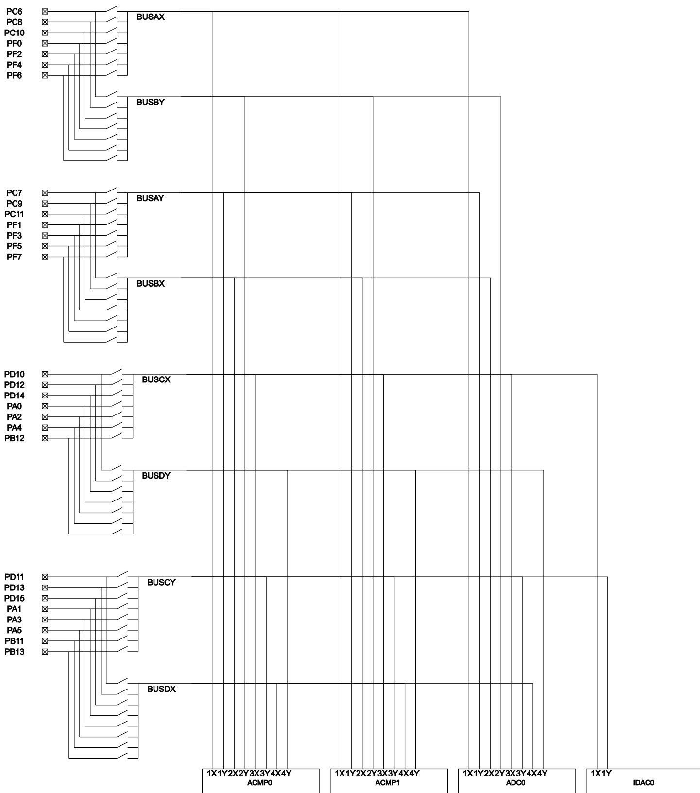
Figure 7.2. BGM121/BGM123 APORT
