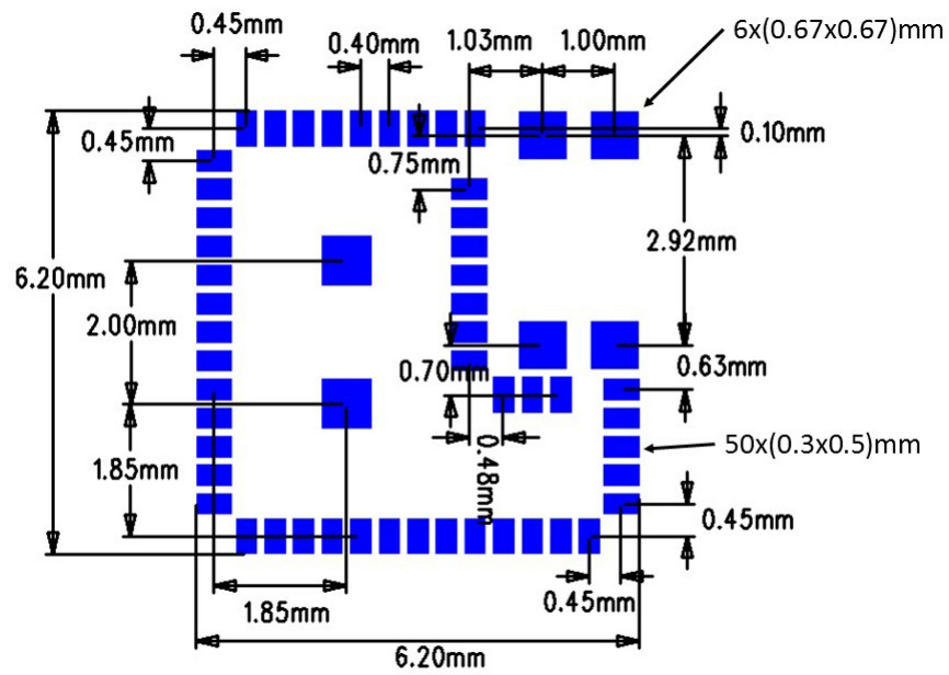
Figure 8.2. BGM121/BGM123 Dimensions and Footprint
