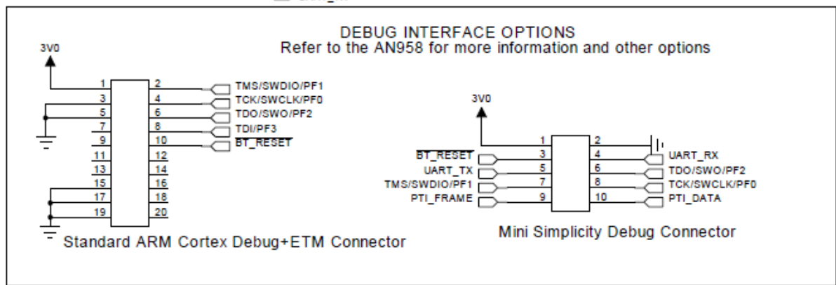
Figure 5.1. BGM121/BGM123 Connected to a Host CPU with Typical Power Supply, Ground and Debug connections
