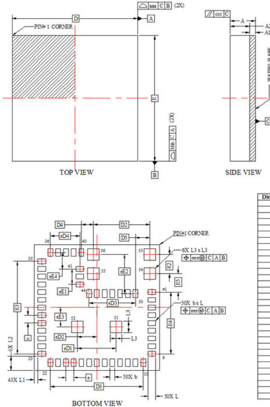
Figure 8.1. BGM121/BGM123 Package Dimensions
