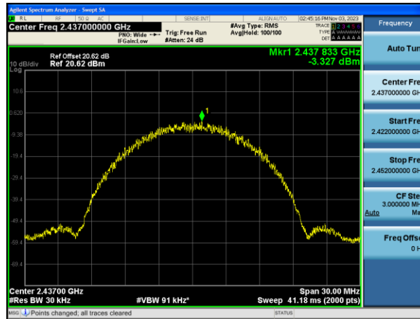
Power Spectral Density (802.11g-CH 6)
