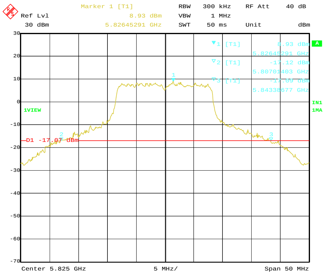
Date: 24.JAN.2005 17:42:12 Plot 1-7a. 26dB Bandwidth of 5825MHz (OFDM, 24Mbps)
