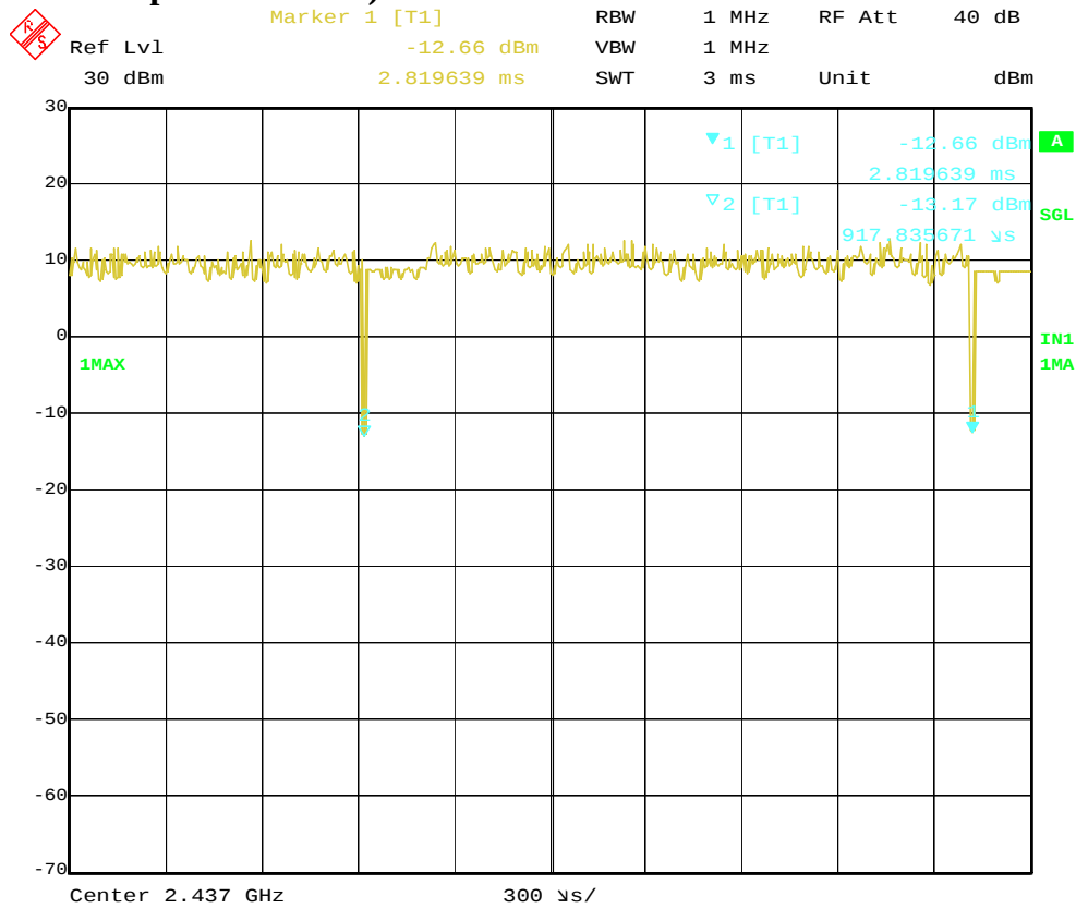
Date: 18.JAN.2005 14:23:01 Plot 1-0 Transmission Pulse Duration of DSSS Tx mode
