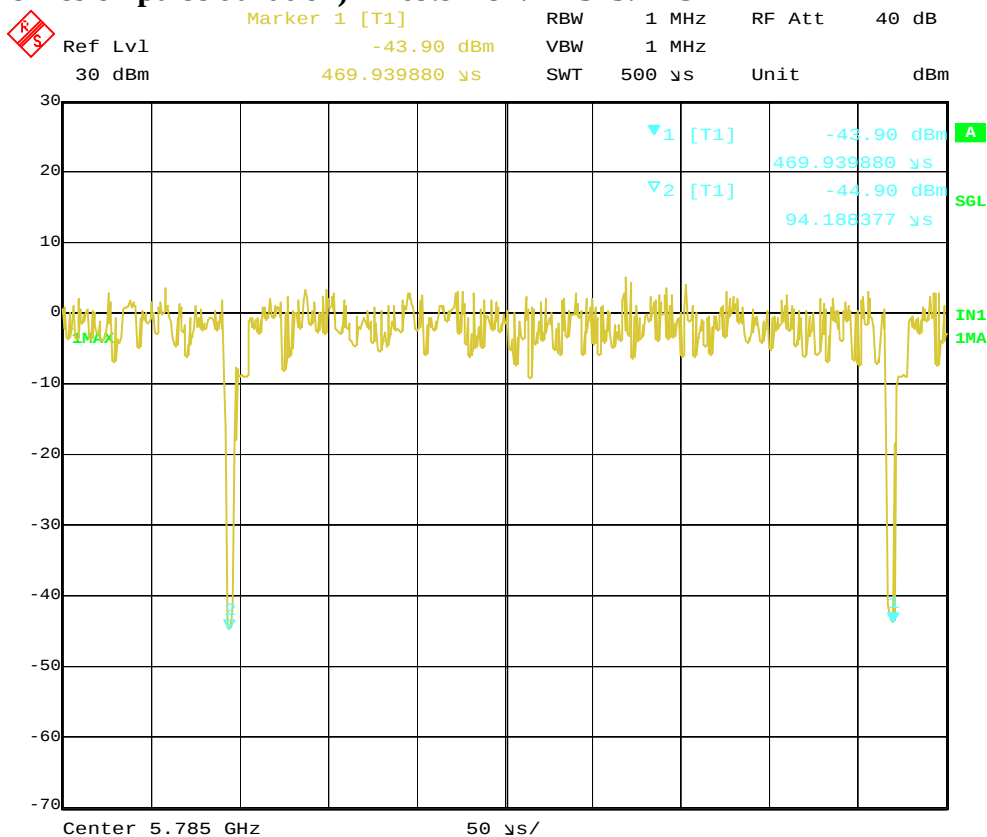
Date: 24.JAN.2005 13:32:24 Plot 1-1 Transmission Pulse Duration of QEDM Tx mode
