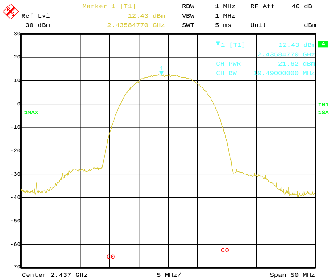
Date: 18.JAN.2005 15:58:53 Plot 1-2b. Conducted Peak Output Power of 2437MHz (DSSS, 11Mbps, peak power )
