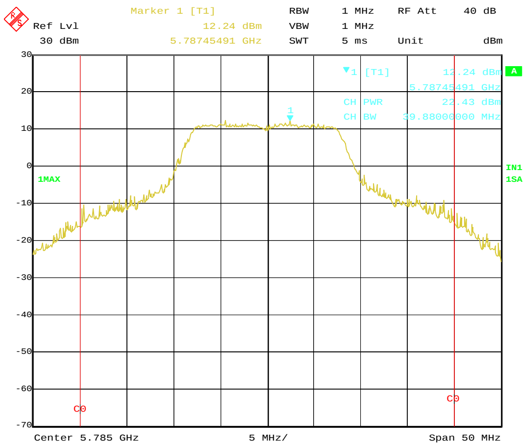
Date: 24.JAN.2005 18:51:27 Plot 1-4b. Conducted Peak Output Power of 5785MHz (OFDM, 6Mbps peak power)
