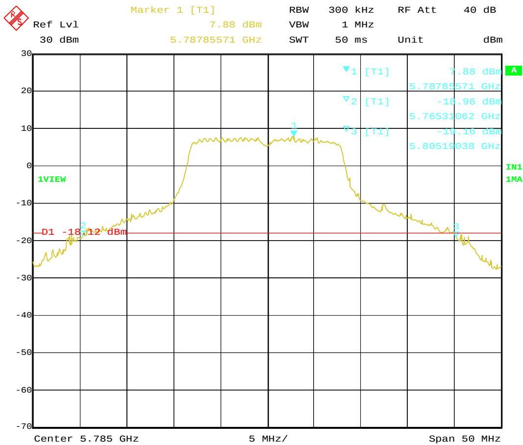
Date: 24.JAN.2005 14:45:21 Plot 1-4a. 26dB Bandwidth of 5785MHz (OFDM, 6Mbps)
