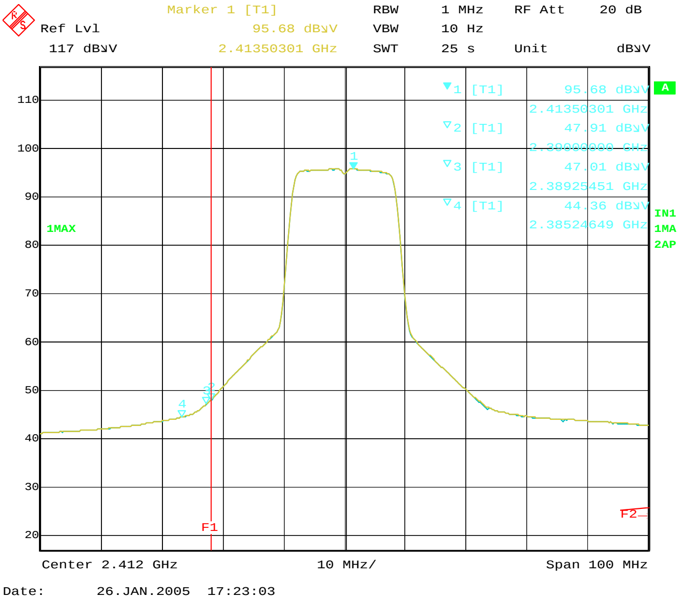
Plot 2-4 Ch.1 2412MHz TX, OFDM 24Mbps (Average) in tablet operation mode
