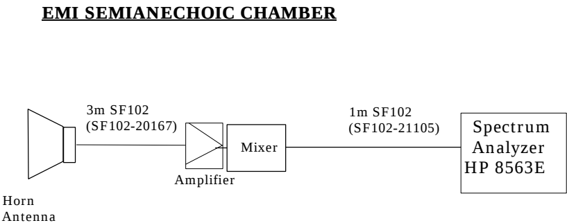
Figure 2-4. Cables for Radiated Emission Test (26.5 – 40GHz)
