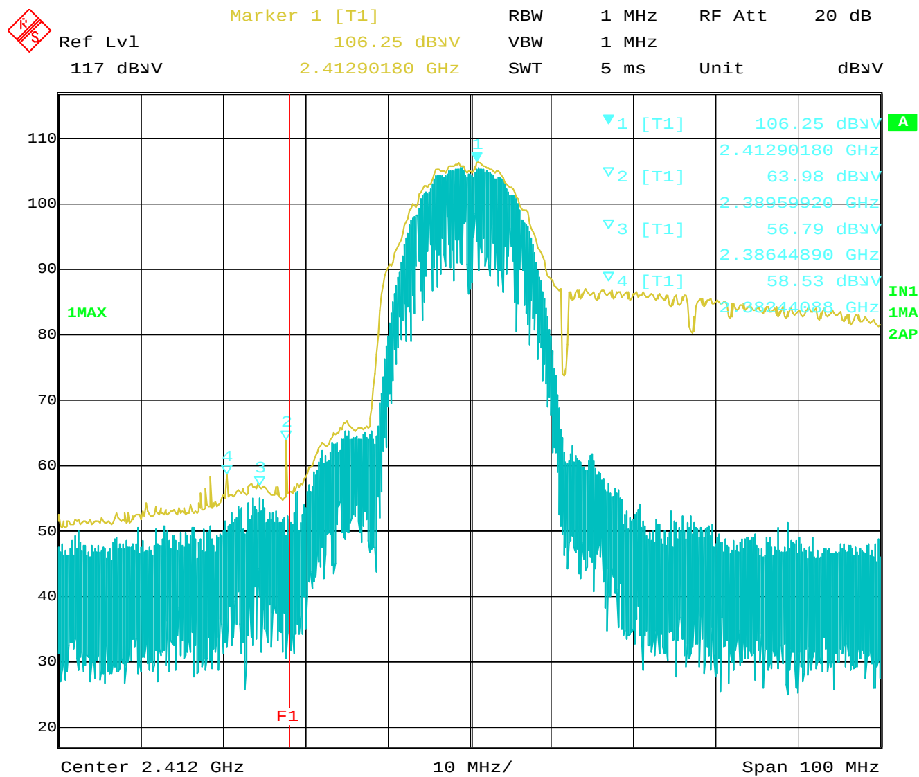
Plot-2-1 Ch.1 2412MHz TX, DSSS 1Mbps (Peak) in normal operation mode
