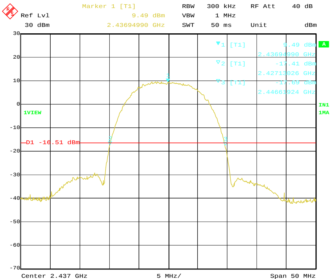
Date: 18.JAN.2005 15:01:54 Plot 1-2a. 26dB Bandwidth of 2437MHz (DSSS, 11Mbps)
