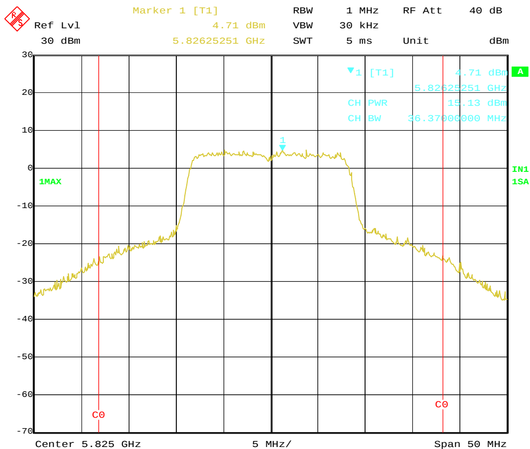
Date: 24.JAN.2005 20:30:22 Plot 1-7b. Conducted Peak Output Power of 5825MHz (OFDM, 24Mbps, mean power)
