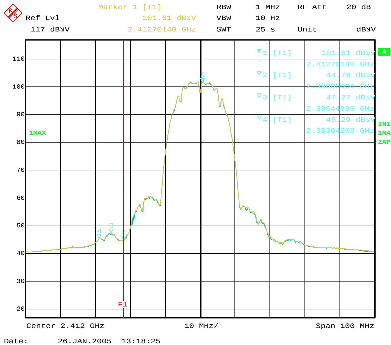
Plot 2-2 Ch.1 2412MHz TX, DSSS 1Mbps (Average) in normal operation mode
