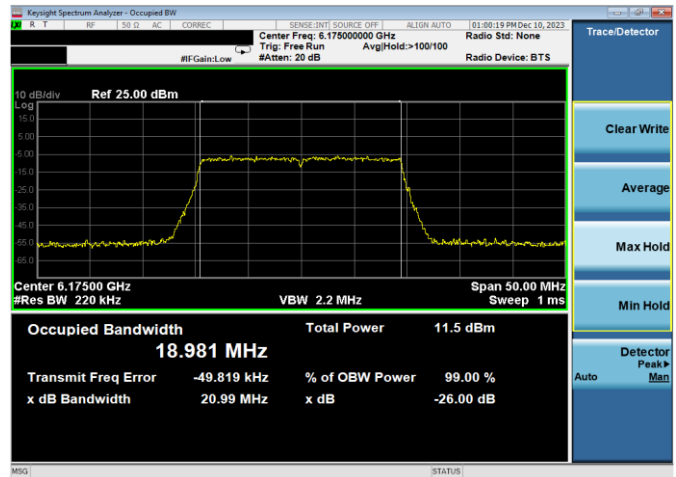
Plot 7-4. 26dB & 99% Bandwidth Plot Antenna WF7a (20MHz 802.11ax RU242 (UNII Band 5) - Ch. 45)
