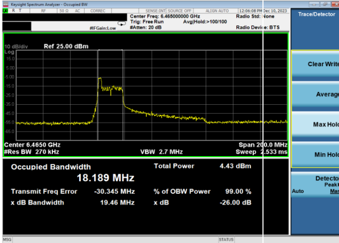
Plot 7-25. 26dB & 99% Bandwidth Plot Antenna WF7a (80MHz 802.11ax RU26 (UNII Band 6) - Ch. 103)
