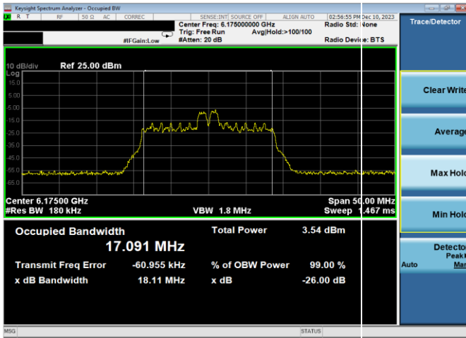
Plot 7-66. 26dB & 99% Bandwidth Plot Antenna WF2a (20MHz 802.11ax RU26 (UNII Band 5) – Ch. 45)
