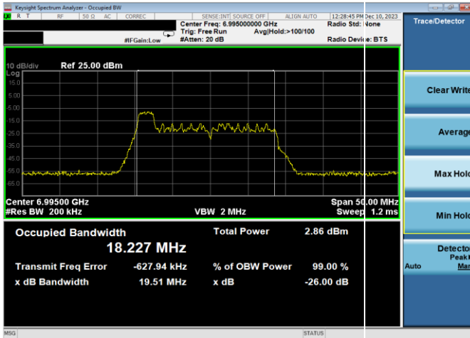
Plot 7-49. 26dB & 99% Bandwidth Plot Antenna WF7a (20MHz 802.11ax RU26 (UNII Band 8) - Ch. 209)
