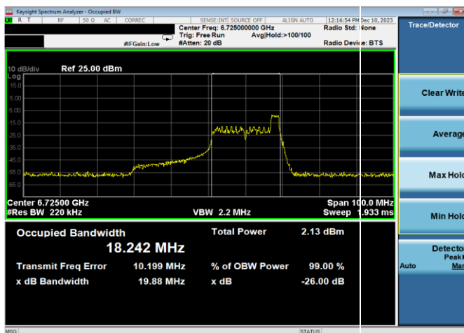
Plot 7-39. 26dB & 99% Bandwidth Plot Antenna WF7a (40MHz 802.11ax RU26 (UNII Band 7) – Ch. 155)
