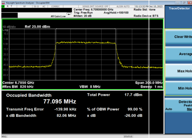
Plot 7-44. 26dB & 99% Bandwidth Plot Antenna WF7a (80MHz 802.11ax RU996 (UNII Band 7) - Ch. 151)
