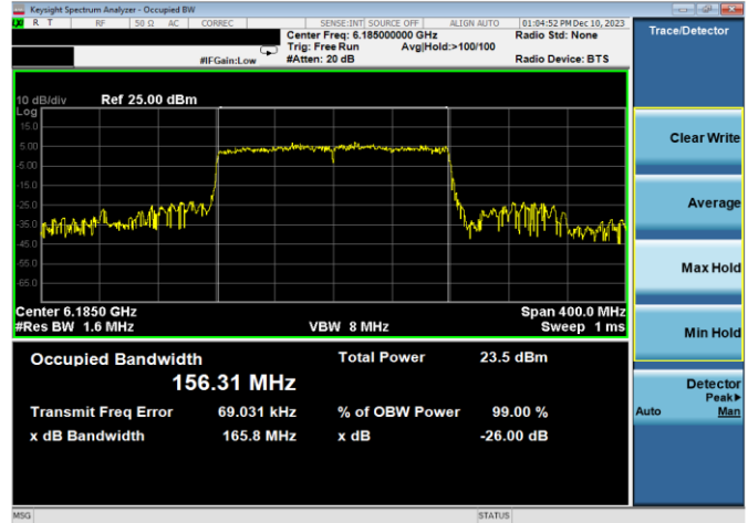
Plot 7-16. 26dB & 99% Bandwidth Plot Antenna WF7a (160MHz 802.11ax RU996x2 (UNII Band 5) - Ch. 47)
