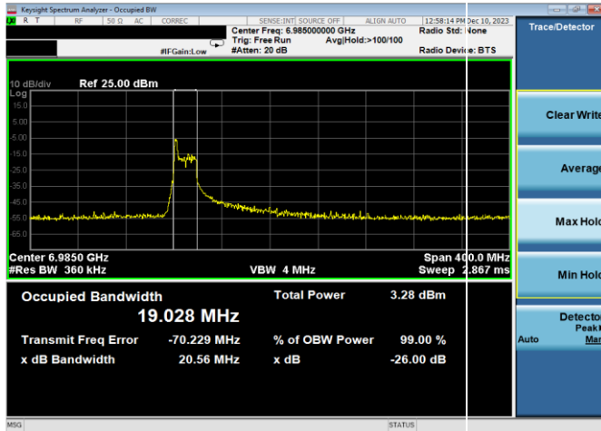
Plot 7-61. 26dB & 99% Bandwidth Plot Antenna WF7a (160MHz 802.11ax RU26 (UNII Band 8) – Ch. 207)
