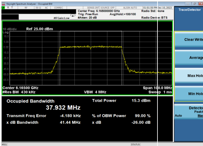
Plot 7-8. 26dB & 99% Bandwidth Plot Antenna WF7a (40MHz 802.11ax RU484 (UNII Band 5) – Ch. 43)
