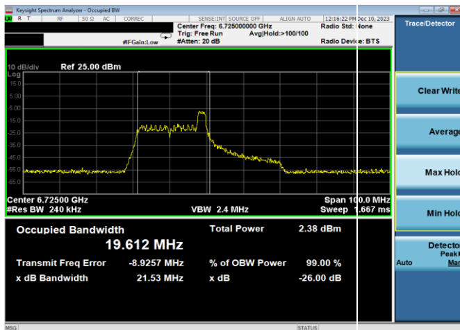
Plot 7-38. 26dB & 99% Bandwidth Plot Antenna WF7a (40MHz 802.11ax RU26 (UNII Band 7) – Ch. 155)
