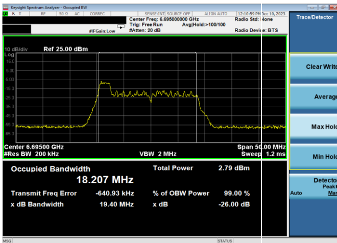
Plot 7-33. 26dB & 99% Bandwidth Plot Antenna WF7a (20MHz 802.11ax RU26 (UNII Band 7) – Ch. 149)
