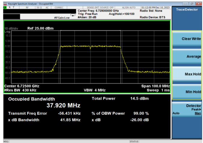
Plot 7-40. 26dB & 99% Bandwidth Plot Antenna WF7a (40MHz 802.11ax RU484 (UNII Band 7) – Ch. 155)
