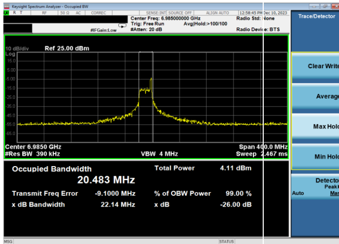
Plot 7-62. 26dB & 99% Bandwidth Plot Antenna WF7a (160MHz 802.11ax RU26 (UNII Band 8) – Ch. 207)
