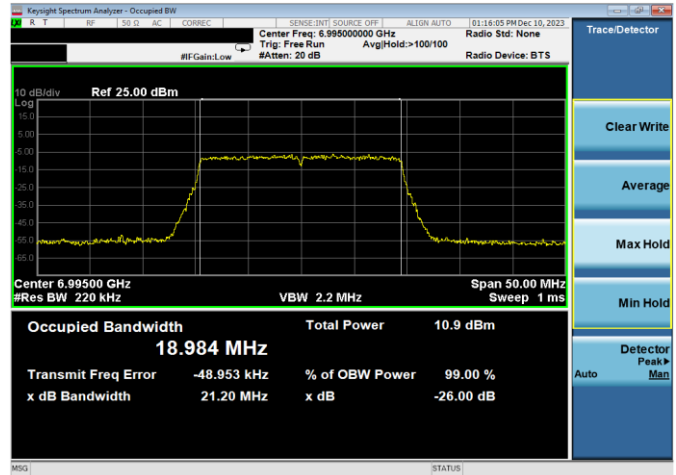
Plot 7-52. 26dB & 99% Bandwidth Plot Antenna WF7a (20MHz 802.11ax RU242 (UNII Band 8) - Ch. 209)
