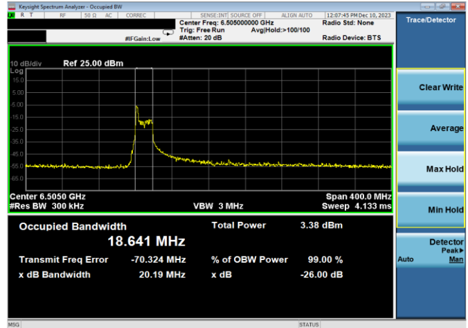
Plot 7-29. 26dB & 99% Bandwidth Plot Antenna WF7a (160MHz 802.11ax RU26 (UNII Band 6) - Ch. 111)
