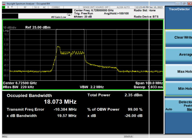
Plot 7-37. 26dB & 99% Bandwidth Plot Antenna WF7a (40MHz 802.11ax RU26 (UNII Band 7) – Ch. 155)
