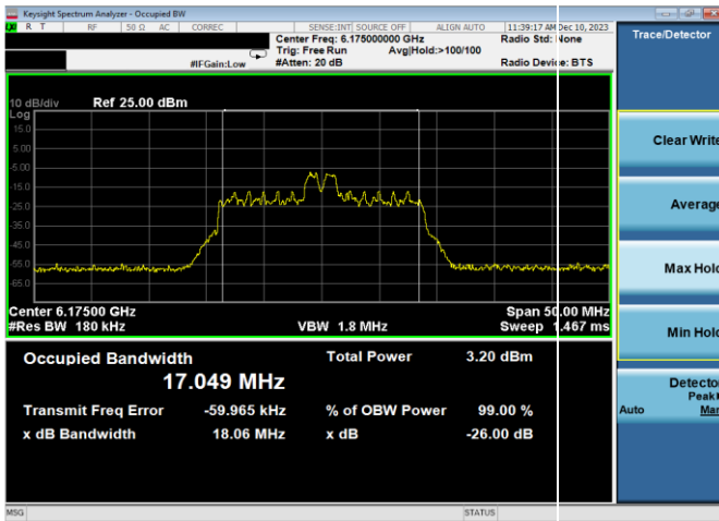
Plot 7-2. 26dB & 99% Bandwidth Plot Antenna WF7a (20MHz 802.11ax RU26 (UNII Band 5) - Ch. 45)
