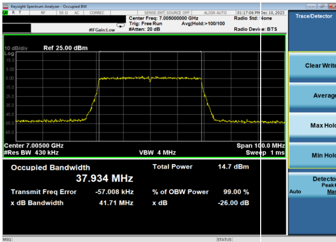
Plot 7-56. 26dB & 99% Bandwidth Plot Antenna WF7a (40MHz 802.11ax RU484 (UNII Band 8) - Ch. 211)
