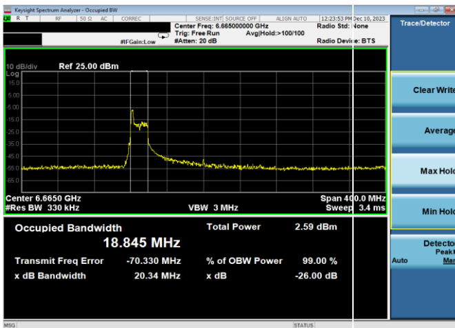
Plot 7-45. 26dB & 99% Bandwidth Plot Antenna WF7a (160MHz 802.11ax RU26 (UNII Band 7) - Ch. 143)
