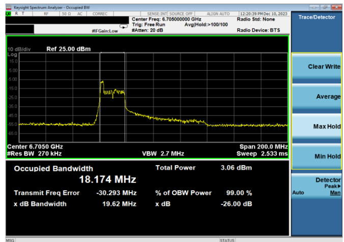
Plot 7-41. 26dB & 99% Bandwidth Plot Antenna WF7a (80MHz 802.11ax RU26 (UNII Band 7) – Ch. 151)
