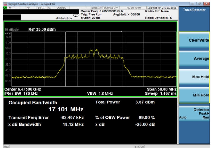
Plot 7-18. 26dB & 99% Bandwidth Plot Antenna WF7a (20MHz 802.11ax RU26 (UNII Band 6) - Ch. 105)
