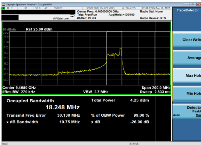
Plot 7-27. 26dB & 99% Bandwidth Plot Antenna WF7a (80MHz 802.11ax RU26 (UNII Band 6) - Ch. 103)
