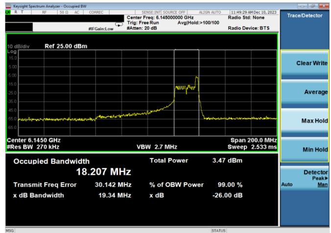
Plot 7-11. 26dB & 99% Bandwidth Plot Antenna WF7a (80MHz 802.11ax RU26 (UNII Band 5) – Ch. 39)
