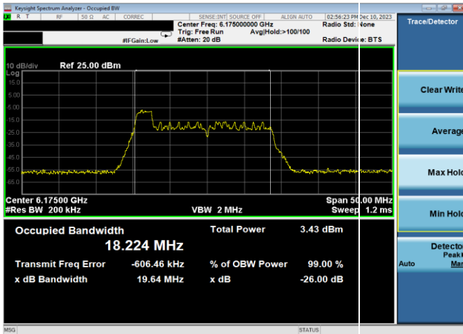
Plot 7-65. 26dB & 99% Bandwidth Plot Antenna WF2a (20MHz 802.11ax RU26 (UNII Band 5) – Ch. 45)
