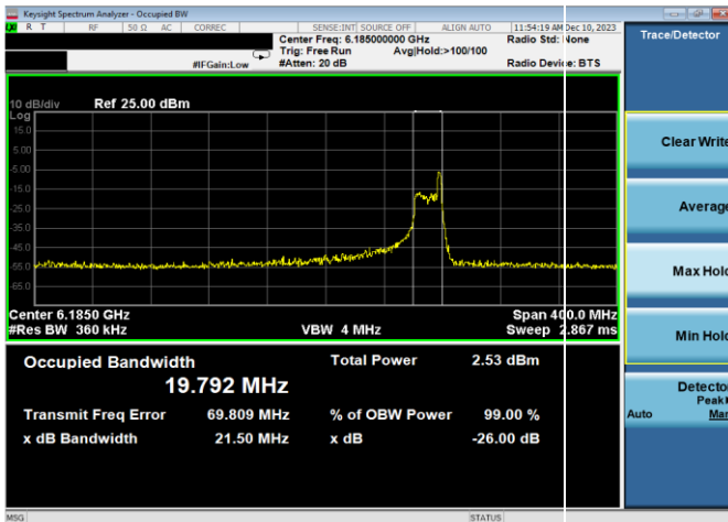
Plot 7-15. 26dB & 99% Bandwidth Plot Antenna WF7a (160MHz 802.11ax RU26 (UNII Band 5) - Ch. 47)
