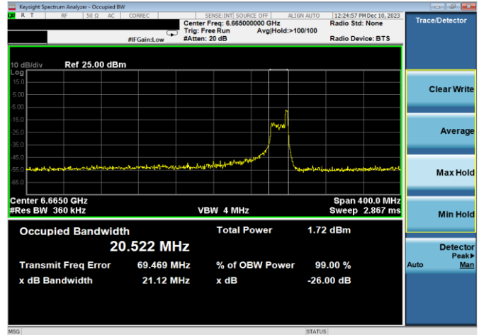
Plot 7-47. 26dB & 99% Bandwidth Plot Antenna WF7a (160MHz 802.11ax RU26 (UNII Band 7) - Ch. 143)
