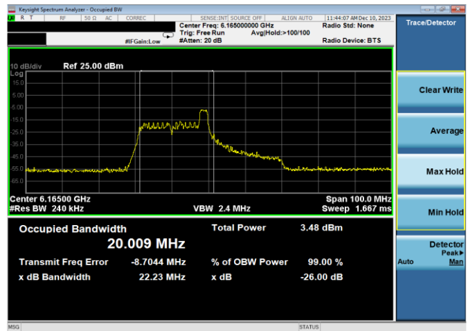
Plot 7-6. 26dB & 99% Bandwidth Plot Antenna WF7a (40MHz 802.11ax RU26 (UNII Band 5) - Ch. 43)
