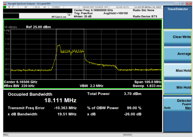
Plot 7-5. 26dB & 99% Bandwidth Plot Antenna WF7a (40MHz 802.11ax RU26 (UNII Band 5) - Ch. 43)
