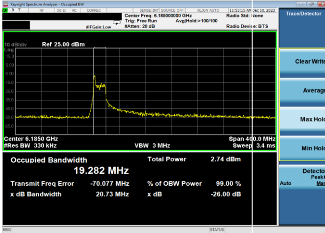
Plot 7-13. 26dB & 99% Bandwidth Plot Antenna WF7a (160MHz 802.11ax RU26 (UNII Band 5) - Ch. 47)
