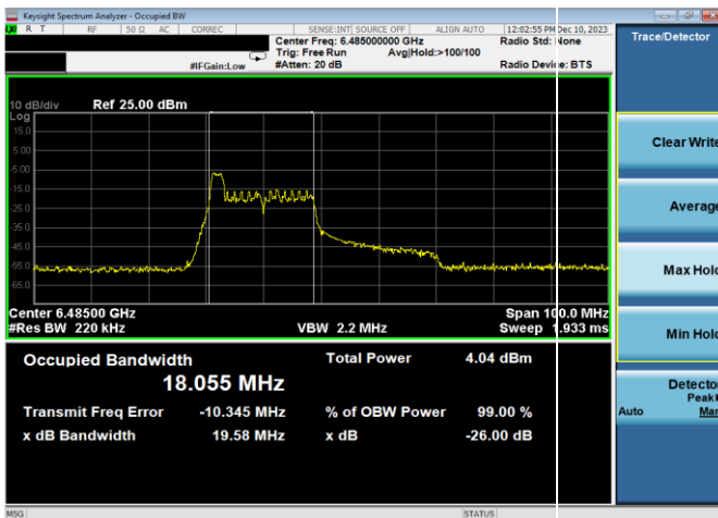
Plot 7-21. 26dB & 99% Bandwidth Plot Antenna WF7a (40MHz 802.11ax RU26 (UNII Band 6) - Ch. 107)
