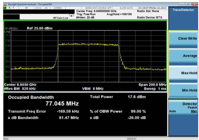
Plot 7-60. 26dB & 99% Bandwidth Plot Antenna WF7a (80MHz 802.11ax RU996 (UNII Band 8) - Ch. 199)
