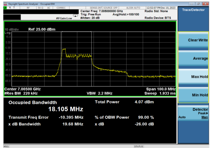
Plot 7-53. 26dB & 99% Bandwidth Plot Antenna WF7a (40MHz 802.11ax RU26 (UNII Band 8) - Ch. 211)
