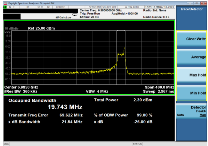
Plot 7-63. 26dB & 99% Bandwidth Plot Antenna WF7a (160MHz 802.11ax RU26 (UNII Band 8) – Ch. 207)
