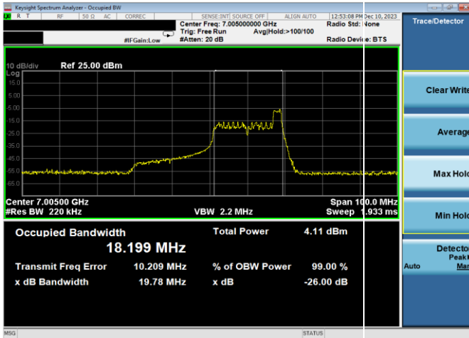
Plot 7-55. 26dB & 99% Bandwidth Plot Antenna WF7a (40MHz 802.11ax RU26 (UNII Band 8) - Ch. 211)
