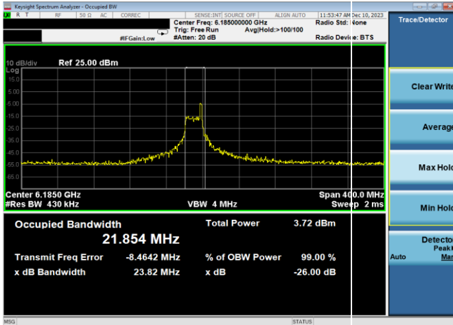
Plot 7-14. 26dB & 99% Bandwidth Plot Antenna WF7a (160MHz 802.11ax RU26 (UNII Band 5) - Ch. 47)
