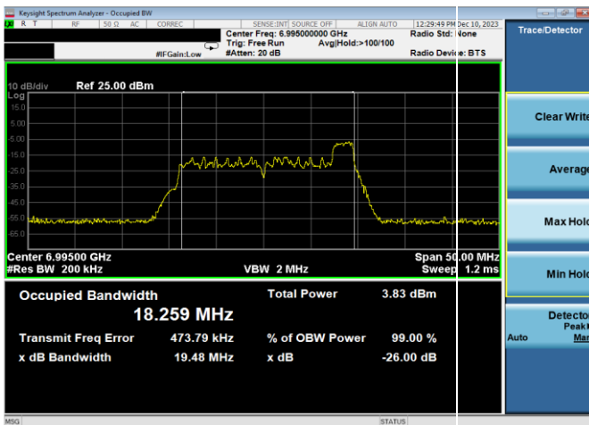
Plot 7-51. 26dB & 99% Bandwidth Plot Antenna WF7a (20MHz 802.11ax RU26 (UNII Band 8) - Ch. 209)
