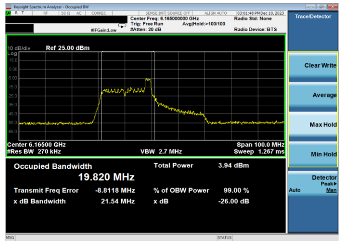
Plot 7-70. 26dB & 99% Bandwidth Plot Antenna WF2a (40MHz 802.11ax RU26 (UNII Band 5) – Ch. 43)
