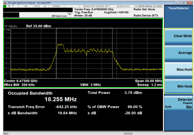
Plot 7-17. 26dB & 99% Bandwidth Plot Antenna WF7a (20MHz 802.11ax RU26 (UNII Band 6) - Ch. 105)
