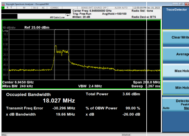
Plot 7-57. 26dB & 99% Bandwidth Plot Antenna WF7a (80MHz 802.11ax RU26 (UNII Band 8) - Ch. 199)
