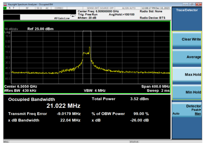
Plot 7-30. 26dB & 99% Bandwidth Plot Antenna WF7a (160MHz 802.11ax RU26 (UNII Band 6) - Ch. 111)
