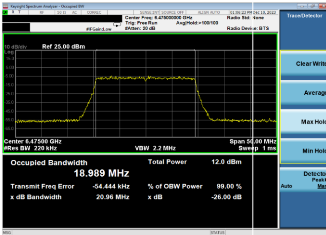
Plot 7-20. 26dB & 99% Bandwidth Plot Antenna WF7a (20MHz 802.11ax RU242 (UNII Band 6) - Ch. 105)
