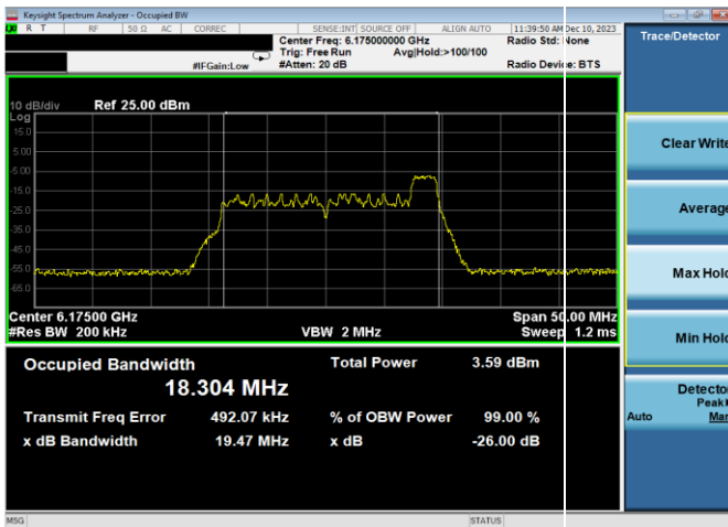
Plot 7-3. 26dB & 99% Bandwidth Plot Antenna WF7a (20MHz 802.11ax RU26 (UNII Band 5) - Ch. 45)
