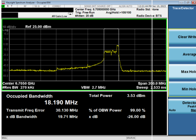
Plot 7-43. 26dB & 99% Bandwidth Plot Antenna WF7a (80MHz 802.11ax RU26 (UNII Band 7) - Ch. 151)
