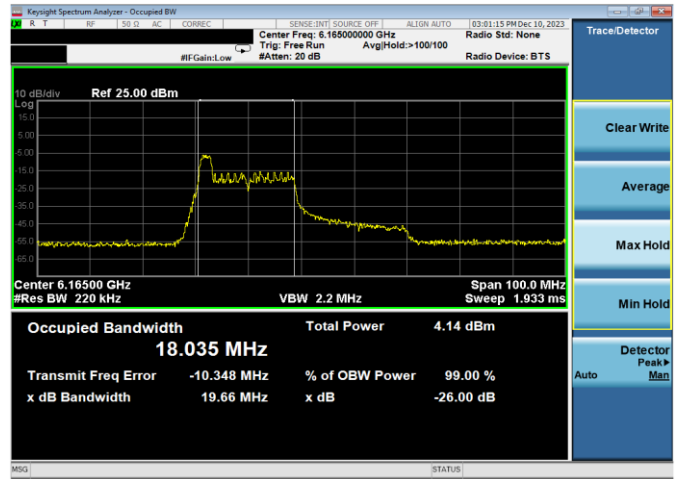
Plot 7-69. 26dB & 99% Bandwidth Plot Antenna WF2a (40MHz 802.11ax RU26 (UNII Band 5) – Ch. 43)
