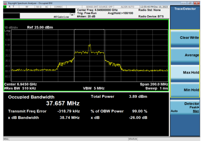
Plot 7-58. 26dB & 99% Bandwidth Plot Antenna WF7a (80MHz 802.11ax RU26 (UNII Band 8) - Ch. 199)
