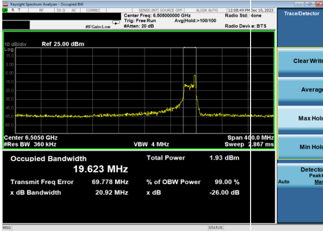
Plot 7-31. 26dB & 99% Bandwidth Plot Antenna WF7a (160MHz 802.11ax RU26 (UNII Band 6) – Ch. 111)
