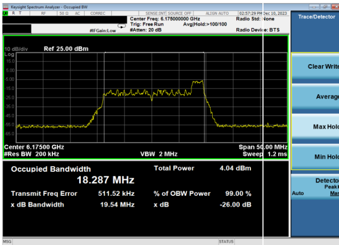
Plot 7-67. 26dB & 99% Bandwidth Plot Antenna WF2a (20MHz 802.11ax RU26 (UNII Band 5) – Ch. 45)
