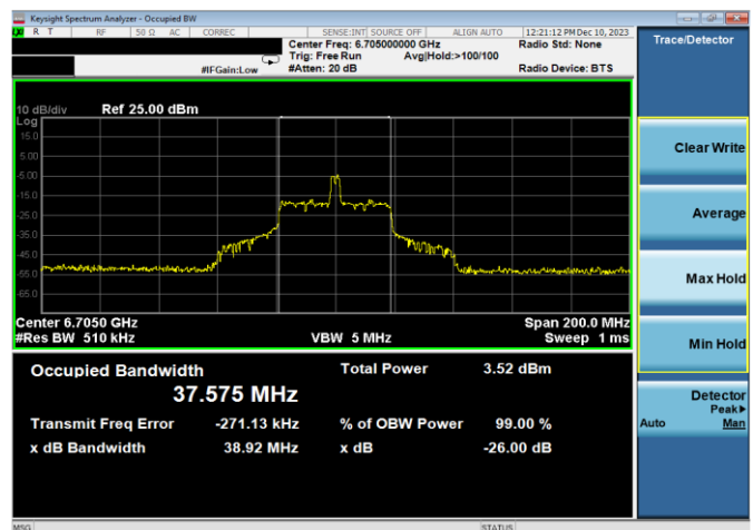
Plot 7-42. 26dB & 99% Bandwidth Plot Antenna WF7a (80MHz 802.11ax RU26 (UNII Band 7) – Ch. 151)
