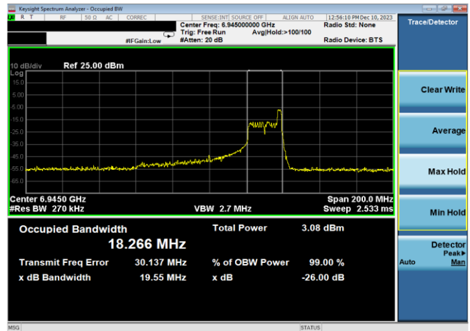
Plot 7-59. 26dB & 99% Bandwidth Plot Antenna WF7a (80MHz 802.11ax RU26 (UNII Band 8) - Ch. 199)
