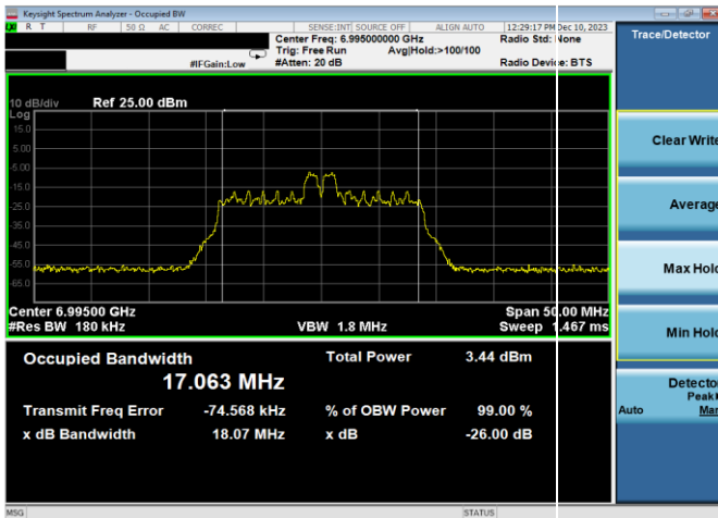
Plot 7-50. 26dB & 99% Bandwidth Plot Antenna WF7a (20MHz 802.11ax RU26 (UNII Band 8) - Ch. 209)
