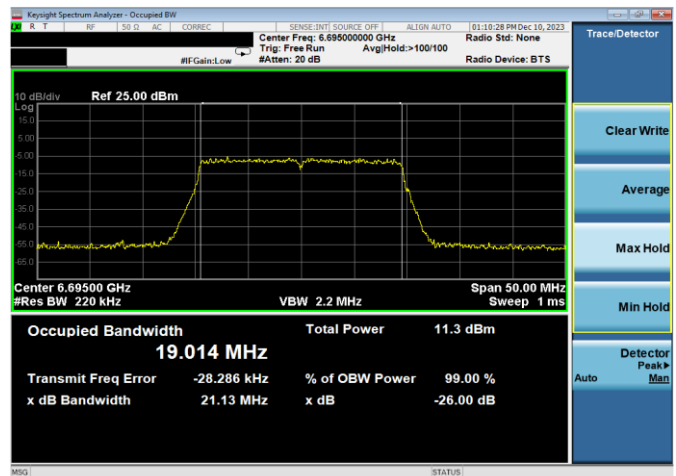
Plot 7-36. 26dB & 99% Bandwidth Plot Antenna WF7a (20MHz 802.11ax RU242 (UNII Band 7) – Ch. 149)
