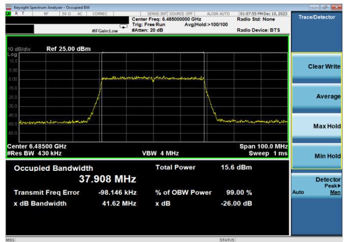
Plot 7-24. 26dB & 99% Bandwidth Plot Antenna WF7a (40MHz 802.11ax RU484 (UNII Band 6) - Ch. 107)
