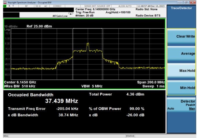
Plot 7-10. 26dB & 99% Bandwidth Plot Antenna WF7a (80MHz 802.11ax RU26 (UNII Band 5) – Ch. 39)
