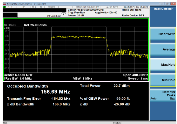
Plot 7-48. 26dB & 99% Bandwidth Plot Antenna WF7a (160MHz 802.11ax RU996x2 (UNII Band 7) - Ch. 143)
