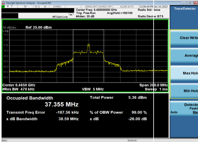
Plot 7-26. 26dB & 99% Bandwidth Plot Antenna WF7a (80MHz 802.11ax RU26 (UNII Band 6) - Ch. 103)
