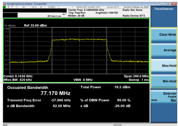
Plot 7-12. 26dB & 99% Bandwidth Plot Antenna WF7a (80MHz 802.11ax RU996 (UNII Band 5) – Ch. 39)
