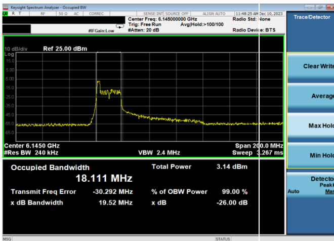
Plot 7-9. 26dB & 99% Bandwidth Plot Antenna WF7a (80MHz 802.11ax RU26 (UNII Band 5) – Ch. 39)
