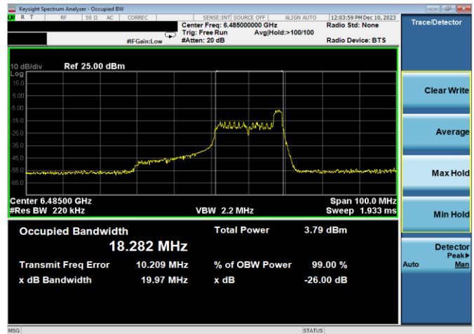
Plot 7-23. 26dB & 99% Bandwidth Plot Antenna WF7a (40MHz 802.11ax RU26 (UNII Band 6) - Ch. 107)
