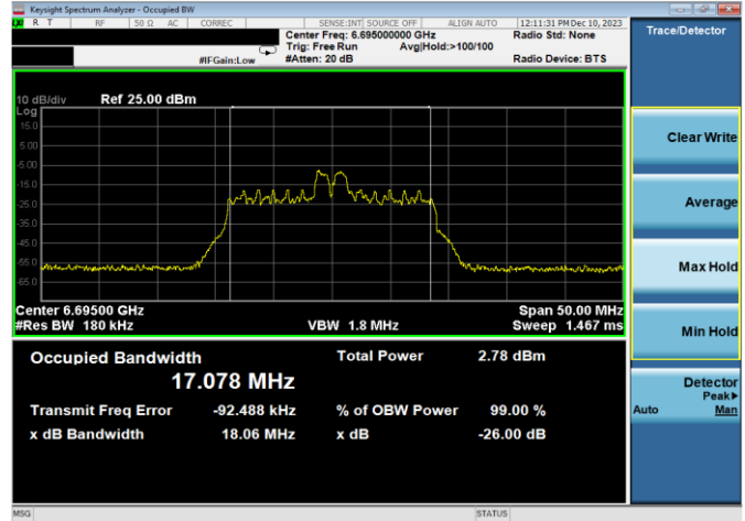
Plot 7-34. 26dB & 99% Bandwidth Plot Antenna WF7a (20MHz 802.11ax RU26 (UNII Band 7) – Ch. 149)
