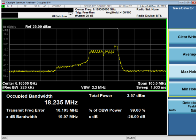
Plot 7-7. 26dB & 99% Bandwidth Plot Antenna WF7a (40MHz 802.11ax RU26 (UNII Band 5) – Ch. 43)
