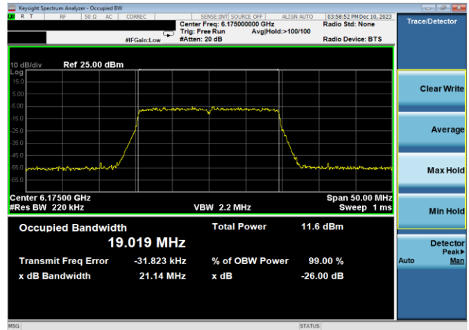
Plot 7-68. 26dB & 99% Bandwidth Plot Antenna WF2a (20MHz 802.11ax RU242 (UNII Band 5) – Ch. 45)
