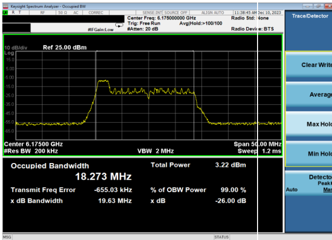
Plot 7-1. 26dB & 99% Bandwidth Plot Antenna WF7a (20MHz 802.11ax RU26 (UNII Band 5) - Ch. 45)
