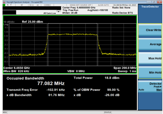
Plot 7-28. 26dB & 99% Bandwidth Plot Antenna WF7a (80MHz 802.11ax RU996 (UNII Band 6) - Ch. 103)
