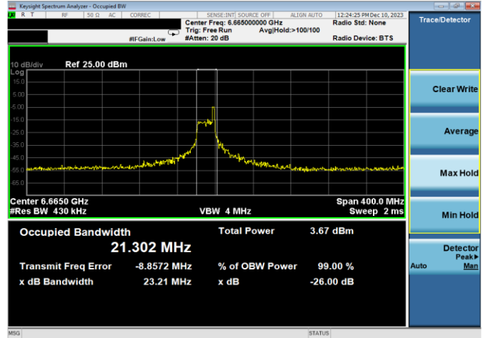
Plot 7-46. 26dB & 99% Bandwidth Plot Antenna WF7a (160MHz 802.11ax RU26 (UNII Band 7) - Ch. 143)
