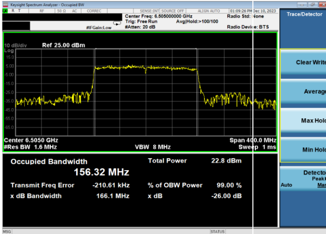
Plot 7-32. 26dB & 99% Bandwidth Plot Antenna WF7a (160MHz 802.11ax RU996x2 (UNII Band 6) – Ch. 111)
