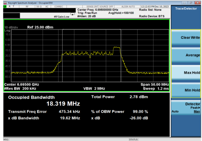
Plot 7-35. 26dB & 99% Bandwidth Plot Antenna WF7a (20MHz 802.11ax RU26 (UNII Band 7) – Ch. 149)
