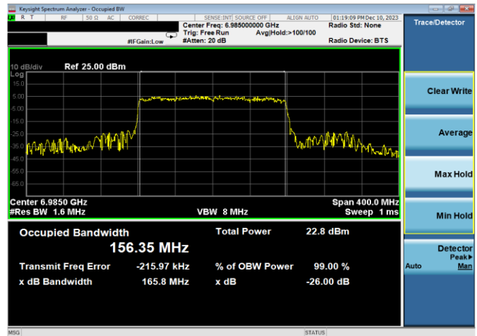
Plot 7-64. 26dB & 99% Bandwidth Plot Antenna WF7a (160MHz 802.11ax RU996x2 (UNII Band 8) – Ch. 207)
