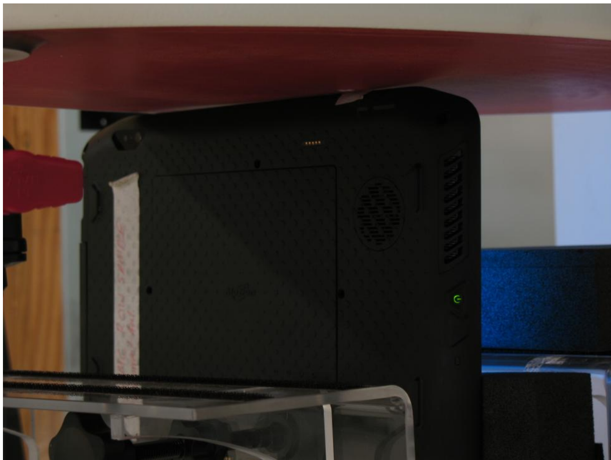
Figure 3: Device Positioning for SAR Scans – Top Edge with no Spacing
