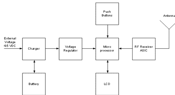
LPU - 810 Block Diagram
