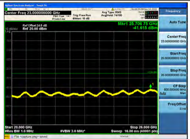
Band7-20G-26G / 15MHz / Mid CH / 16QAM
