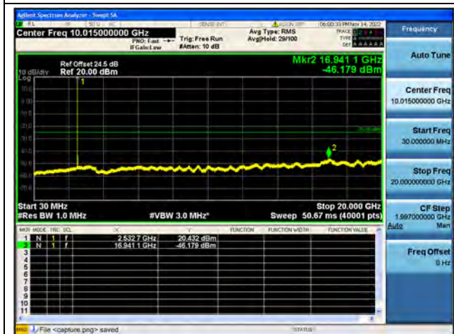
Band7-30M-20G / 5MHz / Mid CH / 16QAM
