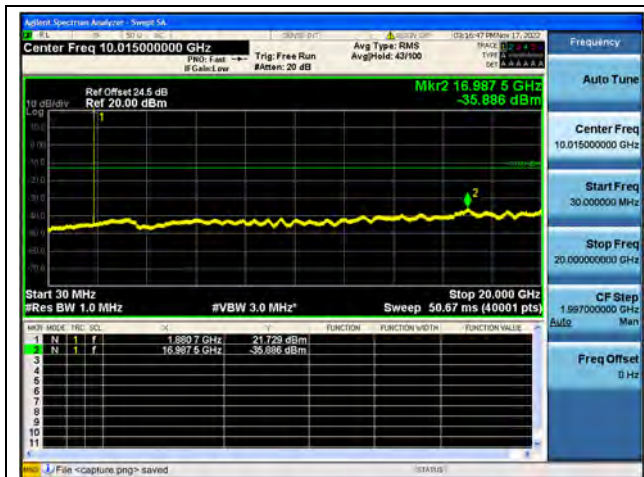
Band25 / 3MHz / Mid CH / QPSK
