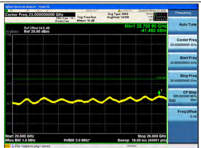
Band7-20G-26G / 15MHz / Mid CH / 64QAM
