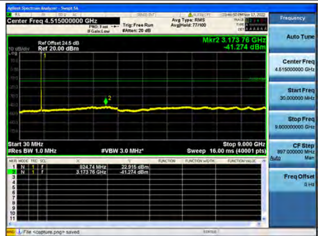
Band26Part22 / 10MHz / Low CH / QPSK
