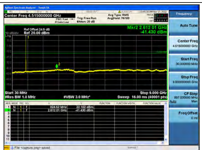
Band26Part22 / 5MHz / Low CH / 16QAM
