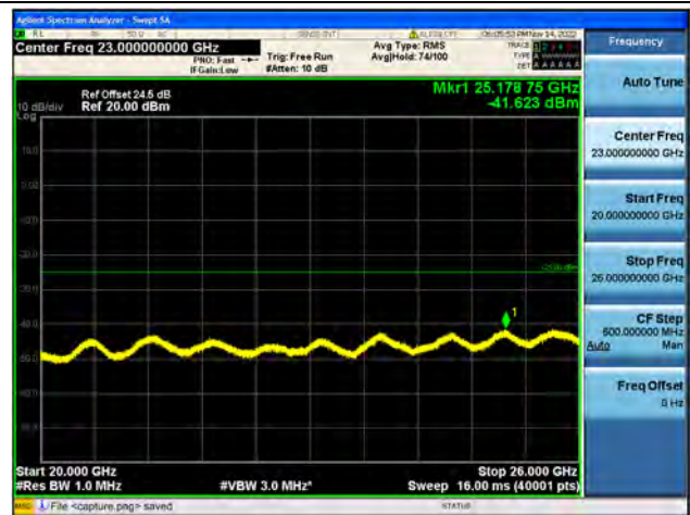
Band7-20G-26G / 10MHz / High CH / 16QAM
