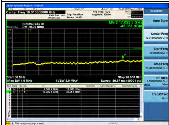
Band7-30M-20G / 5MHz / Mid CH / 64QAM
