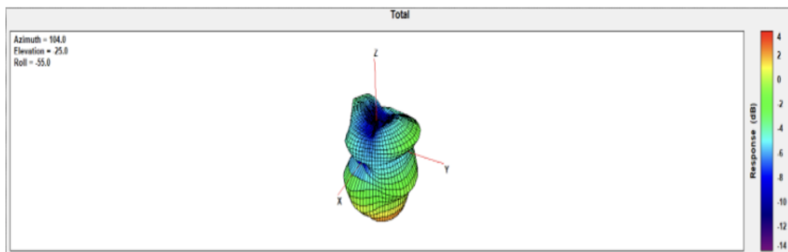
ANT3 Frequency 2480MHz
