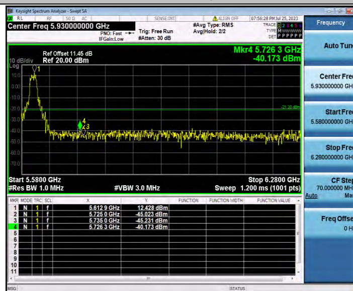
11AC80SISO_Ant1_High_5610_Peak
