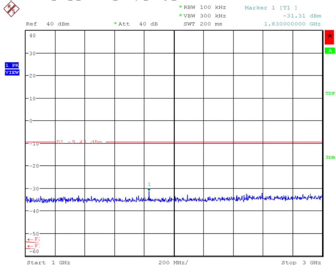
Figure 48: D01_037_2_CSE20dBc_Sweep2_ChHigh_FHSS
