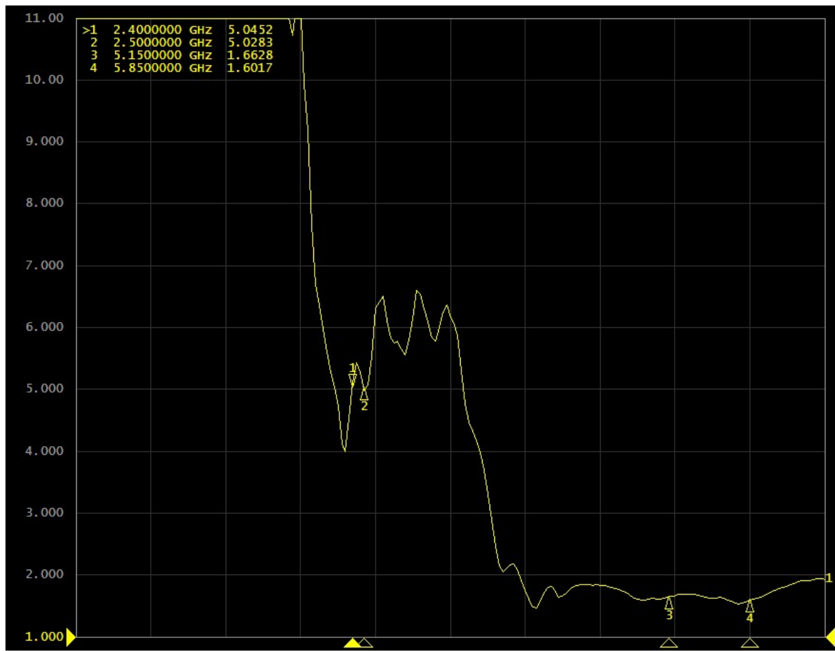
5G1-SWR
