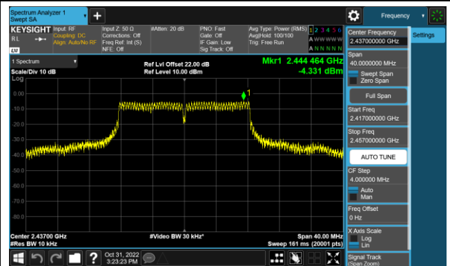
Channel 06 (2437MHz)
