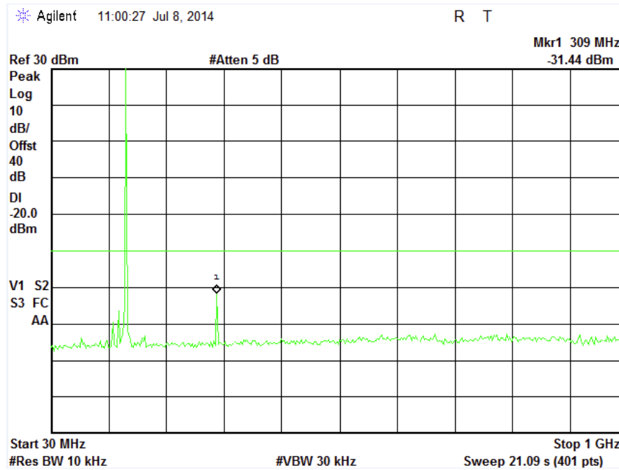
Plot D5 : 155.025 MHz @ 12.5KHz Channel Separations – Middle Power Level
