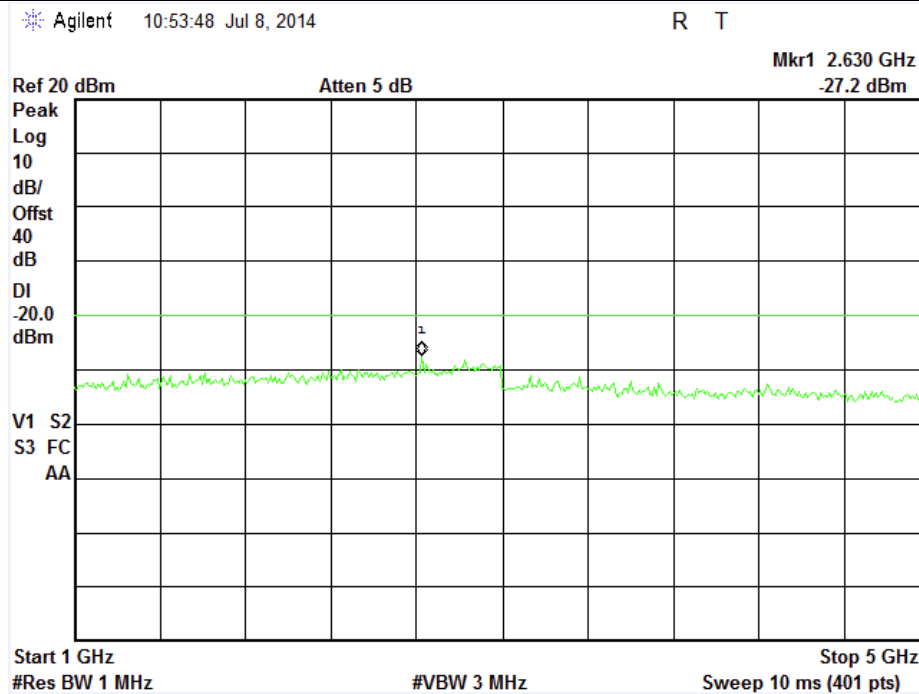
Plot D6 : 155.025 MHz @ 12.5KHz Channel Separations – Middle Power Level
