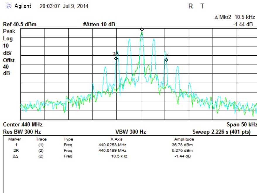
Plot C2 : 440.025MHz (Maximum) @ 12.5 KHz Channel Separation
