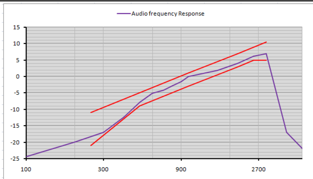
Plot B4: 440.025MHz @ 12.5 KHz Channel Separation
