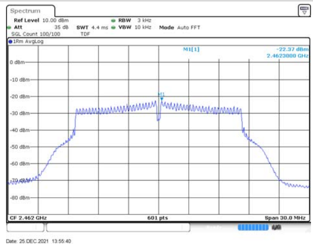
802.11g HIGH CHANNEL
