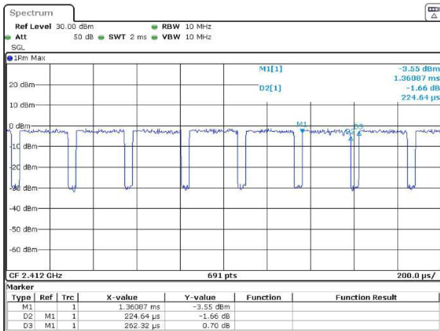
Test Graph_ IEEE802.11 n (HT20) Duty Cycle:
