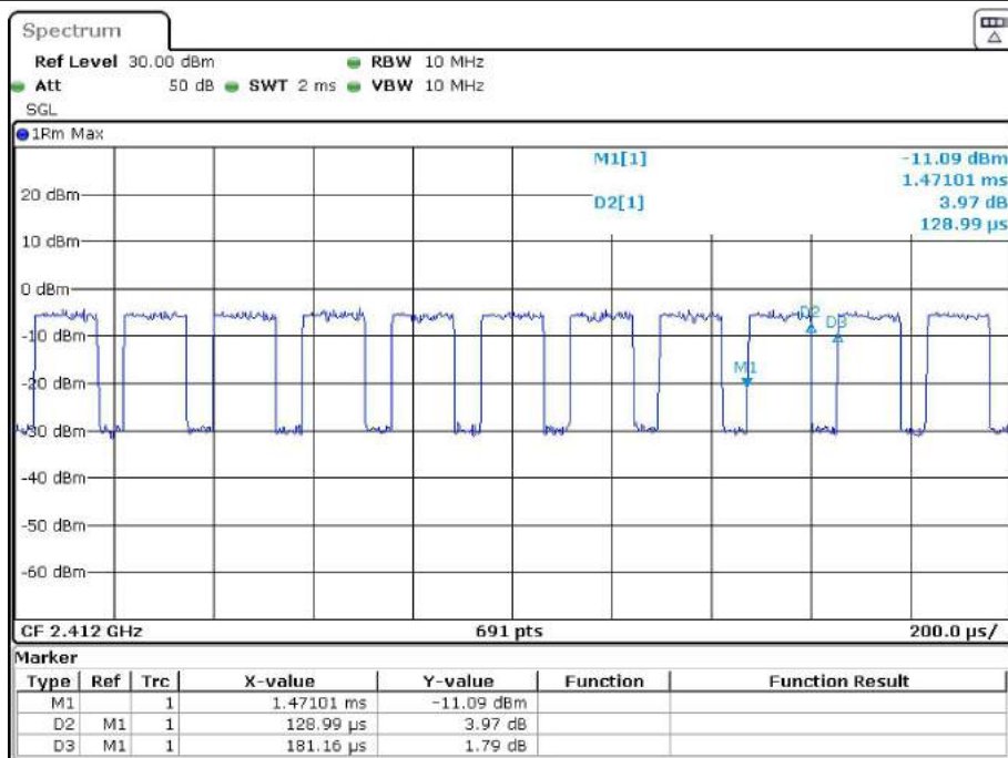
Test Graph_IEEE802.11 n (HT40) Duty Cycle:
