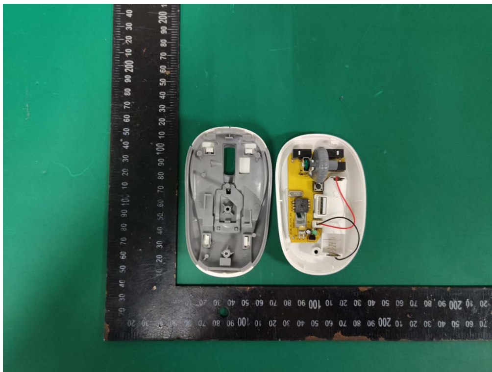
Internal photos M/N: NX-7028
