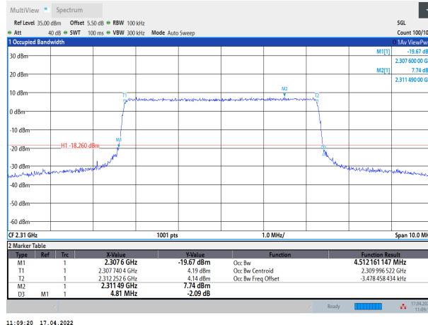
Band30-5MHz-QPSK-27710-25RB#0
